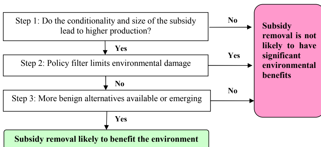
Figure 2: The Checklist
