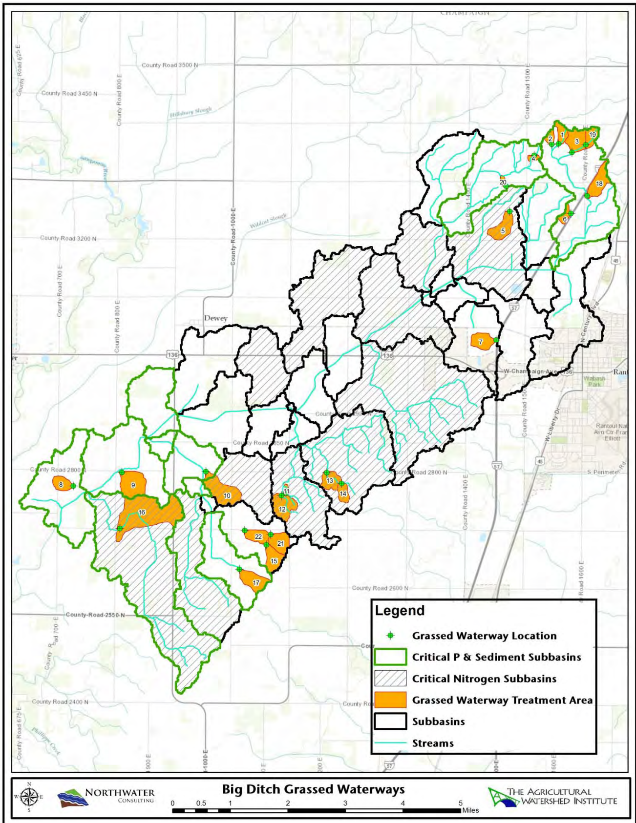
Figure 7 – Potential Site-Specific Grassed Waterway
