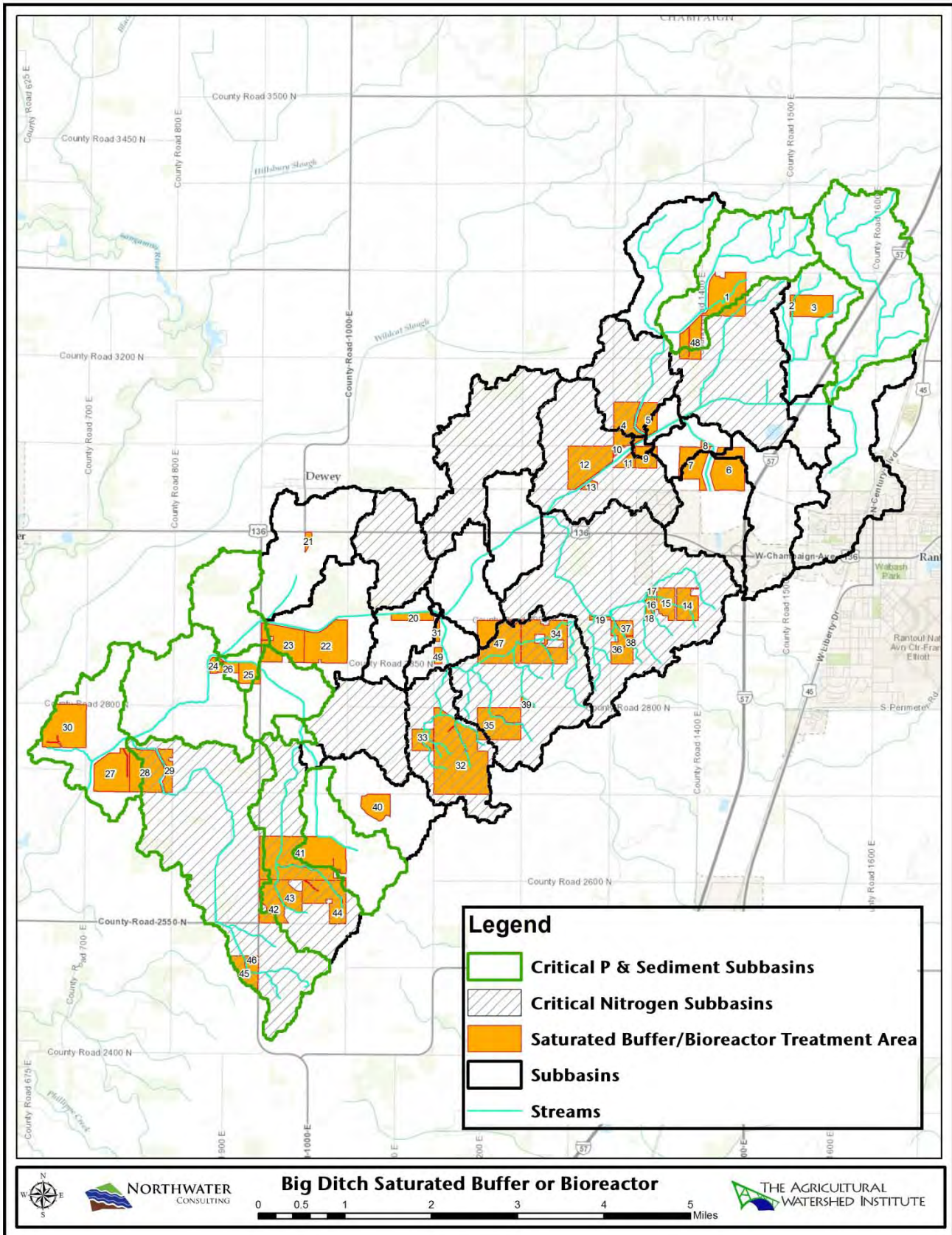
Figure 17 – Potential Basin-Wide Saturated Buffer/Bioreactor
