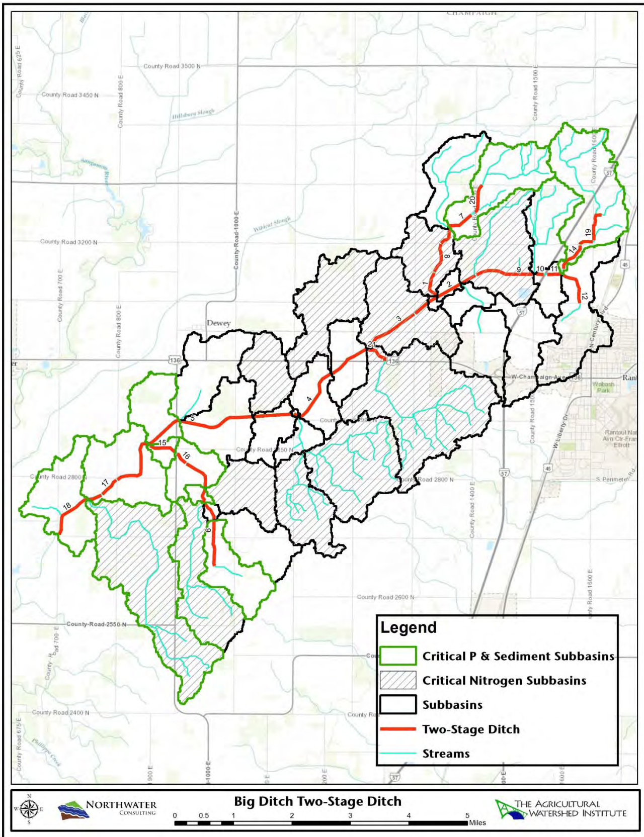
Figure 10 – Potential Site Specific Two-Stage Ditch
