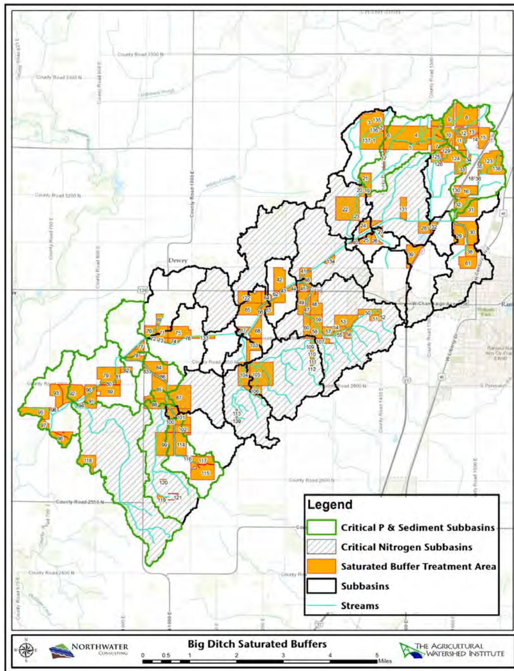
Figure 13 – Potential Basin-Wide Saturated Buffers
