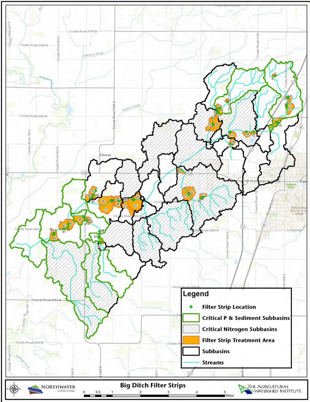
Figure 11 – Potential Site-Specific Filter Strips
