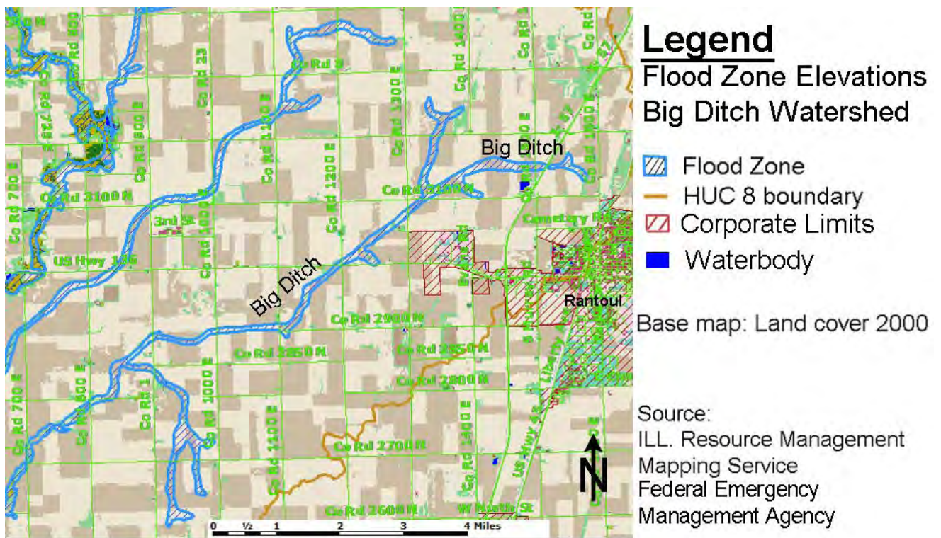
Fig. 6 - Floodplain Map
