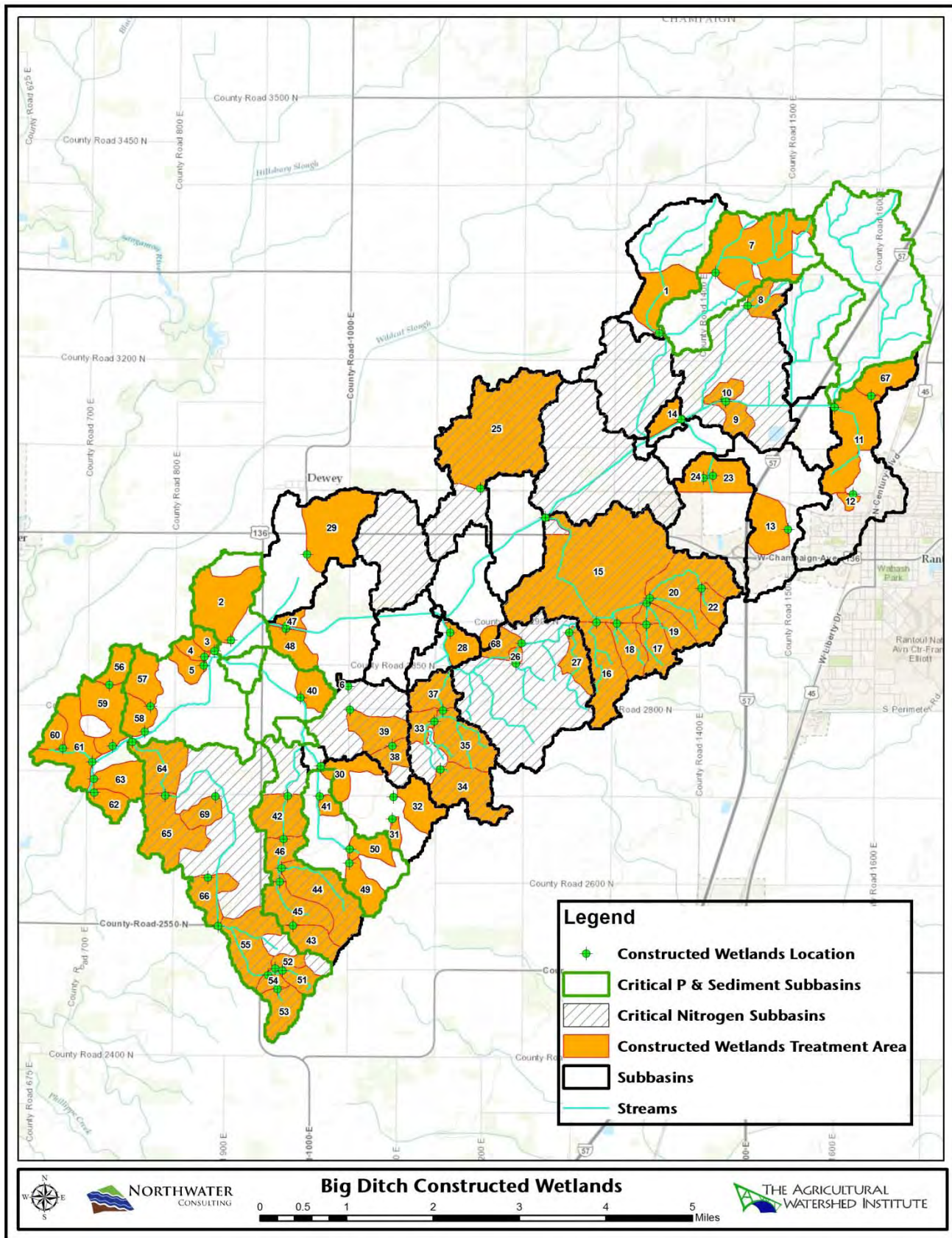
Figure 8 – Potential Site-Specific Constructed Wetland
