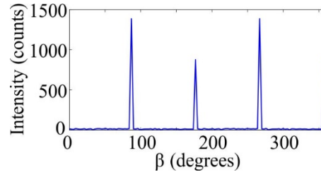
Fig. 3. XRD data of the Yb(1.4%):YAG film on \langle 100 \rangle YAG displayed as an intensity profile at \alpha = 0^\circ of a (400) pole figure with \langle 100 \rangle orientation.
