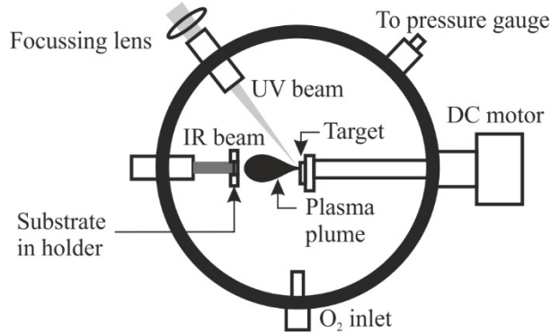
Fig. 1. Schematic of pulsed laser deposition set-up.
