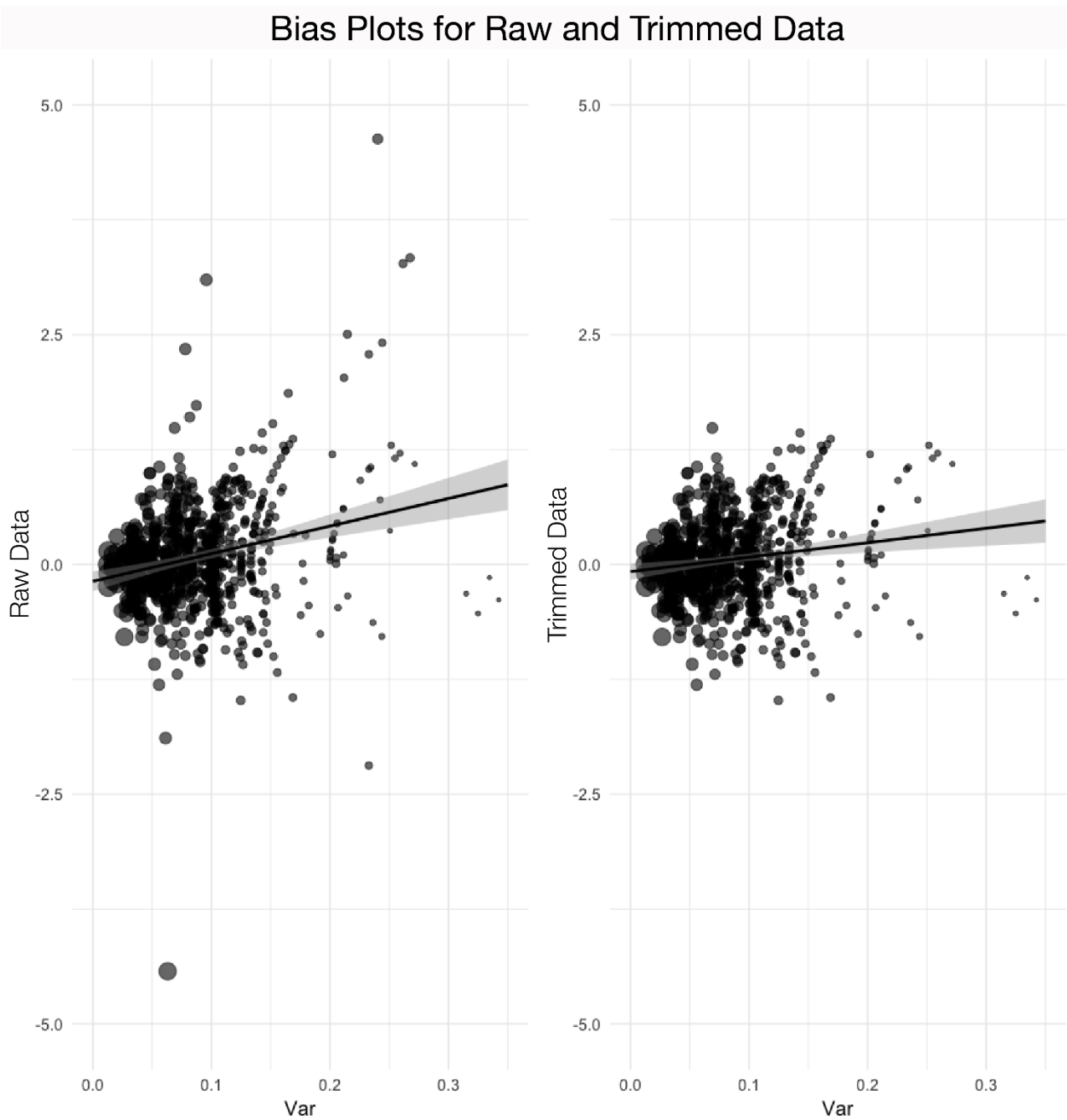
7 8 Figure 3. Plots visualizing the PEESSE-corrected effect size. The line depicts the regression
