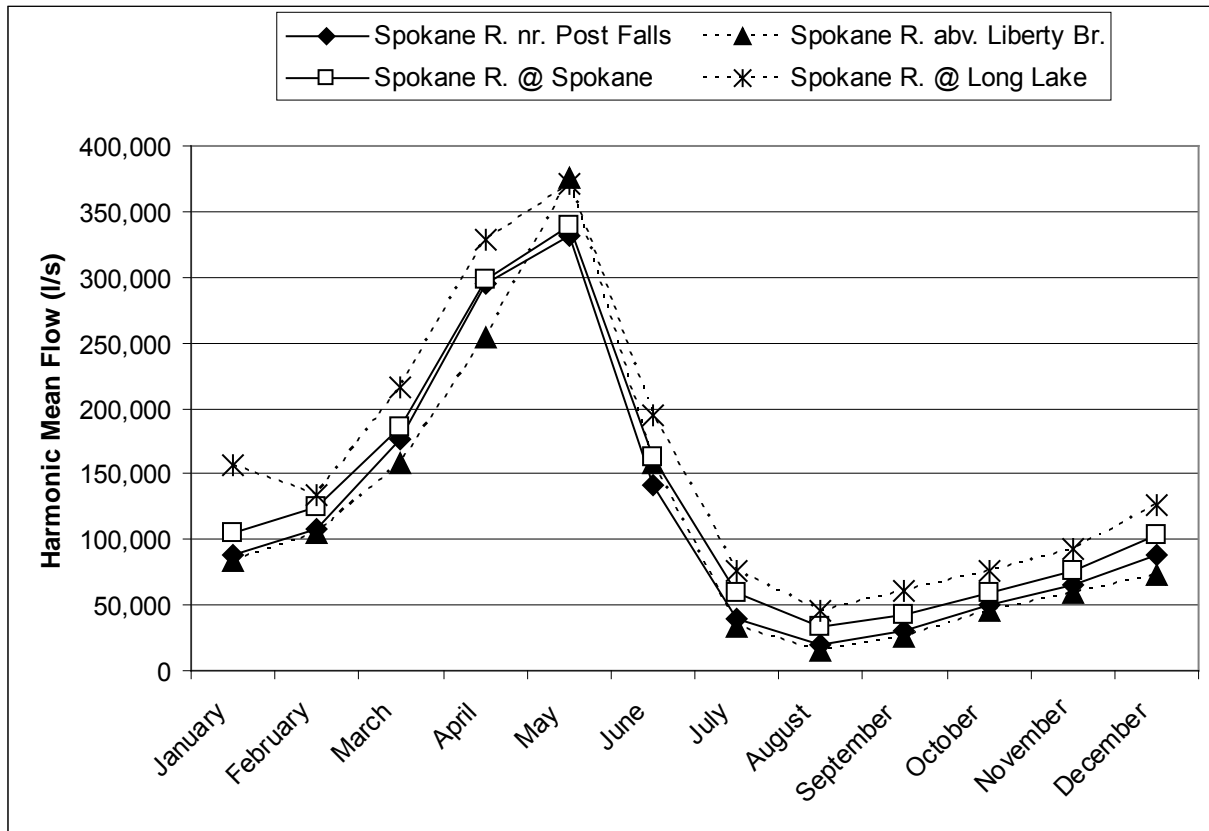
Figure 3. Spokane River Monthly Harmonic Mean Flows for Water Years 1969-2002.
