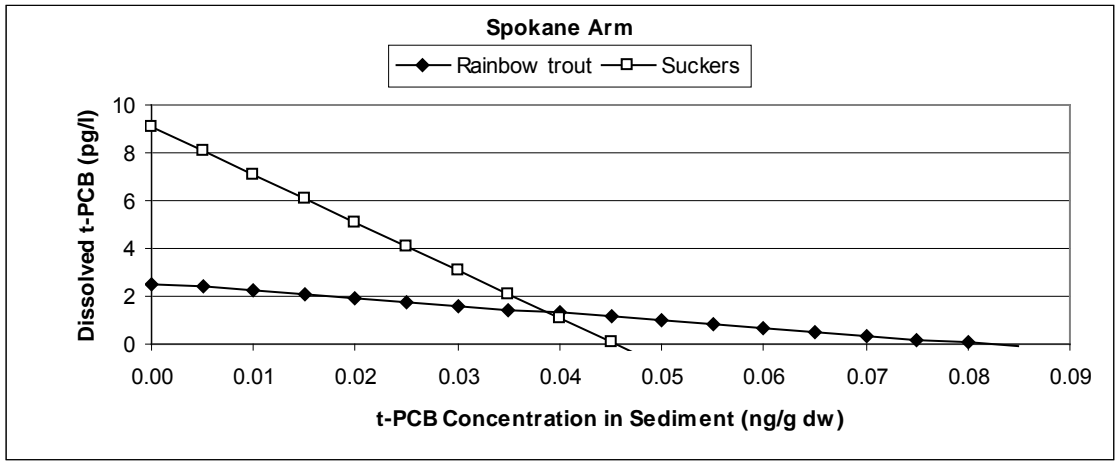
Figure 21. Dissolved Water and Sediment Total PCB Concentrations Predicted to Yield 0.1 ng/g in Rainbow Trout and Sucker Fillet (Little Falls and Spokane Arm).
