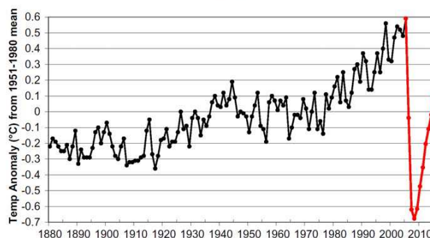
Fig. 9. Global average surface air temperature change from the 5 Tg standard case (red) in the context of the climate change of the past 125 years. Observations are from the GISS analysis (Hansen et al., 2001, updated at http://data.giss.nasa.gov/gistemp/2005/ ).
