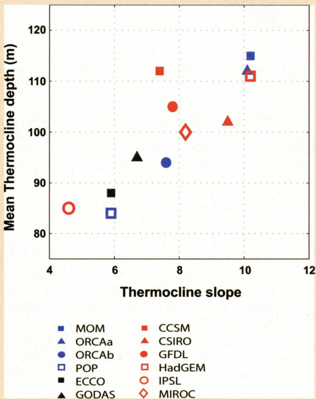
FIG. 2. Mean depth of the equatorial thermocline and mean thermocline slope along the equator as simulated in a number of ocean-only models (blue), data assimilation models (black), and coupled models (red). The thermocline slope is defined as the normalized difference between thermocline depth at 180° and 100°W, where an appropriate isopycnal surface was chosen for each individual model. The thermocline depth corresponds to maximum vertical density gradient along the equator. Note the large differences in the mean thermocline depth and, especially, thermocline slope in the models. After Brown and Fedorov (2008).
