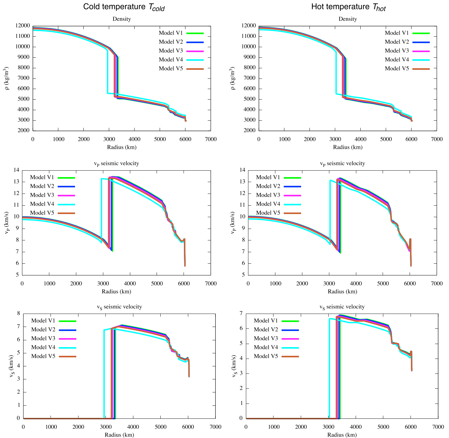
Figure 2. Density \rho and seismic velocities v_p and v_s corresponding to composition models of Table 1. (left column) Geophysical data associated with the cold temperature profile of Steinberger et al. [2010] and (right column) data associated with the hot temperature profile of Armann and Tackley [2012].
