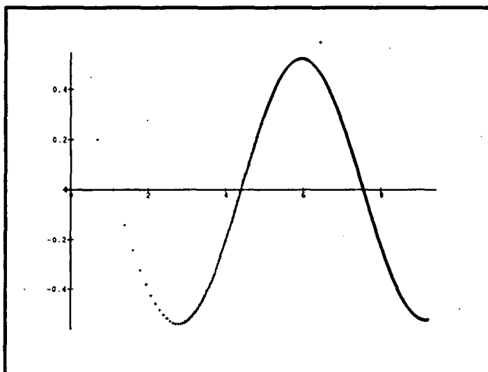
FIGURE 1. A plot of T_n versus \log n for n \leq 10,000 displays oscillations that arise from the two complex poles s = \pm i of the function \varphi(s) = (1 + s^2)^{-1} .
