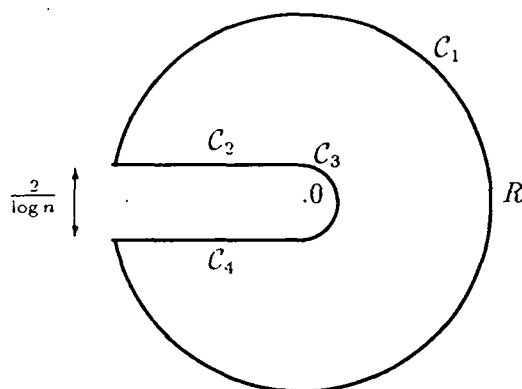
FIGURE 2. The Hankel contour relative to an algebraic or logarithmic singularity (here for s = 0 ).
