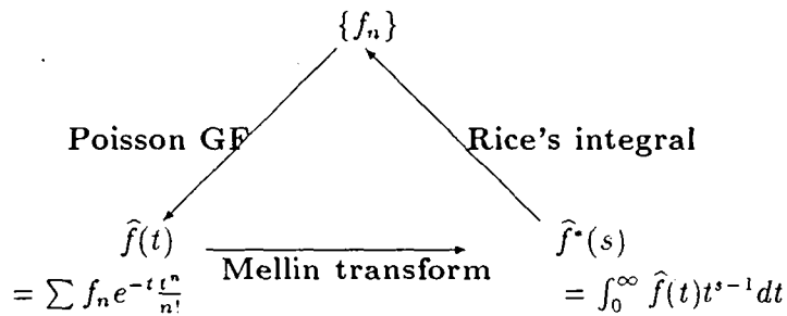
FIGURE 4. The Poisson-Mellin-Newton cycle.
