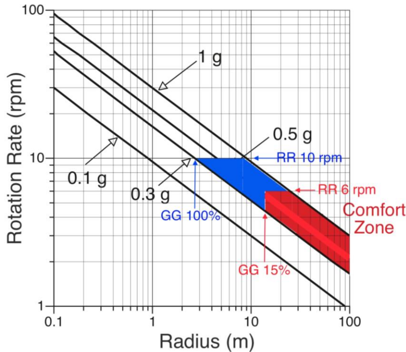
Figure 7. The rotation rate is plotted as a function of the radius of rotation for four gravity levels. Slow rotation rooms studies performed in the 1960s referred to the “comfort zone” as the red area delimited by gravity levels ranging from 0.3 g to 1 g, rotation rate < 6 rpm, and gravity gradient GG < 15% (radius > 12 m). However, recent data indicate that these limits are overly conservative: rotation rates of up to 10 rpm can be tolerated with incremental exposures, and large gravity gradient during intermittent short-radius centrifugation does not seem to be a critical factor (blue area).
