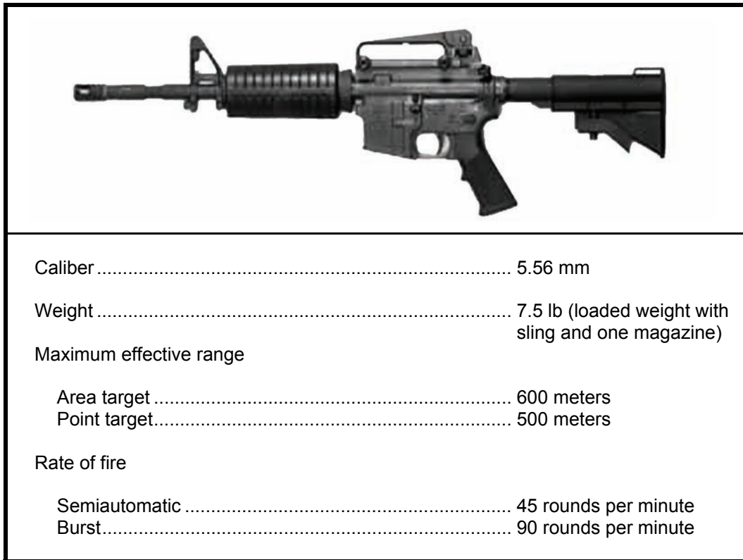
Figure 10-3. M4 carbine.
