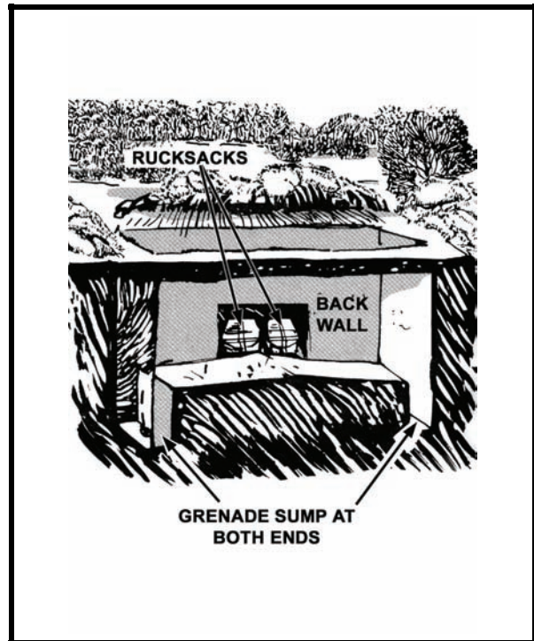
Figure 6-13. Storage compartments.
