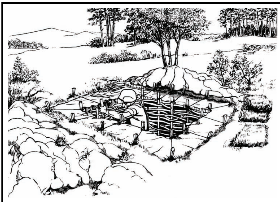
Figure 6-11. Revetment construction.
