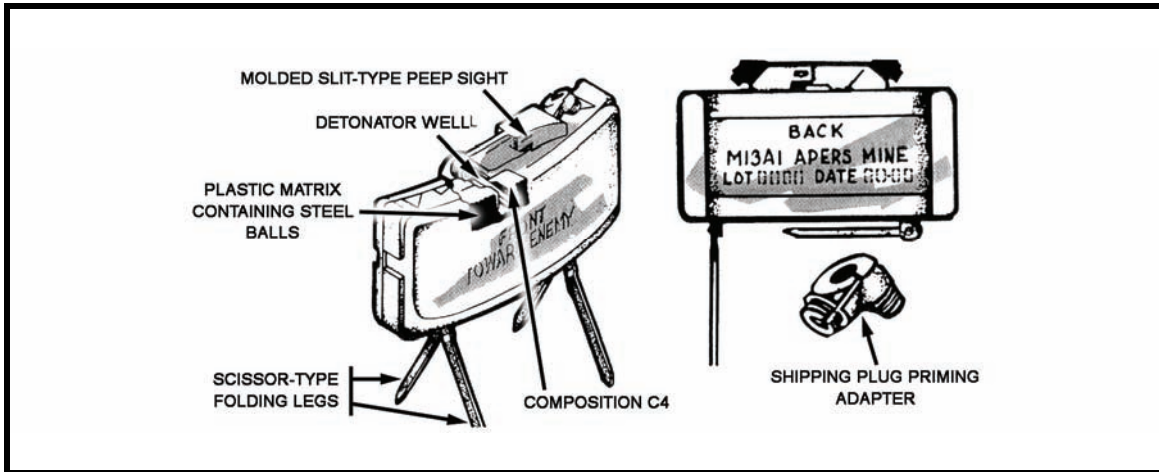
Figure 14-1. M18A1 antipersonnel mine.
