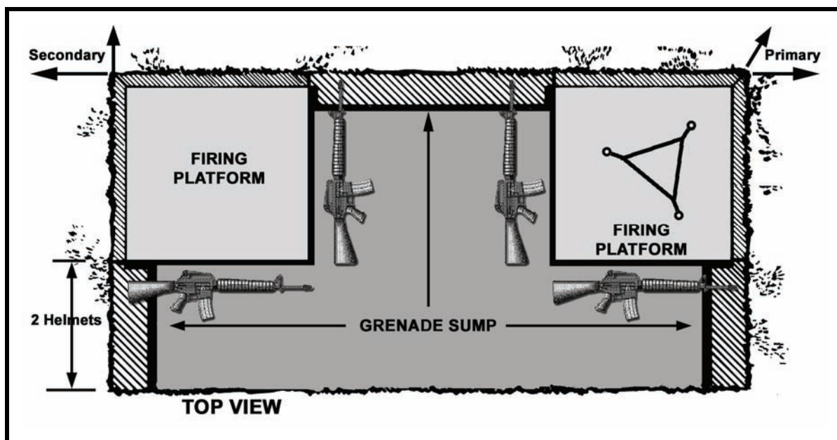
Figure 6-18. Position with firing platforms.
