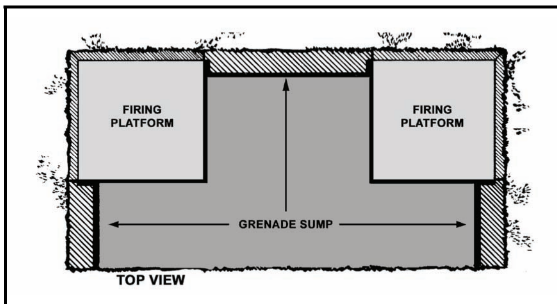
Figure 6-19. Grenade sump locations.
