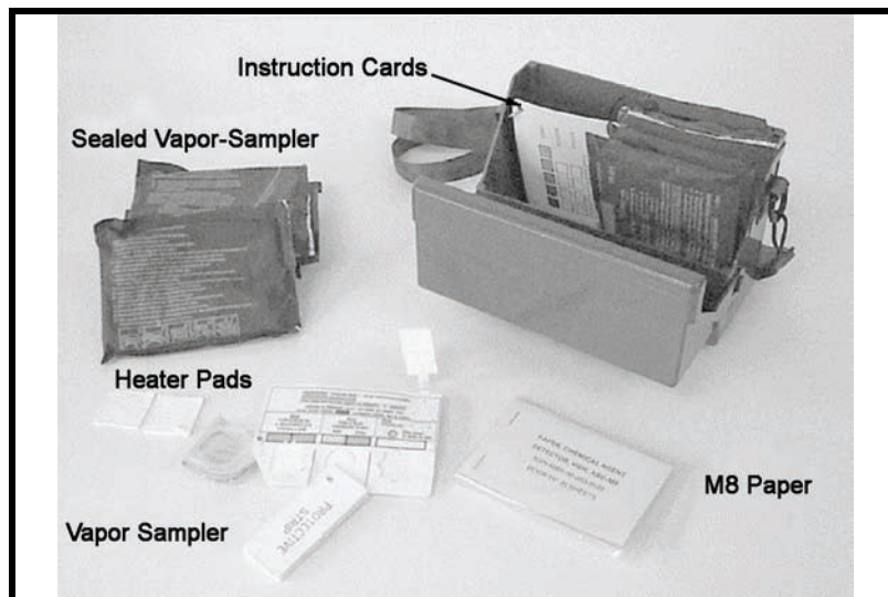
Figure 13-7. M256 chemical agent detector kit.
