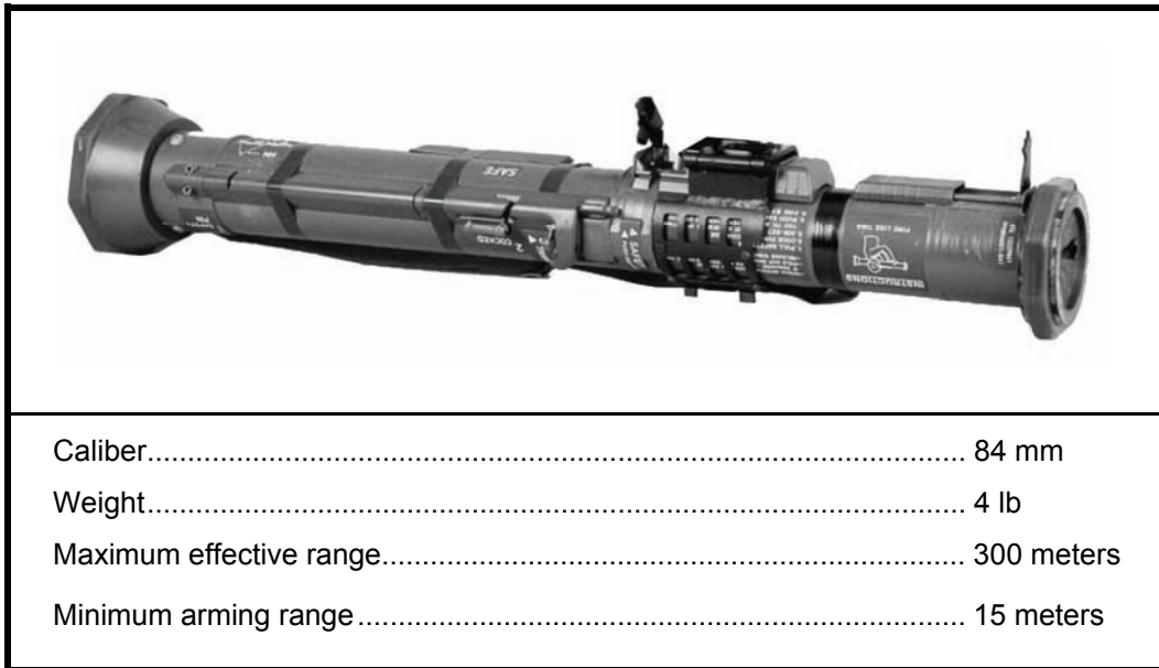
Figure 10-10. M136 AT4.
