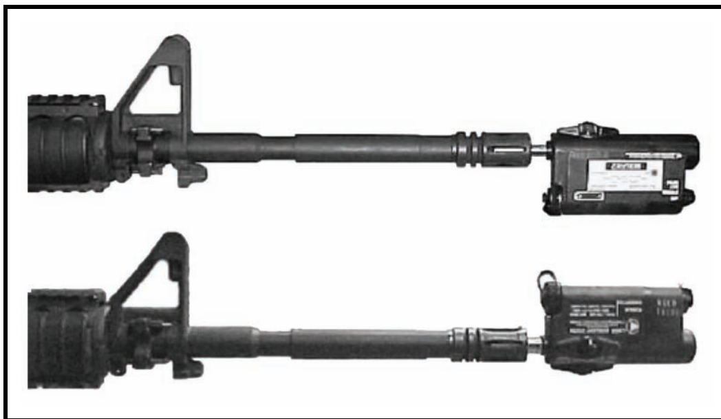
Figure 10-20. Borelight in the start point position.
