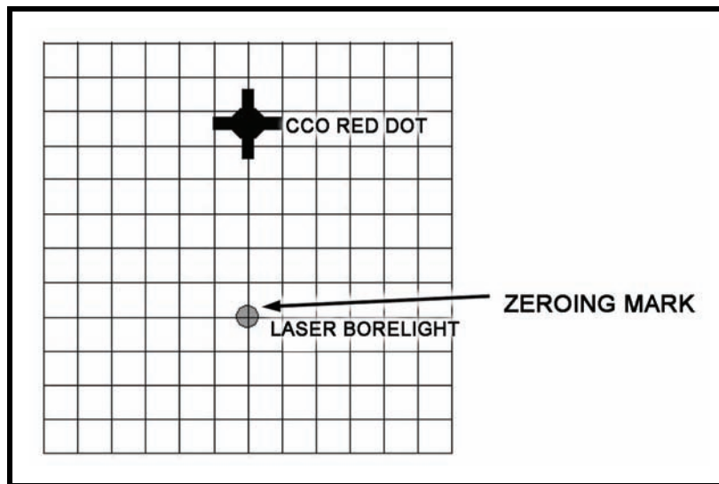
Figure 10-19. Example zeroing mark.
