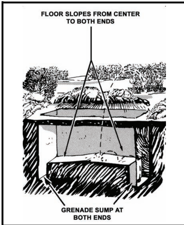
Figure 6-12. Grenade sumps.
