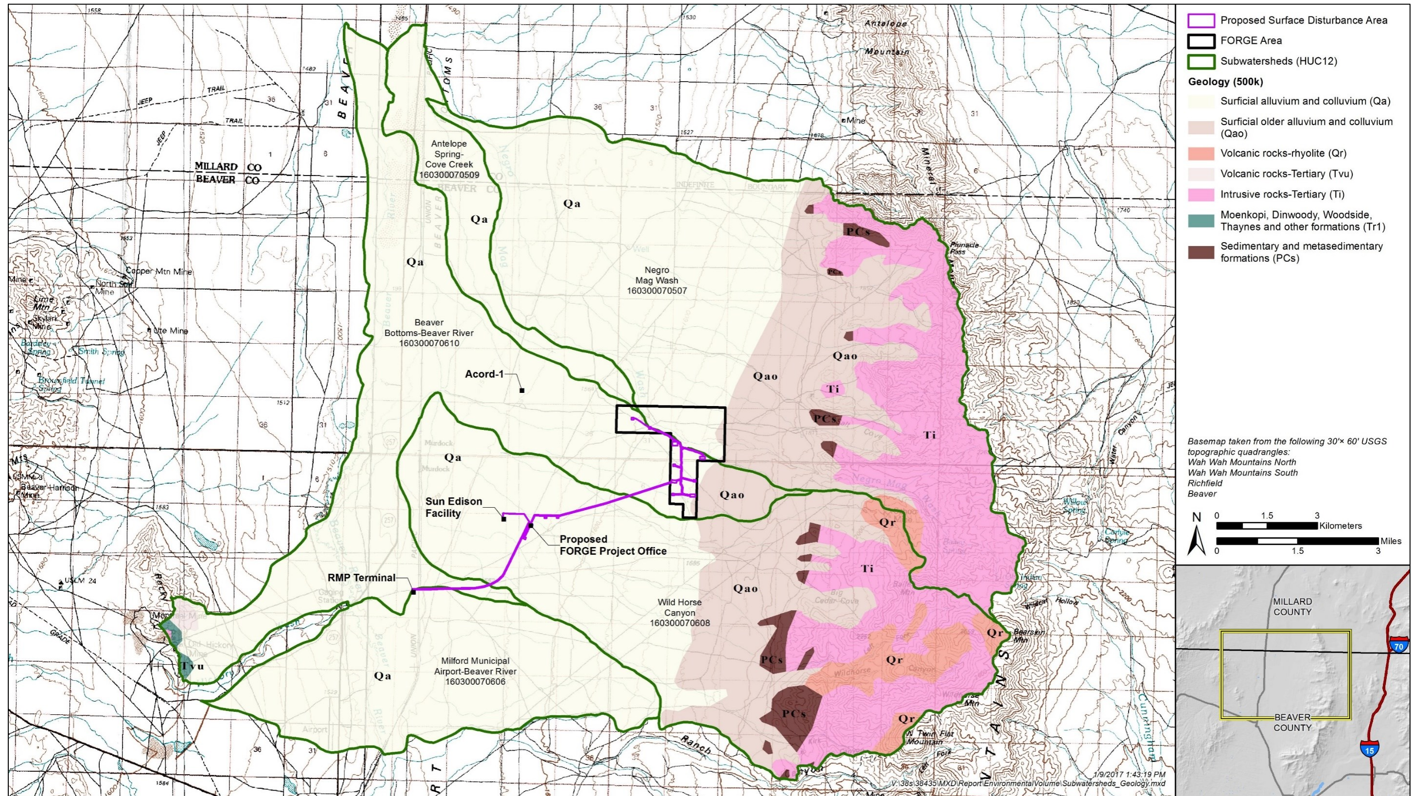
Figure 3-5. Surface geology in the project area, FORGE area, and geologic and soils analysis area.
