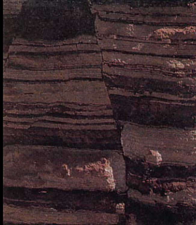
Faulting in tuff deposits
