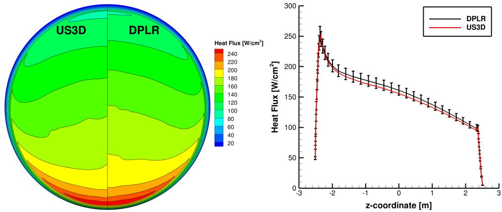
Figure 3. Comparison of surface heat flux ( W/cm^2 ).
