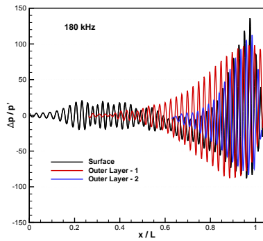
(e) Centerline
