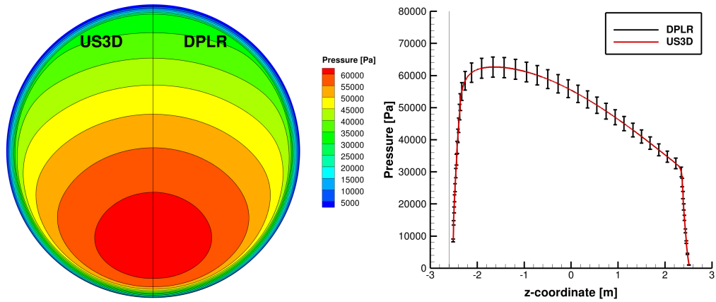
Figure 2. Comparison of surface pressure (Pa).
