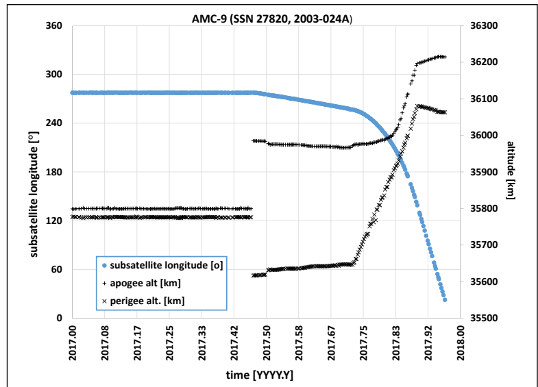
Figure 1. The 2017 orbital evolution of the AMC-9 spacecraft. Depicted are the subsattellite longitude, demonstrating a westward drift post-event, and the apogee/perigee altitude history. The altitude profile clearly indicates the abrupt nature of the 17 June 2017 event, recovery activities by the owner/operator, and the final boost to the so-called graveyard orbit above the GEO belt. Inclination control appears to have terminated in late June 2017.
