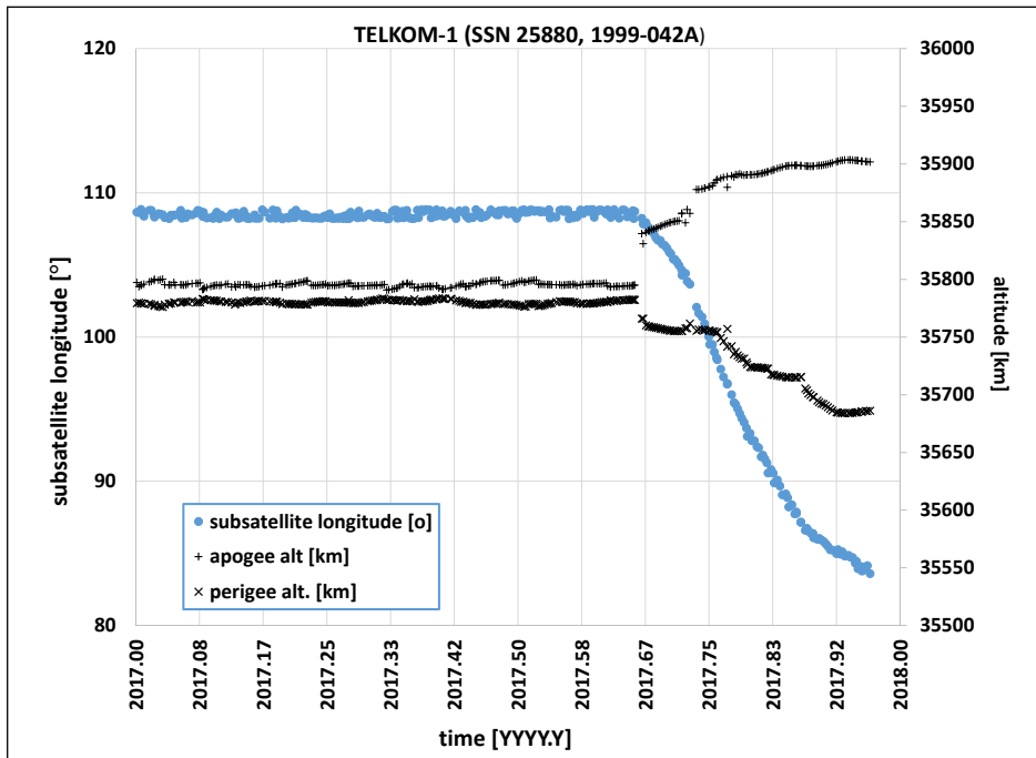
Figure 2. The 2017 orbital evolution of the TELKOM-1 spacecraft. Depicted are the subsattelite longitudes, demonstrating a westward drift post-event, and the apogee/perigee altitude history. The altitude profile clearly indicates the abrupt nature of the event and possible mitigation activities by the owner/operator. Inclination control apparently terminated in early September 2017.
