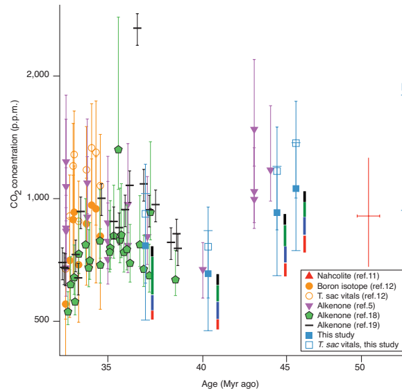
Extended Data Fig. 4 Compilation of several CO 2 records for the Eocene in comparison to this study. Data are from refs 5, 11, 12, 18 and 19. The contribution of different parameters to the uncertainty on our CO 2 reconstructions is colour-coded; sequentially from bottom to top, red is from \delta^{11}\text{B}_{\text{sw}} , blue is from the \Omega_{\text{calc}} uncertainty, green is from the \delta^{11}\text{B}_{\text{c}} error, black is the 40 p.p.m. uncertainty in the event of disequilibrium with the atmosphere. Other parameters contribute <10% uncertainty to the CO 2 calculations and are not shown. Note that the data from Pearson et al. 12 (orange circles) are corrected as in Fig. 3, and there are two scenarios included for the Tanzania records of ref. 12 and this study: one with \delta^{11}\text{B}_{\text{c}} = \delta^{11}\text{B}_{\text{borate}} (closed blue and orange symbols) and the other applying T. sacculifer (open blue and orange symbols) corrections to the shallowest symbiotic planktonic foraminifera (Methods). The y axis is in log-scale. Error bars are representative of each proxy's reconstruction uncertainty (typically at 95% confidence). For the \delta^{11}\text{B} reconstructions in this study, the errors are based on Monte Carlo propagation of relevant errors (Methods).
