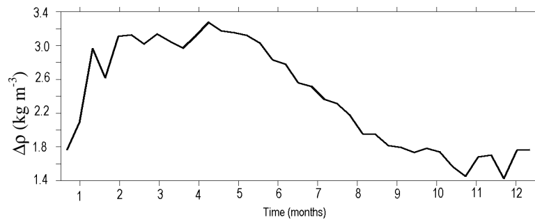
Fig. 6. Seasonal variations of the density difference at both sides of the Strait of Hormuz at a depth level of ~70 m.
