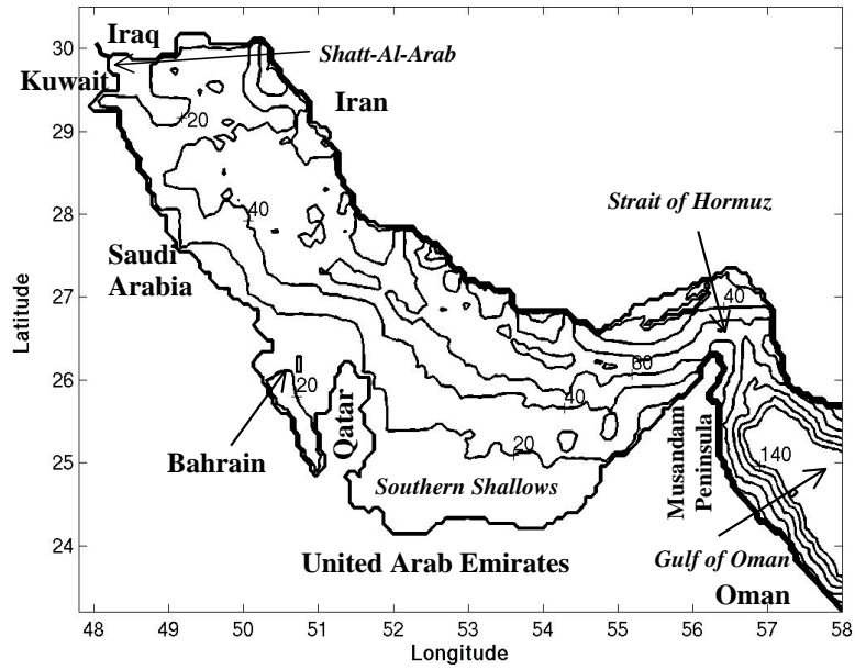
Fig. 1. Bathymetry (CI=20 m) used in this study.
