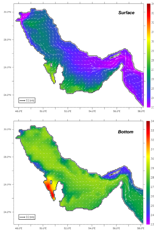
Fig. 8. Lateral distributions of surface and bottom flow vectors (arrows, \text{m s}^{-1} ) over density (colours, \text{sigma-t} , \text{kg m}^{-3} ) averaged over summer months (June–August).
