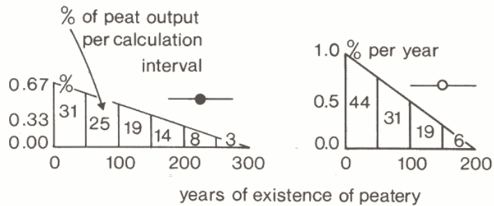
FIG. 2. Computation of the progress of peat exploitation in the Holland-Utrecht low peat region.
