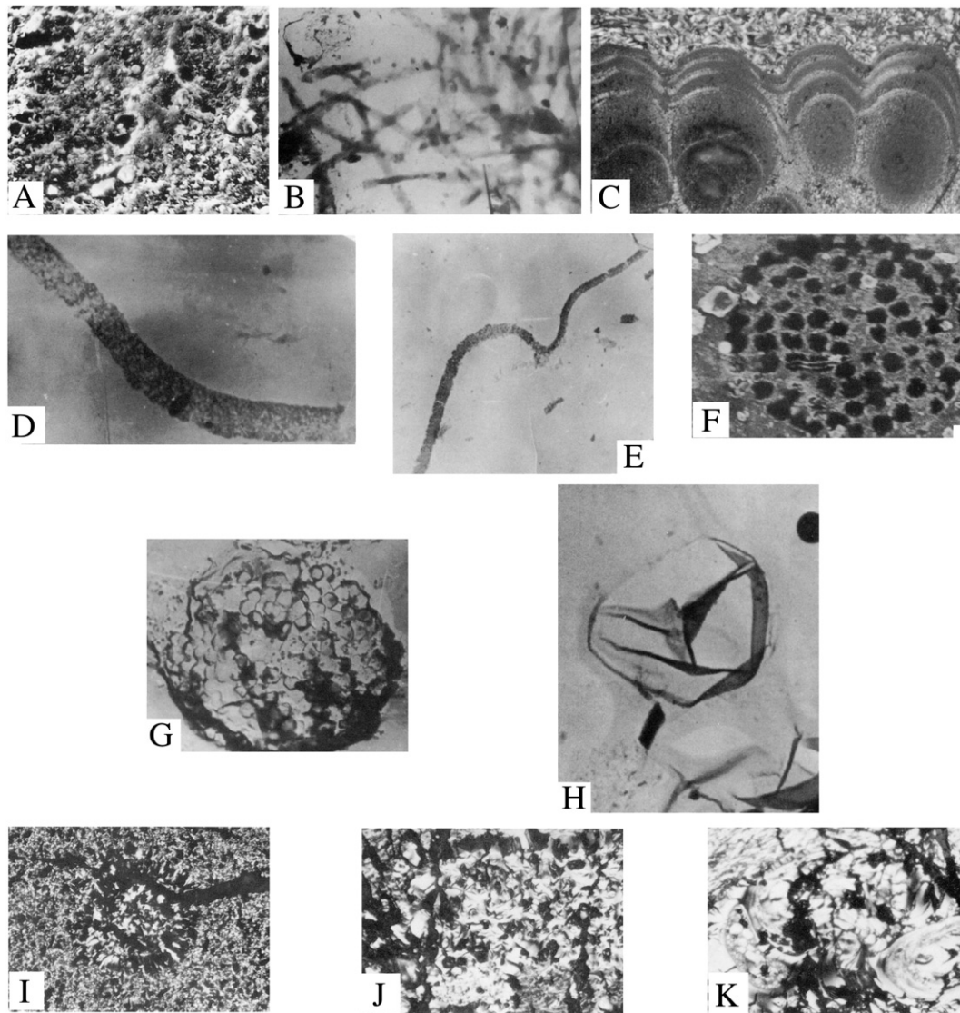
Fig. 2. A. Spropelic groundmass in the Early Paleozoic anthracite boghead from Xupu, Hunan. (SEM; field width 85 \mu\text{m} ). B. Nocardia ? sp. in the Middle Cambrian anthracite boghead from Pingli, Shaanxi (TEM; field width 15 \mu\text{m} ). C. Conical columnar stromatolite (algae) in the Early Silurian anthracite boghead from Ankang, Shaanxi (reflected light, crossed polars, oil immersion; field width 375 \mu\text{m} ). D. The filamentous alga Oscillatoropsis minuta in the Early Cambrian from Xupu, Hunan (TEM; field width 11.4 \mu\text{m} ). E. The filamentous alga Oscillatoropsis tenuis in the Early Cambrian anthracite boghead from Xupu of Hunan (TEM; field width 8.3 \mu\text{m} ). F. The cyanobacterium Sphaerocongrus wufengensis in the Middle Cambrian anthracite boghead from Xupu, Hunan (SEM; field width 4 \mu\text{m} ). G. The cyanobacterium Sphaerocongrus yinpingensis in the Middle Ordovician anthracite boghead from Dongkou, Hunan (SEM; field width 4 \mu\text{m} ). H. The acritarch Leiosphaeridia in the Cambrian anthracite boghead from Pingli, Shaanxi (TEM; field width 380 \mu\text{m} ). I. Fine mosaic texture of the Early Silurian anthracite boghead from Ankang, Shaanxi (reflected light, oil immersion; field width 160 \mu\text{m} ). J. Coarse mosaic texture of the Middle Cambrian anthracite boghead from Ziyang, Shaanxi (reflected light, oil immersion; field width 160 \mu\text{m} ). K. Leafy and spherical anisotropic carbon in the Early Silurian anthracite boghead from Ziyang, Shaanxi (reflected light, oil immersion; field width 160 \mu\text{m} ).
