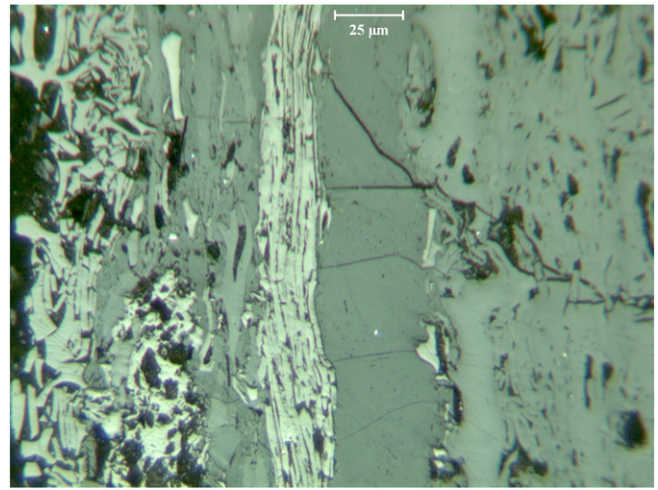
Fig. 7. Low-reflecting inertinite in a Permian Gondwana coal from Mozambique (image Moz 01 09). Photo by Hower and Wagner.
