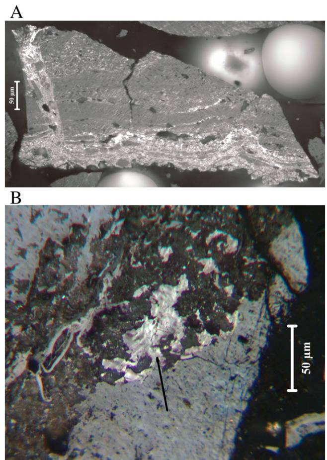
Fig. 8. A. Natural graphite occurring in a coal adjacent to a dolerite intrusion in South Africa. B. Pyrolytic carbon in Permian Matla coal, Witbank coalfield, about 0.7% R_{\text{mean}} . Photos by Hower and Wagner.
