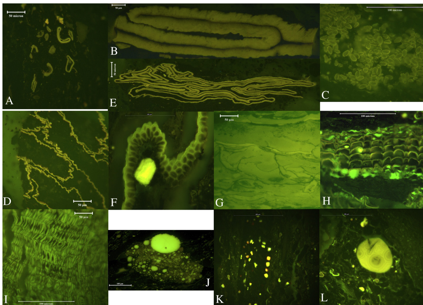
Fig. 9. Changing aspects of liptinite through time. All images are in blue-light illumination. A. Sporinite. Miospores in the Carboniferous Moscow Basin; Seredin collection coal; Photo by Hower. B. Sporinite. A megaspore in the Permian from China; Photo by Hower. C. Sporinite. Pollen from the middle Eocene Claiborne Formation of Kentucky, USA; Photo by O'Keefe. D. Cutinite. "Classic" toothed cutinite from the Carboniferous of Mongolia; USGS World Coal Quality Collection; Photo by Hower. E. Cutinite. Thin cutinite; Photo by Hower. F. Cutinite. Thick, layered cutinite from the middle Eocene Claiborne Formation of Kentucky, USA; Photo by O'Keefe. G. "Barkinite"-type suberinite. Liptinitic material separated by very thin cellular divisions; Photo by Hower. H. Suberinite. Thin form from the middle Eocene Claiborne Formation of Kentucky, USA; Photo by O'Keefe. I. Suberinite. Thick form from the middle Eocene Claiborne Formation of Kentucky, USA; Photo by O'Keefe. J. Resinite. Jurassic from the Sinai Peninsula; Photo by Hower. K. fluorinite-type Resinite in textinite through the middle of field of view. Middle Eocene Claiborne Formation of Kentucky, USA; Photo by O'Keefe. L. Resinite. Zoned resinite from the Middle Eocene Claiborne Formation of Kentucky; Photo by O'Keefe.
