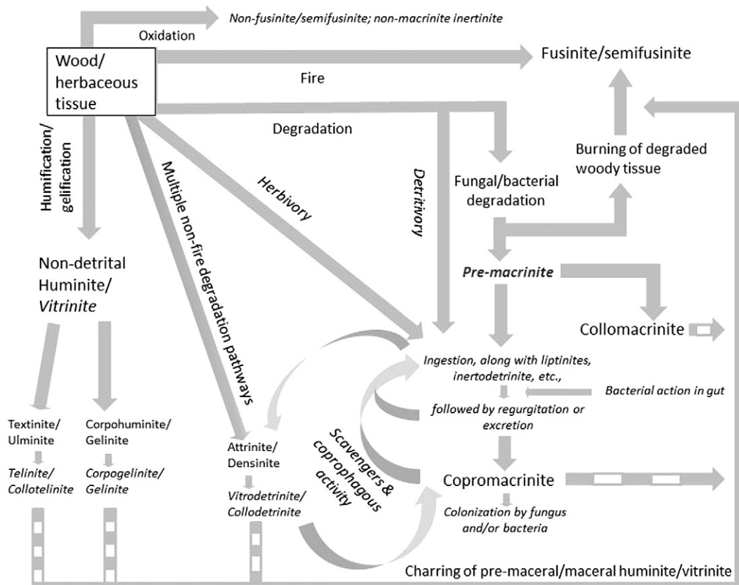
Fig. 3. Developmental pathways of helophytic-derived macerals. Liptinite and non-wood-origin inertinite (resin-derived secretinite and funginite) are not directly included as end products. Funginite, as fungus, is part of the process. The charring of pre-maceral huminite or huminite or vitrinite macerals is not necessarily a continuing step in maceral formation and the end product, while located close to primary fusinite/semifusinite on the chart, has a different origin than primary fusinite/semifusinite. This distinction is a necessary part of the description of the macerals. The naming of the inclusion-free collomacrinite and the complex copromacrinite is a convenience in the description of the maceral origins and does not represent formally accepted maceral nomenclature.
