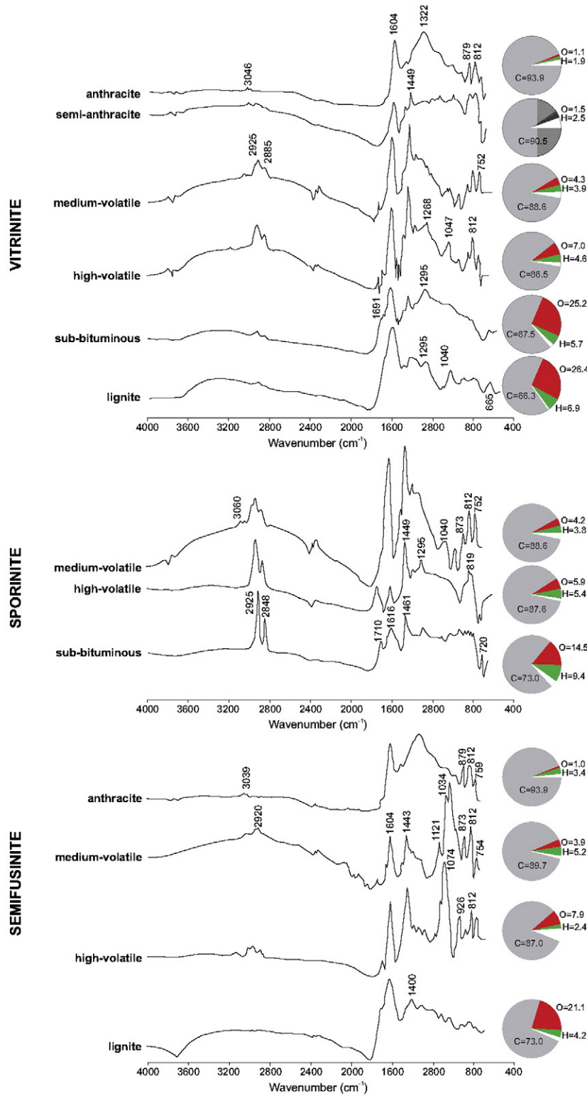
FTIR spectra and elemental composition of vitrinite, sporinite and semifusinite from lignite to anthracite.
