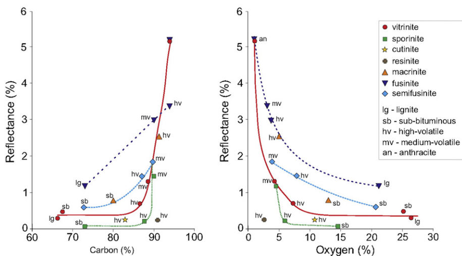
Fig. 12. Carbon and oxygen content of individual macerals of different coal ranks. Each point of the diagrams represent average value of numerous analyses obtained with electron microprobe. Note different paths of vitrinite, sporinite, semifusinite, and fusinite. Other macerals (macrinite, resinite, cutinite) were available only sporadically and this is why are represented only once or twice.
