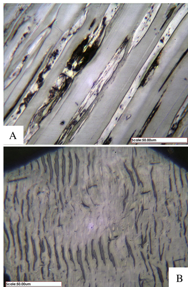
Fig. 5. Examples of vitrinite macerals in etched anthracite coal. A is telovitrinite; B is telovitrinite with resinite. Photos by Eble.
