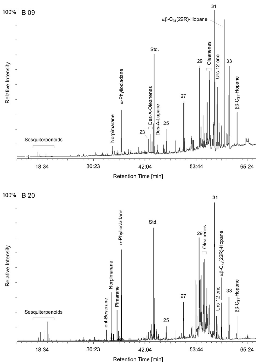
Fig. 14. Gas chromatograms (total ion current) of the saturated hydrocarbon fractions of the samples B 09 and B 20 from the Bourgas coal seam. n -Alkanes are labeled according to their carbon number. Std. = Standard (deuterated n -tetracosane). Refigured from Bechtel et al. (2005).
