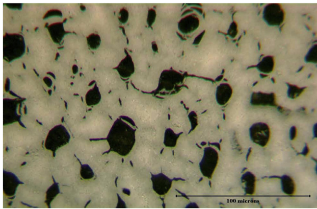
Fig. 6. Fusinite showing evidence of significant degradation prior to combustion. Note the delaminated cell walls and internal cracking. China (Permain, Yunnan Province) coal sample CN 87 02 – fusinite. Refigured from figure 8 of Dennen et al. (2010).
