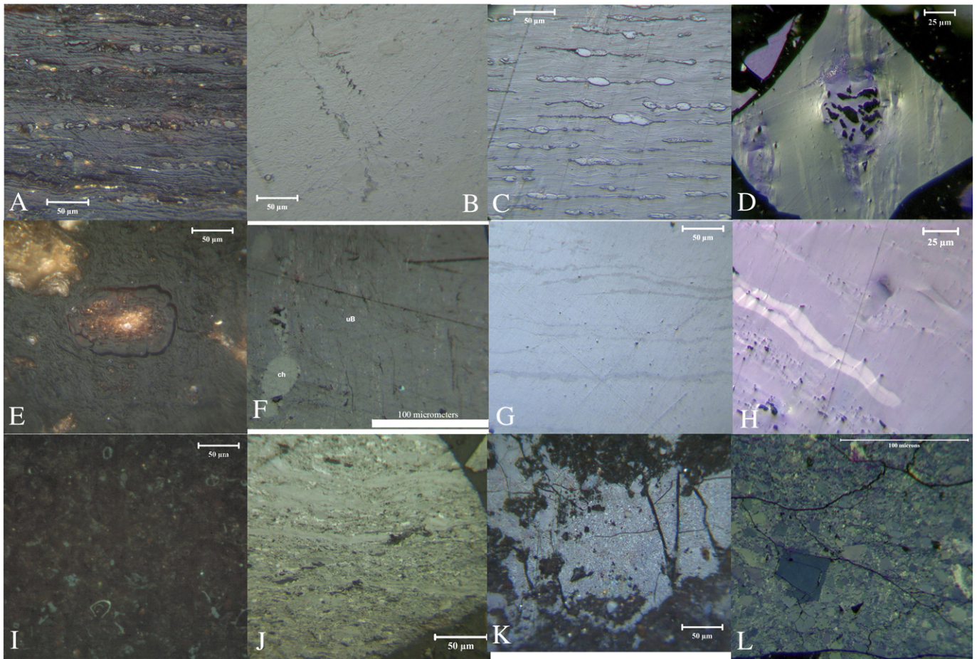
Fig. 4. Examples of “typical” humite/vitrinite macerals through a rank series from peat (leftmost image) to lignite/brown coal (image second from left) to bituminous coal (image second from right) to anthracite (image on right). Fig. 4-1: A–D, textinite/telinite series; E–H, ulminite/collotelinite series; I–L, attrinite–vitrodetrinite series. Fig. 4-2: M–P, densinite/collodetrinite series; Q–T, corpohuminite–corpogelinite series; and U–X, gelinite series. A. Textinite. Neogene peat from Centralia Washington, USA; photo by Hower. B. Textinite. Cenozoic lignite from Tahlesel, Bohemia, Germany (now the Czech Republic); from the Vanderbilt coal collection; photo by Hower. C. Telinite with corpogelinite. Kimmeridgian of New Jersey, USA; photo by Hower. D. Telinite. Asturian of Schuylkill Co., PA, USA; Photo by Hower. E. Ulminite. Peat from Kerry Bog, Ireland; Photo by Hower. F. Ulminite with corpohuminite. Middle Eocene Claiborne Lignite from Kentucky, USA; photo by O’Keefe. G. Telinite with faint cutinite. Triassic of Virginia, USA; Photo by Hower. H. Telinite with sporinite from a megaspore. Asturian of Schuylkill Co., PA, USA; Photo by Hower. I. Attrinite. Recent Indonesian Peat. Photo by Esterle. J. Attrinite. Miocene Eel River Coal, Mendocino Co., California, USA; Photo by Hower. K. Vitrodetrinite. Permian Heshan coalfield, Guangxi, China; Photo by Hower. L. Vitrodetrinite. Permian of Guangdong, China; Photo by Hower. M. Densinite. Modern Loose Compost, Rowan County, KY; Photo by O’Keefe. N. Densinite. Miocene of Slovakia; Photo by Hower. O. Collodetrinite. Aptian Wulantuga Coal of Inner Mongolia, China; Photo by Hower. P. Collodetrinite. Permian of Chongqing, China. Photo by Hower. Q. Corpogelinite. Recent Indonesian Peat. Photo by Esterle. R. Corpogelinite. Paleocene Buelah Zap from North Dakota, USA; Photo by Hower. S. Corpogelinite. Pennsylvanian of Bell County, KY; Photo by Hower. T. Corpogelinite. Permian of South Africa; Photo by Hower. U. Gelinite. Modern drift wood from Holden Beach, North Carolina, USA; Photo by Hower. V. Gelinite. Cenozoic brown coal from Dambroich bei Bonn, Germany; Vanderbilt Coal Collection; Photo by Hower. W. Gelinite. Asturian from Tioga County, Pennsylvania, USA; Photo by Hower. X. Gelinite. Asturian Buck Mountain Coal, Schuylkill County, PA, USA; Photo by Hower.
