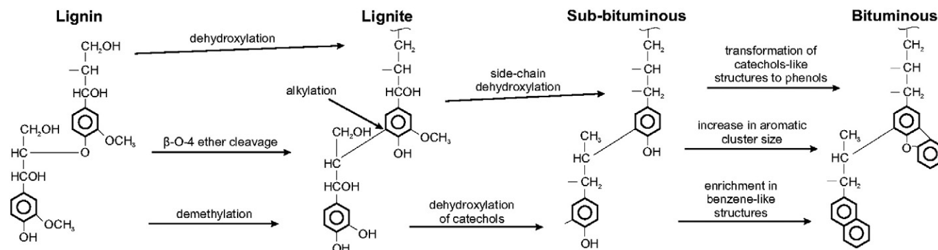
Fig. 11. Chemical transition from wood to peat, showing the elimination of cellulose and transformation of lignin. Modified after Hatcher and Clifford (1996).
