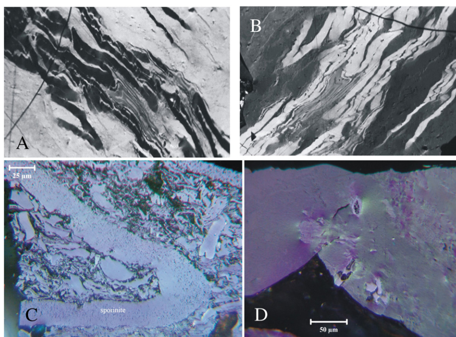
Fig. 10. A & B. Orthogonal views sporinite in Pennsylvanian anthracite ( R_{\max} > 5\% ), Southern Anthracite Field, Pennsylvania. Scale = ca. 250 \mu\text{m} on long axis. Oil immersion, 50 \times objective, crossed-polars. C. Sporinite in European anthracite ( R_{\max} = 3.89\% ). Scale = 25 \mu\text{m} . Oil immersion, 50 \times objective, crossed-polars with wavelength plate. D. Funginite (upper center) in vitrinite in European semianthracite ( R_{\max} = 2.86\% ). Scale = 50 \mu\text{m} . Oil immersion, 50 \times objective, crossed-polars with wavelength plate. Photos by Hower.
