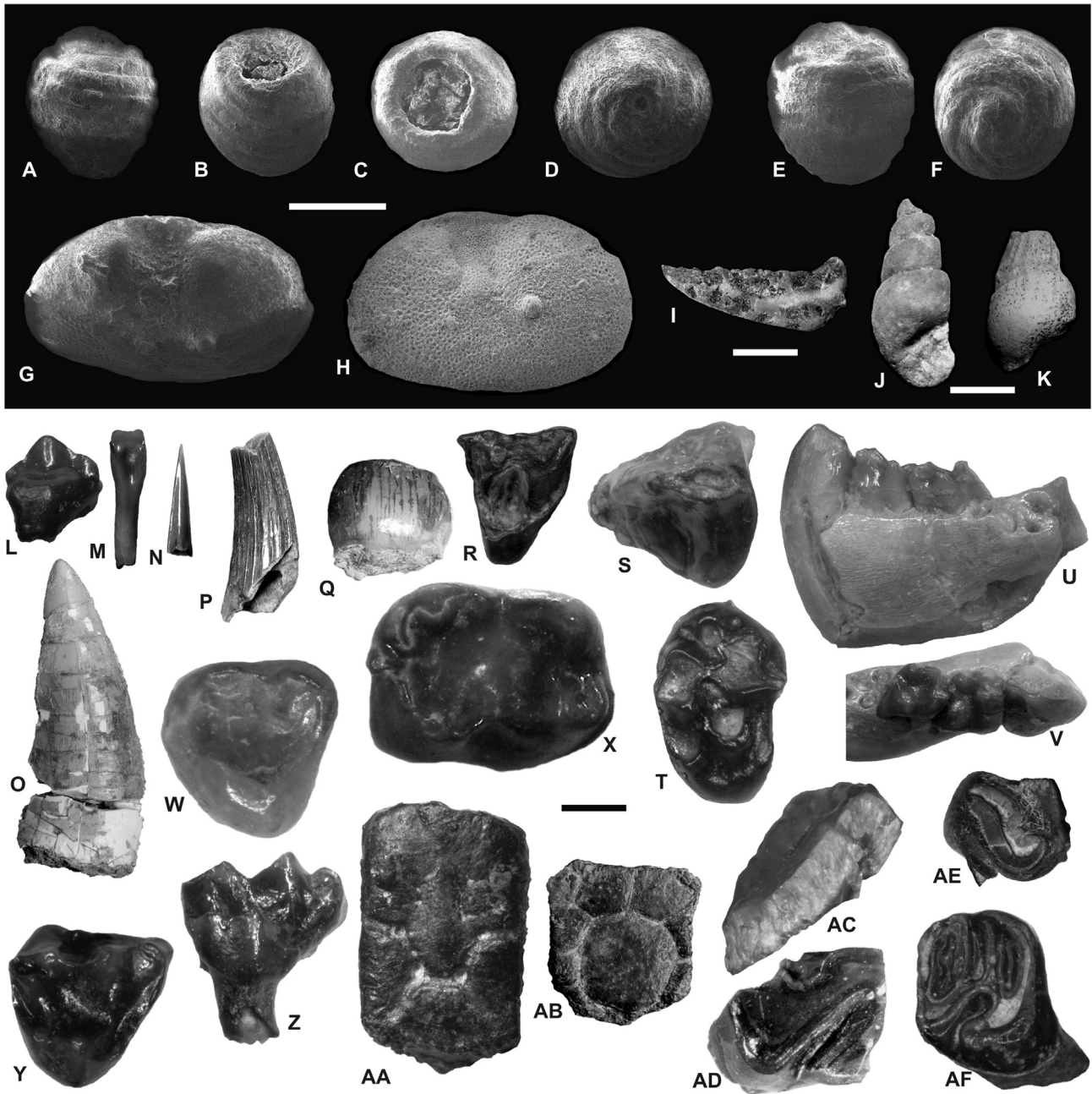
Fig. 6. Selected fossils from the Lower Pozo Formation, Contamana, Peruvian Amazonia. Quebrada Cachiyacu section (late middle Eocene localities). A–F: Charophyte gyrogonites: A: Nodosochara jerbae , in lateral view (CTA-47 locality); B–D: Raskyella pecki meridionale , in lateral (B; CTA-66 locality), apical (C; CTA-51 locality), and basal views (D; CTA-51 locality); E–F: Stephanochara acris , CTA-27 locality, in lateral (E) and apical views (F). G–H: Ostracoda: G: Neocyprideis apostolescui , left valve in lateral view (CTA-27); H: Ilyocypris aff. lusitanica , left valve in lateral view (CTA-27). I: Decapoda: trichodactylid crab claw (MUSM 2264; CTA-27). J–K: Gastropoda: J, unidentified pachychilid, in front view (MUSM 2265; CTA-27); K: Charadreon sp., in rear view (MUSM 2266; CTA-41). L–N: Actinopterygii: L: Colossoma , tooth in buccal view (MUSM 2267; CTA-27); M: Leporinus sp., tooth in palatine view (MUSM 2268; CTA-27). N: cf. Hydrolycus (MUSM 2269; CTA-27). O, Sebecosuchia: cf. Sebecus , tooth in lateral view (MUSM 1959; CTA-47). P–Q, Eusuchia: P: unidentified gavialoid tooth (MUSM 2270; CTA-27); Q: unidentified durophagous caimanine tooth (MUSM 2271; CTA-27). R: Metatheria: Rumiodon sp., left M2 in occlusal view (MUSM 2272; CTA-27). S–Z: Marsupialia: S–V: Wamradolops sp. (CTA-27). S, left P3 in occlusal view (MUSM 2273); T: right M1, in occlusal view (MUSM 2554); U–V: right hemimandible with p3–m2 and alveoli of m3 in lingual (U) and occlusal views (V) (MUSM 2555); W–X: Sasawatsu sp. (CTA-27). W, right M3 in occlusal view (MUSM 2556); X: right m3 in occlusal view (MUSM 2557); Y–Z: cf. Perulestes sp. 2 (MUSM 2558; CTA-27), right M2 in occlusal (Y) and linguo-occlusal view (Z). AA–AB: Xenarthra, Cingulata: AA, Stegosimpsonia sp., osteoderm in dorsal view (MUSM 2559; CTA-66); AB: Eocoleophorus glyptodontoides , osteoderm in dorsal view (MUSM 1586; CTA-29). AC: Pyrotheria: cf. Griphodon , enamel fragment in lateral view (MUSM 2560; CTA-27). AD–AE: Notoungulata (CTA-27): AD: “ Eohyrax–Pseudhyrax–Punahyrax ”, right p3–4, fragmentary, in occlusal view (MUSM 2561); AE: Unidentified intertheriid or “archaeohyracid”, left upper cheek tooth fragment with closed fossette in occlusal view (MUSM 2562). AF: Rodentia: Cachiyacuy cf. contamanensis , right M2 in occlusal view (MUSM 2563; CTA-29). Scale bars = 500 \mu m (A–H, S–T, W–X), 1 mm (R, U–V, Y–Z, AD, AF), 2 mm (J–N, Q, AA, AC, AE), 5 mm (I), 10 mm (O, AB).
