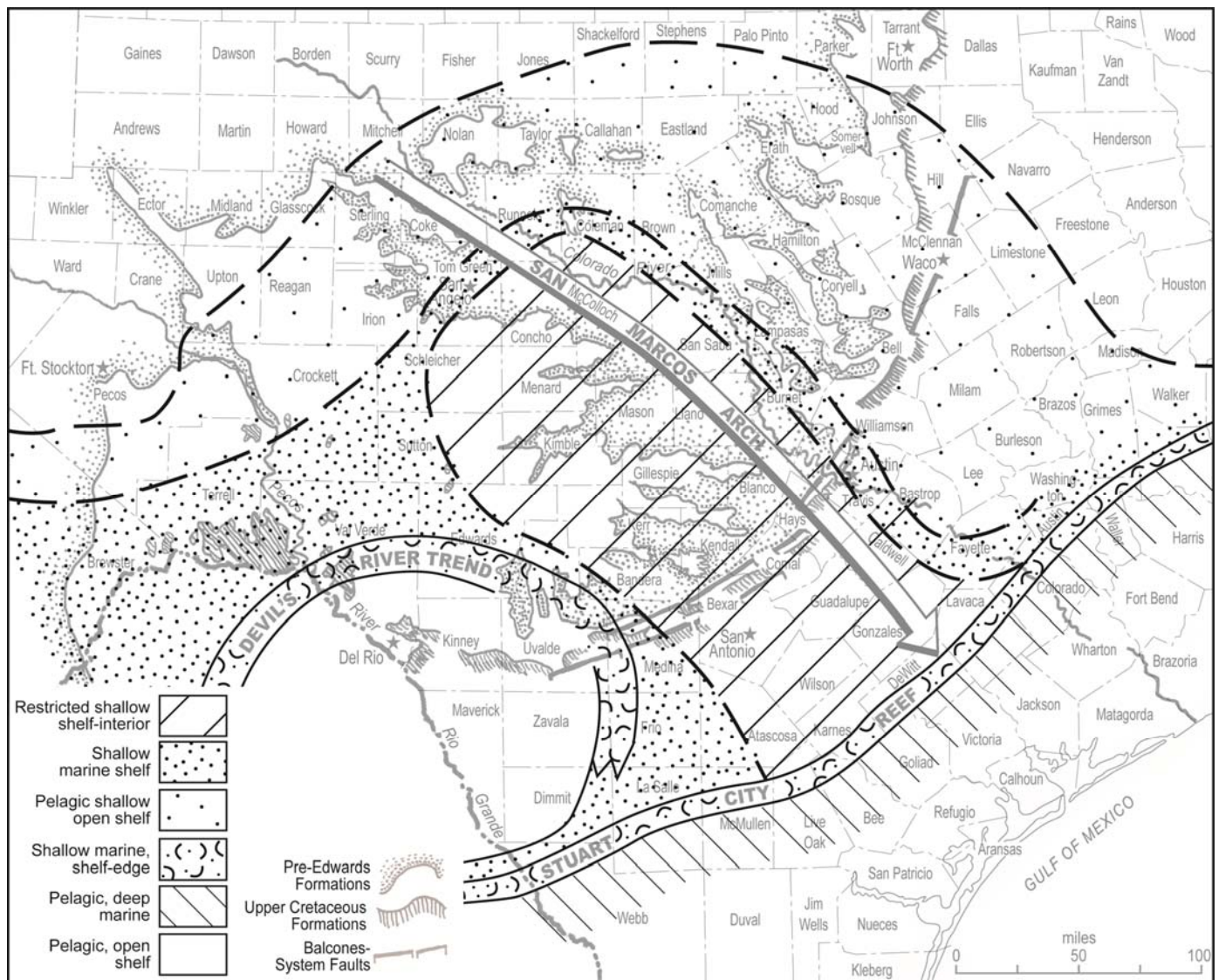
Figure 9. Regional depositional environments, upper Albian (after Rose, 1972; Smith et al., 2000).
