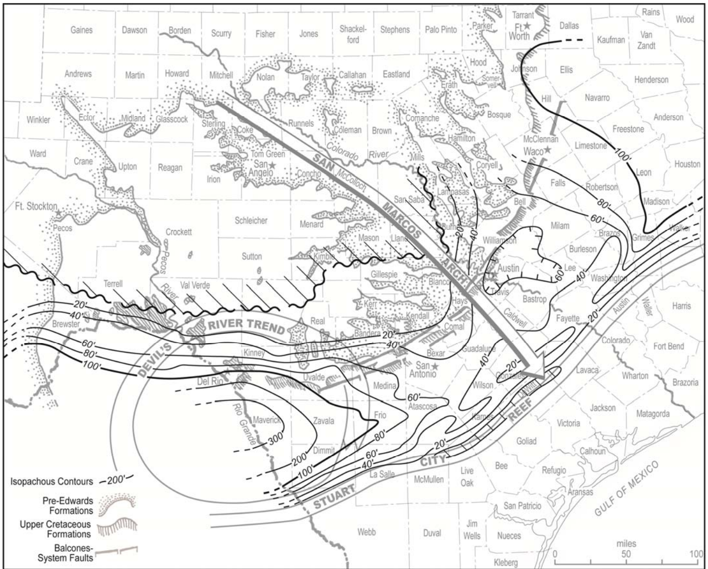
Figure 10. Isopach map of the Del Rio Clay (from Maxwell et al., 1967; Rose, 1972, 1986b; Smith et al., 2000).
