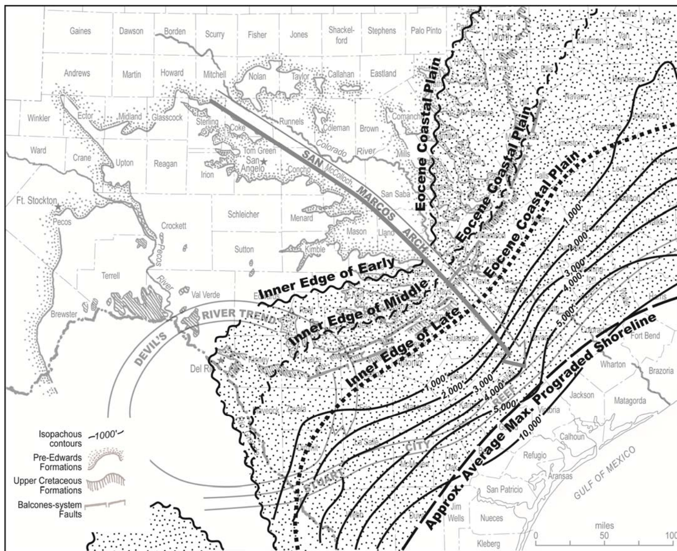
Figure 20. Eocene isopach and depositional environments (from Cook and Bally, 1975; Galloway et al., 2011).
