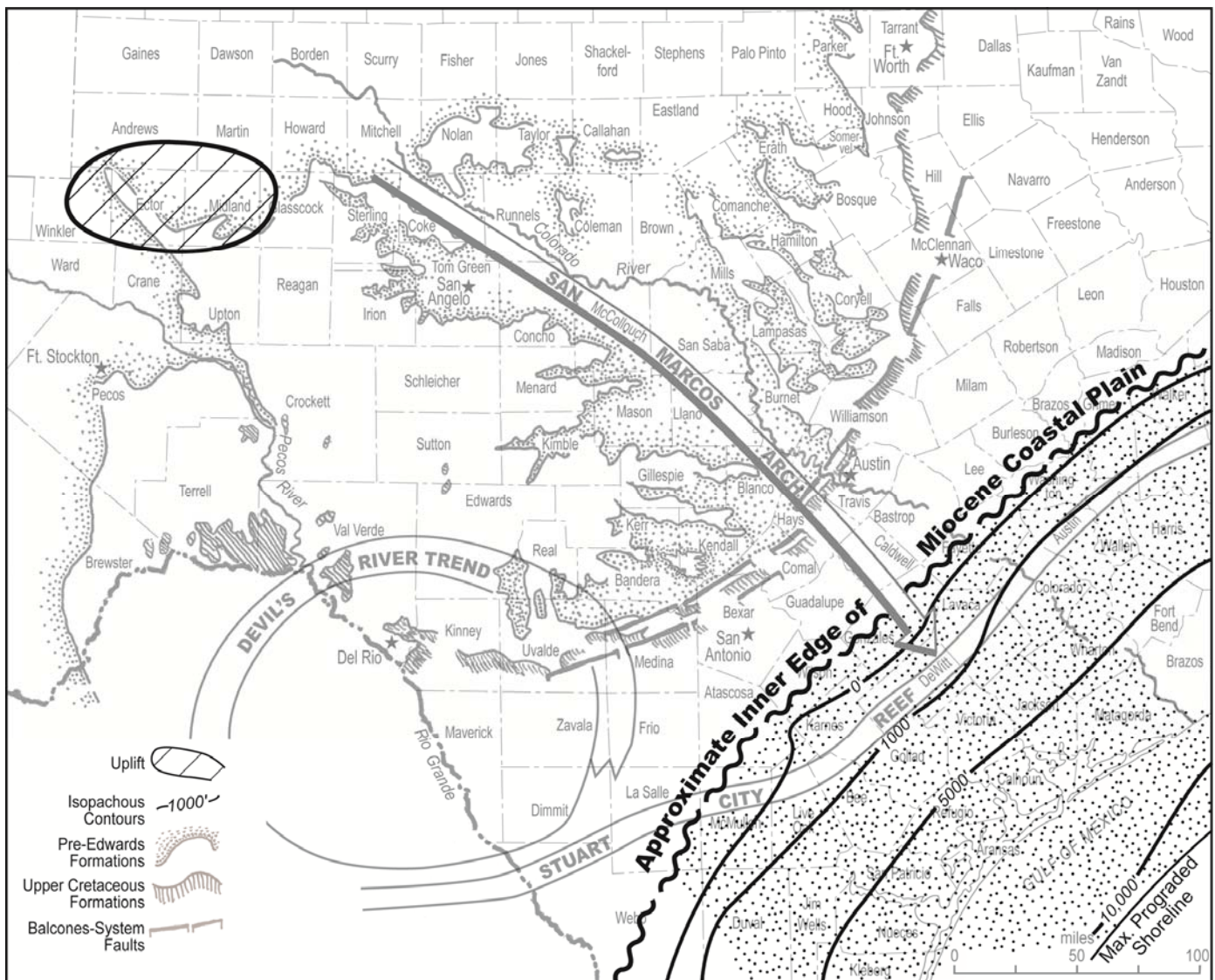
Figure 23. Miocene isopach and depositional environments (from Cook and Bally, 1975; Galloway et al., 2011).
