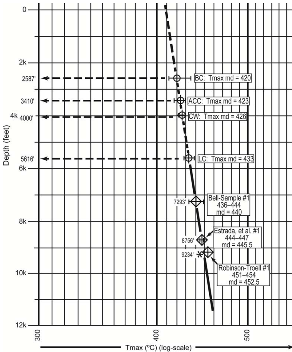
Figure 26. Tmax of surface samples (Eagle Ford Formation) plotted on subsurface depth vs. Tmax profile. First Shot Field, Central Texas (after Edman, 2012; A. Miceli-Romero, 2015, personal communication).
