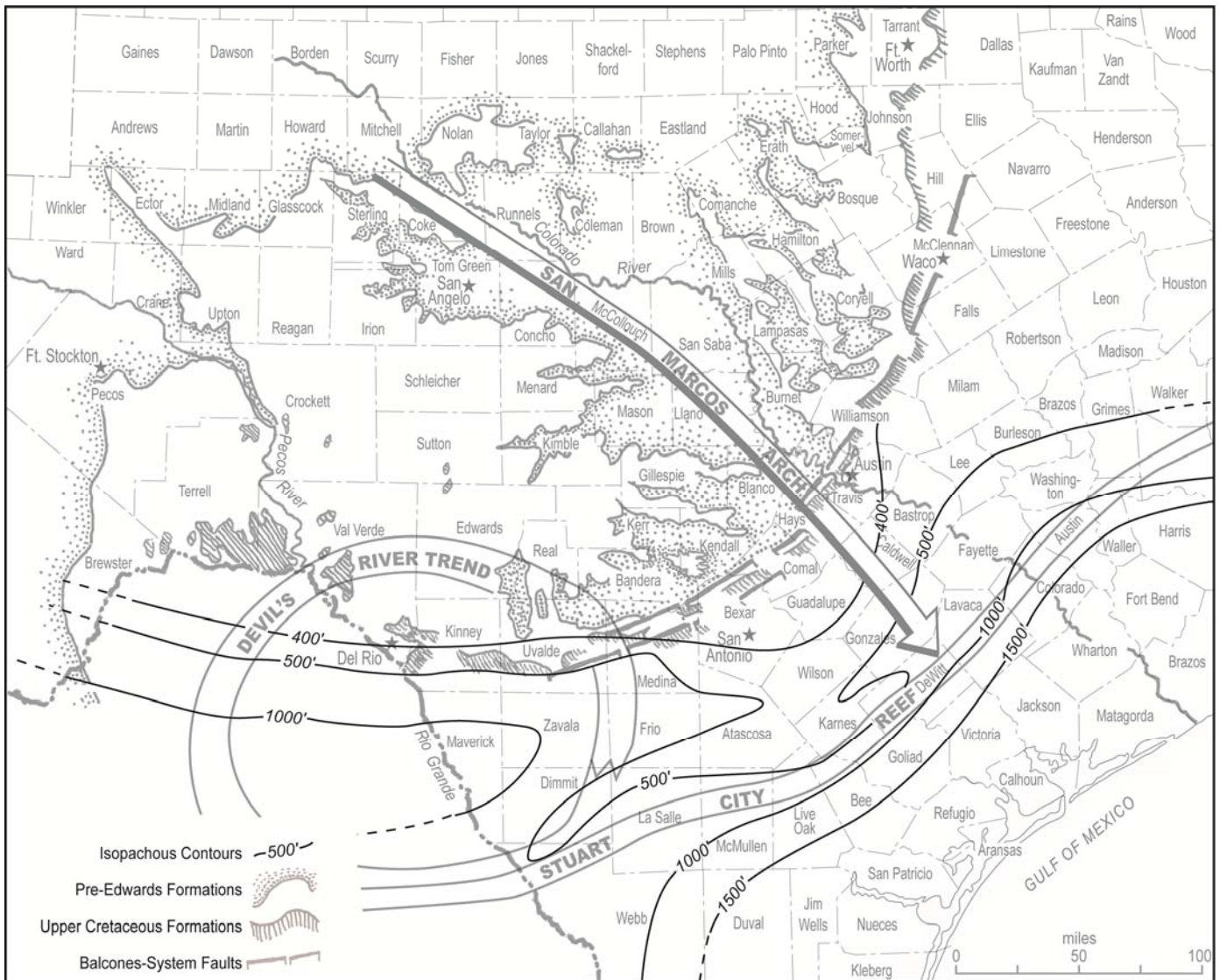
Figure 16. Isopach map of Austin Chalk and equivalents (from Maxwell et al., 1967; Cook and Bally, 1975; Texas Bureau of Economic Geology, Geologic Atlas of Texas (Del Rio [1977], Emory Peak–Presidio [1979], Fort Stockton [1982], Pecos [1975], San Angelo [1976], San Antonio [1983], and Sonora [1981] sheets).
