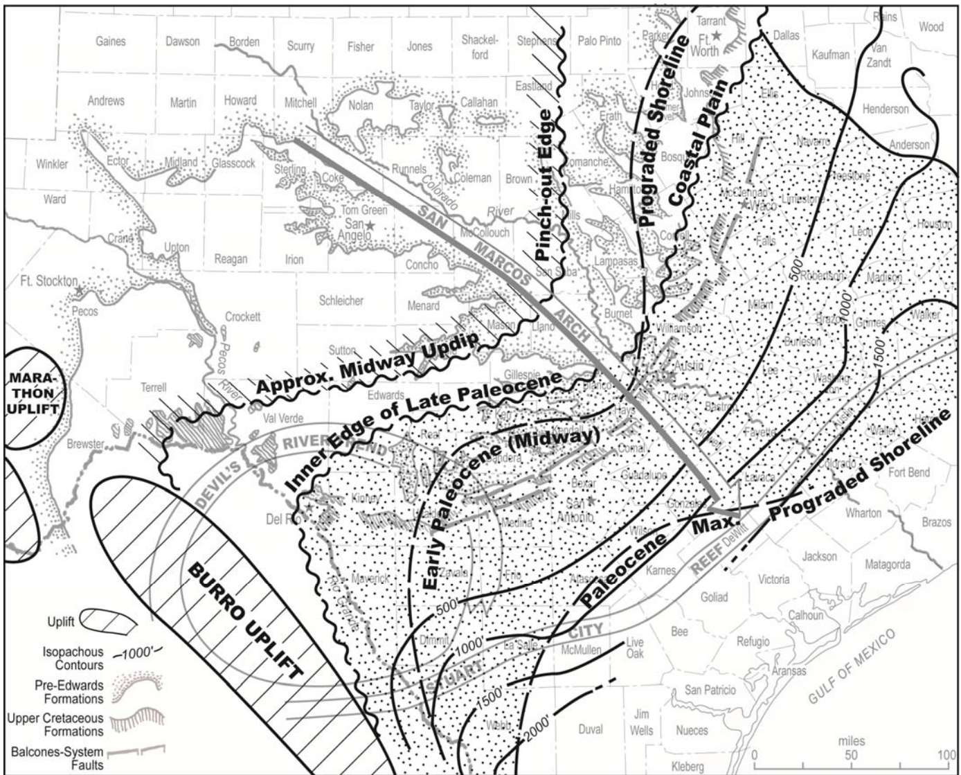
Figure 19. Paleocene isopach and depositional environments (from Cook and Bally, 1975; Galloway et al., 2011).
