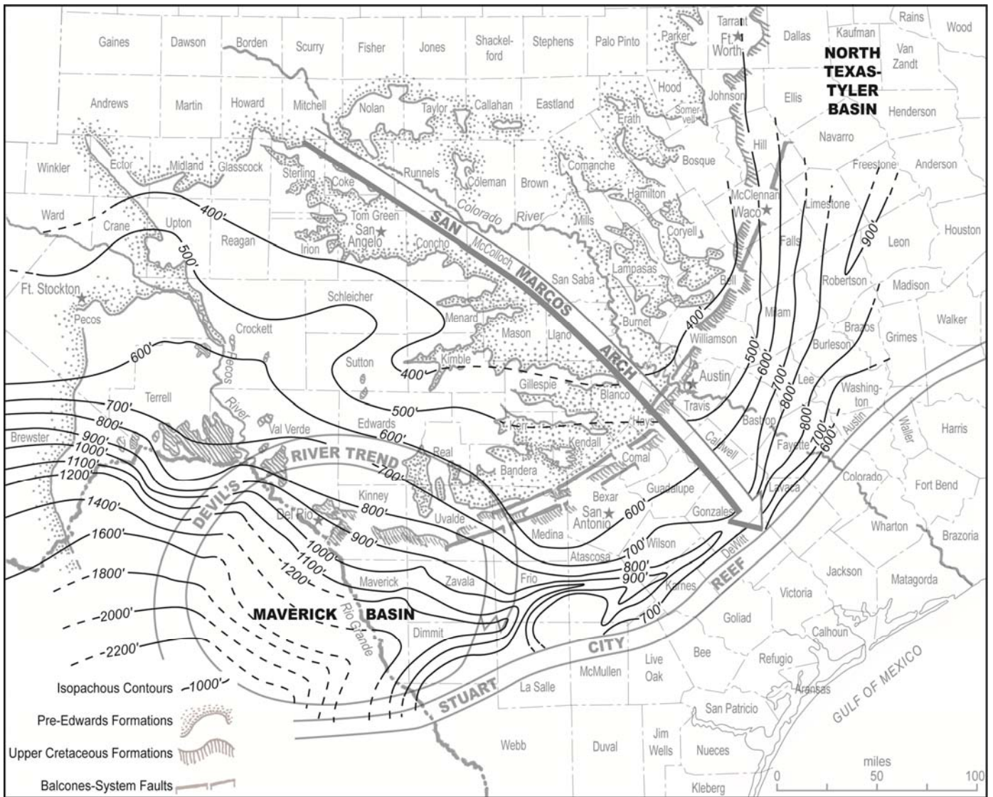
Figure 8. Isopach map of Edwards Group and associated formations (Washita-Fredericksburg Division) (after Rose, 1972, 1986a, 2004).
