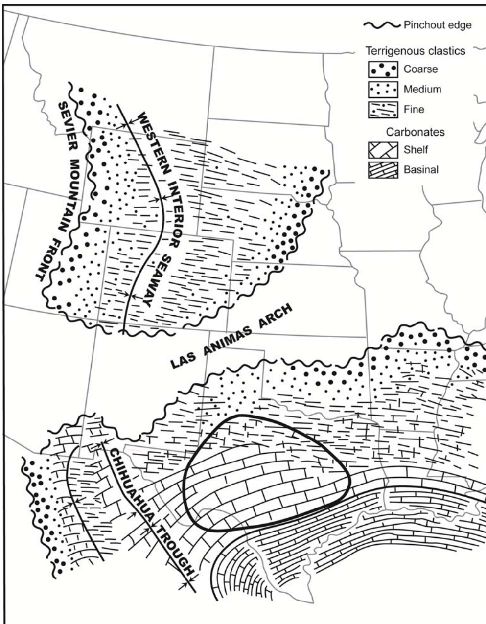
Figure 13. Generalized paleogeography, Cretaceous Western Interior Seaway, Wyoming to Texas (from Rose, 1972; Cook and Bally, 1975; Kauffmann, 1977; Scott et al., 2013).
