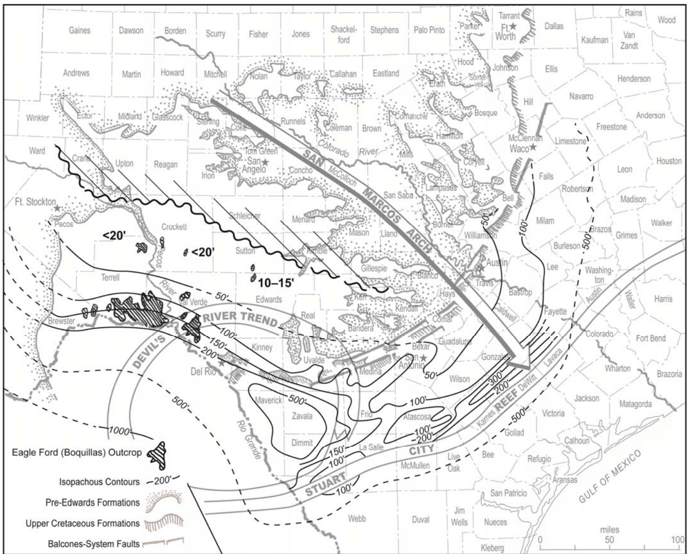
Figure 15. Isopach map of Eagle Ford-Boquillas Formation (from Maxwell et al, 1967; Rose, 1972; Cook and Bally, 1975; Texas Bureau of Economic Geology, Geologic Atlas of Texas (Del Rio [1977], Emory Peak-Presidio [1979], Fort Stockton [1982], Llano [1981], Pecos [1975], San Angelo [1976], San Antonio [1983], and Sonora [1981] sheets).
