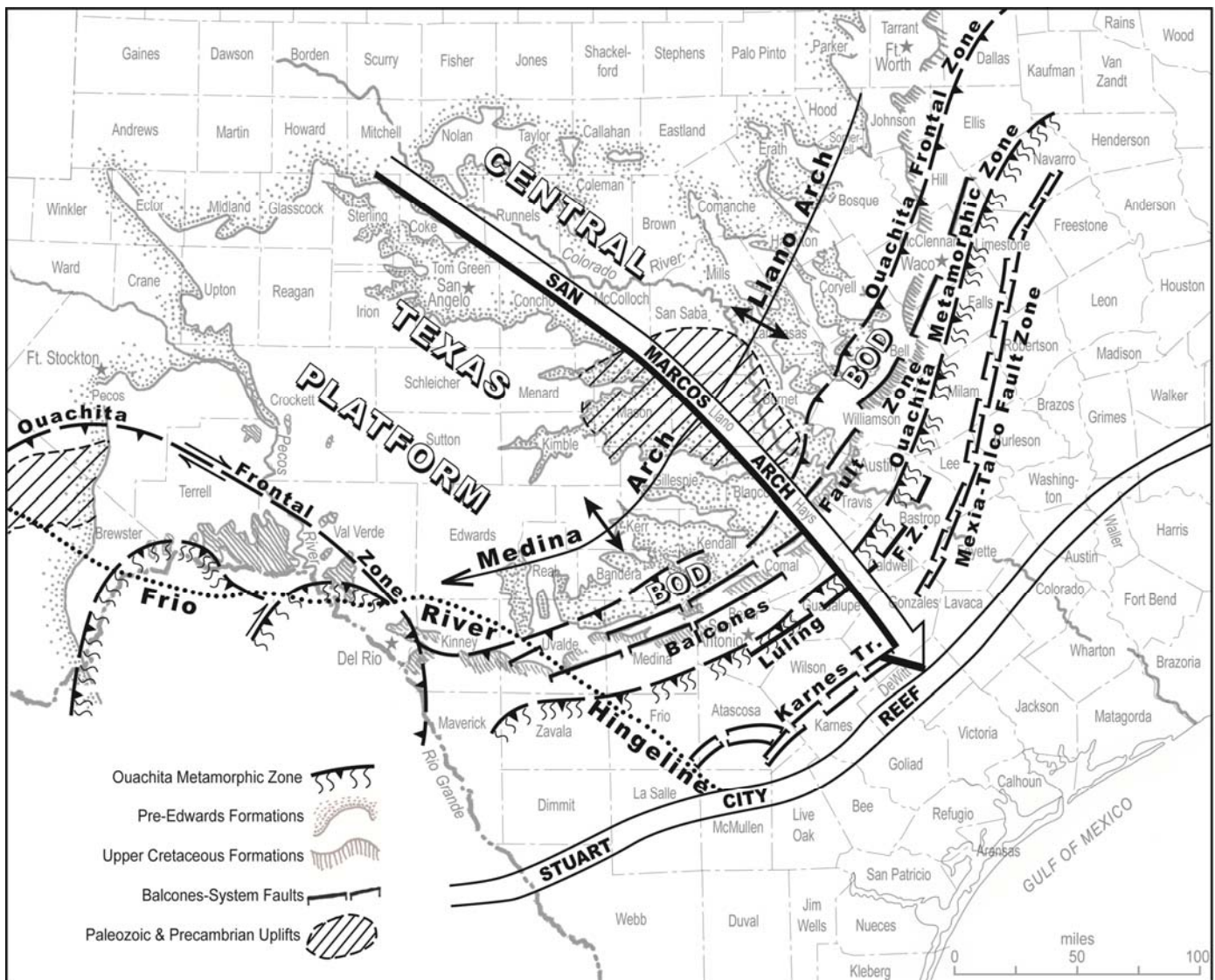
Figure 2. Regional structural elements, Central Texas. BOD, Balcones/Ouachita Downward.
