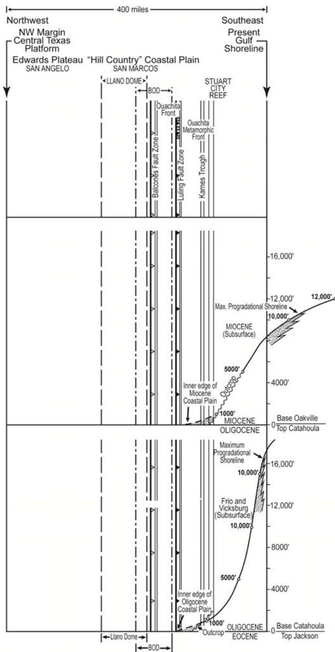
Figure 21. Projected northwest thinning of Oligocene and Miocene formations along San Marcos Arch from Gulf Coastal Plain toward Balcones Fault Zone.
