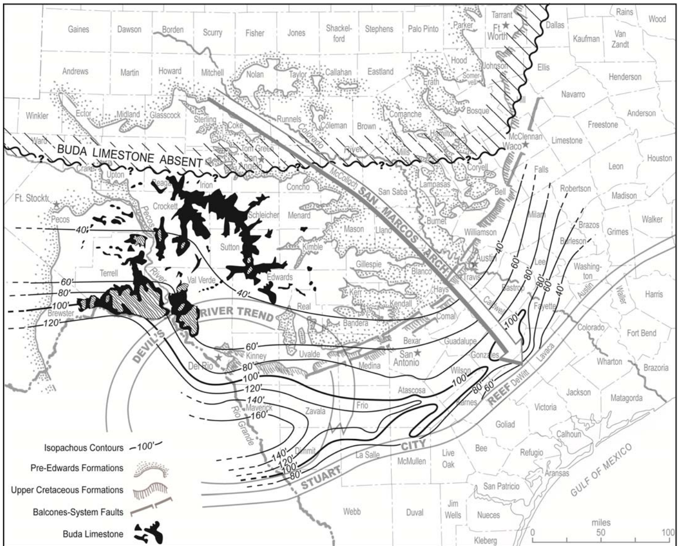
Figure 11. Isopach map of the Buda Limestone, with remnant outcrops on Edwards Plateau (from Maxwell et al., 1967; Rose, 1972, 1986a, 1986b; Smith et al., 2000; Texas Bureau of Economic Geology, Geologic Atlas of Texas [Del Rio [1977], Fort Stockton [1982], Llano [1981], Pecos [1975], San Angelo [1976], San Antonio [1983], and Sonora [1981] sheets).
