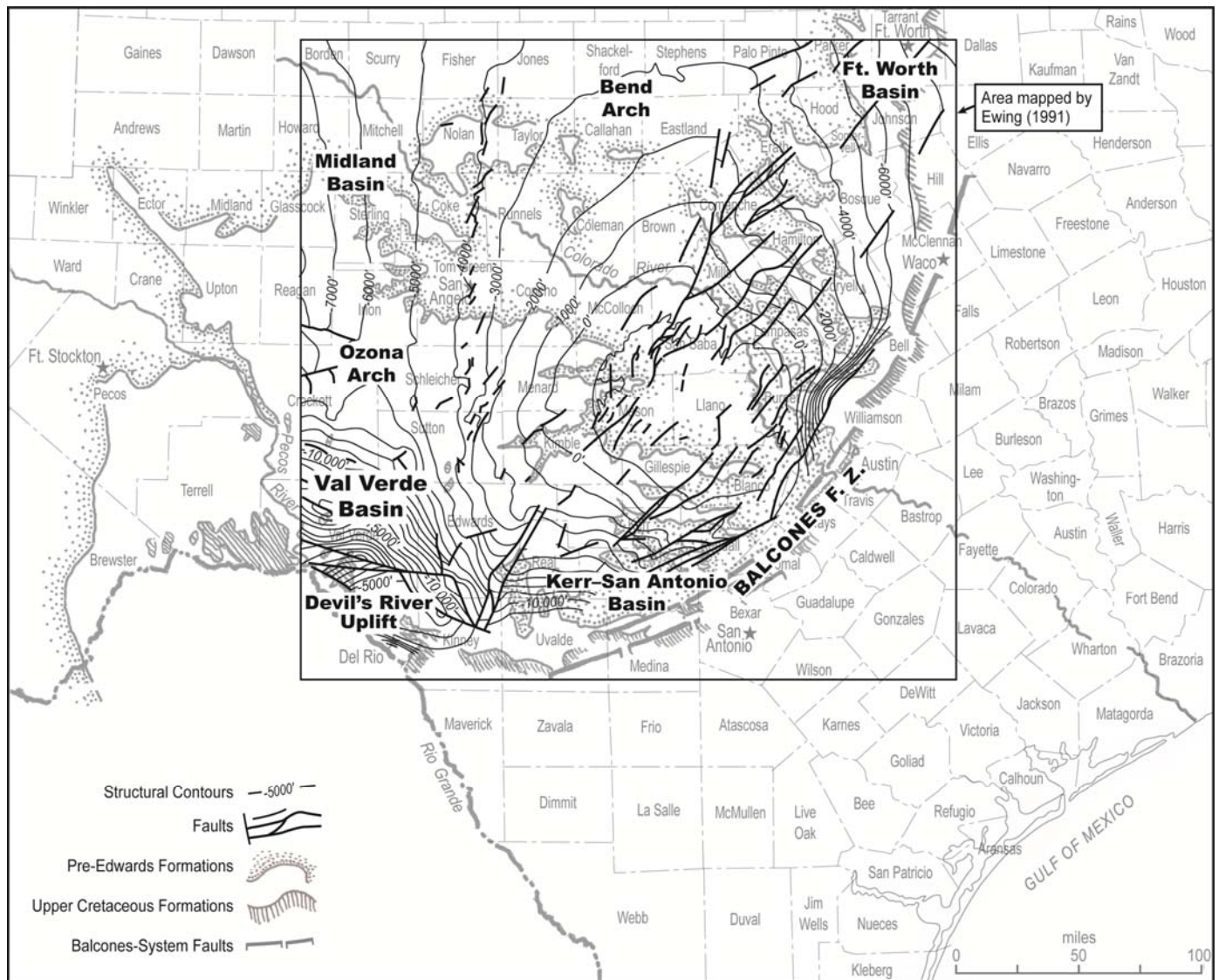
Figure 4. Structure on top Ellenburger Group (Lower Ordovician), Central Texas (from Ewing, 1991).
