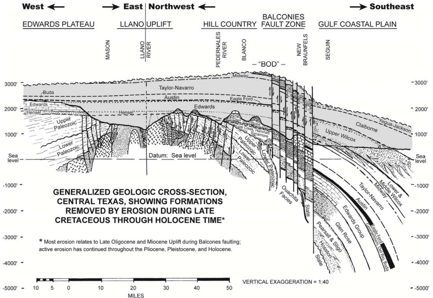
Figure 29. Generalized geologic cross-section, Central Texas, at present time, showing formations removed by Late Cretaceous through Holocene erosion; datum = modern sea-level; shaded area shows geologic section removed by post-Eocene erosion.
