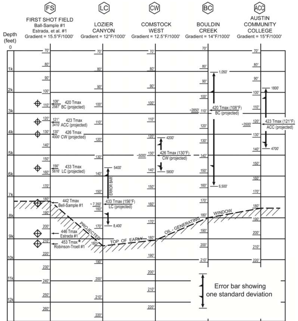
Figure 27. Projected depth of burial of four Eagle Ford–Boquillas surface samples based on subsurface depth vs Tmax profile, First Shot Field (Eagle Ford Formation), Texas, adjusted for geothermal gradients of surface localities.
