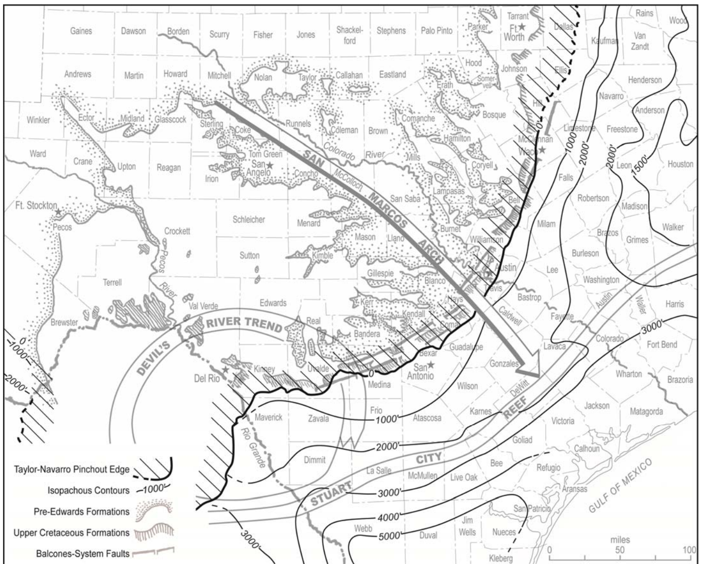
Figure 17. Isopach map of Taylor and Navarro groups (from Maxwell, 1967; Cook and Bally, 1975; Texas Bureau of Economic Geology, Geologic Atlas of Texas (Del Rio [1977], Emory Peak–Presidio [1979], Fort Stockton [1982], Pecos [1975], San Angelo [1976], San Antonio [1983], and Sonora [1981] sheets).
