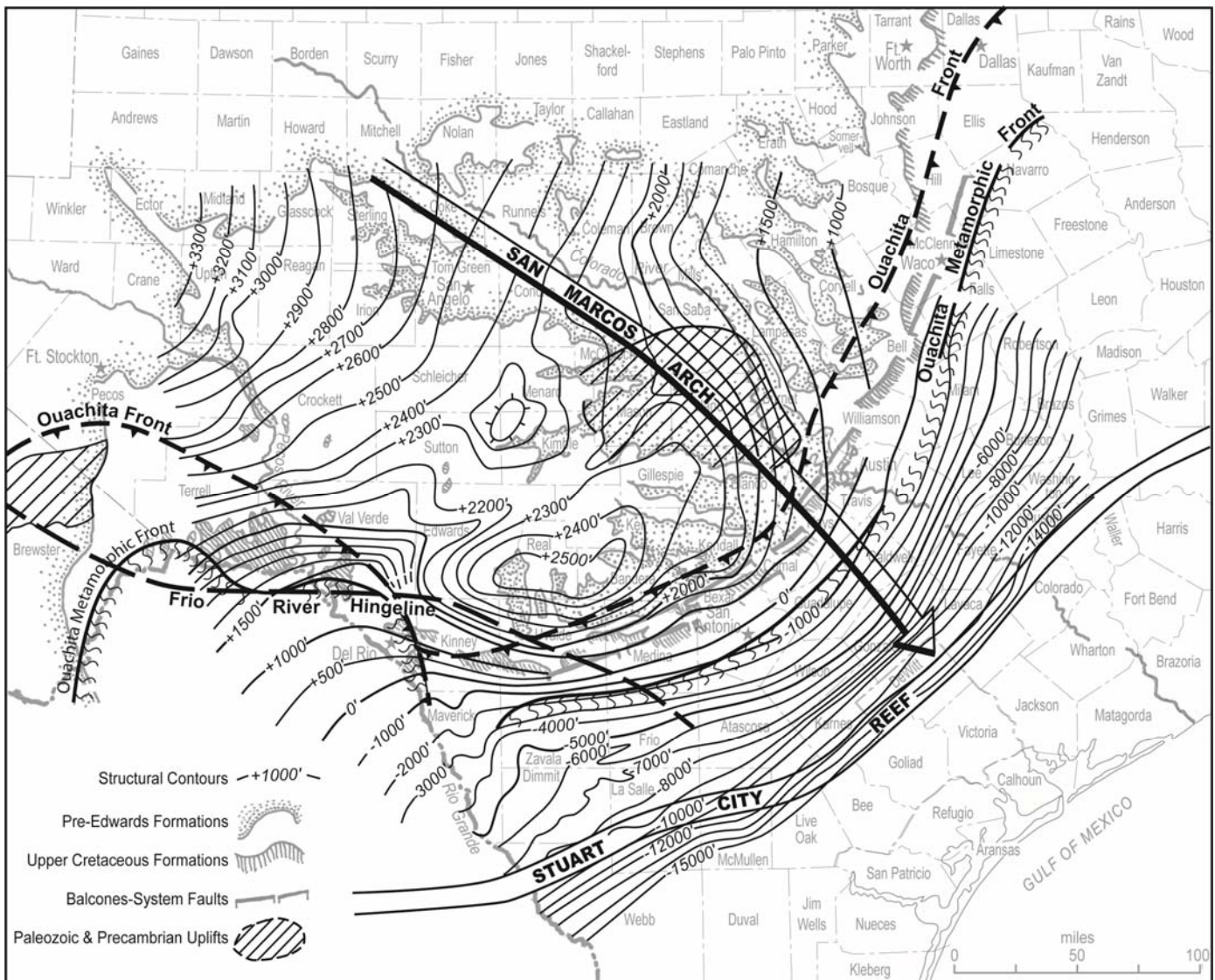
Figure 6. Structure (restored) on top Edwards and equivalents (Lower Cretaceous), Central Texas (from Rose, 1972, 1986a, 1986b, 2004).
