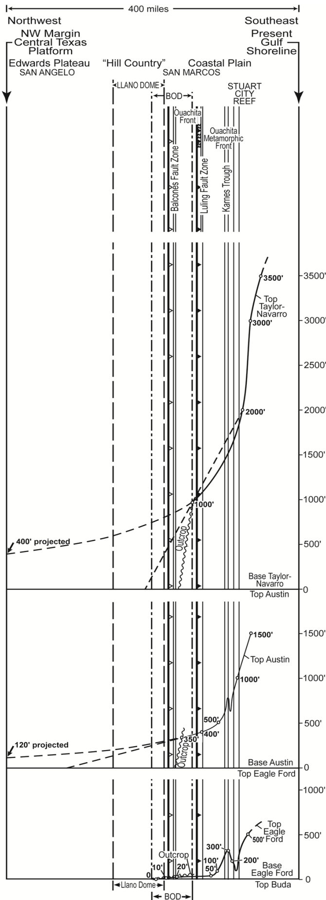
Figure 14. Projected northwest thinning of Upper Cretaceous Formations along San Marcos Arch, from Gulf Coastal Plain across Central Texas Platform.
