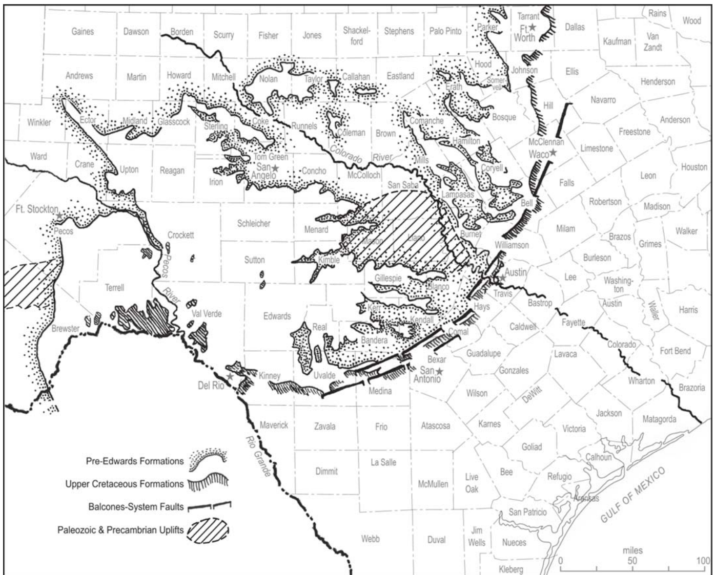
Figure 1. Edwards Plateau, Llano Uplift, Hill Country, Balcones Fault Zone, and Coastal Plain, Central Texas.
