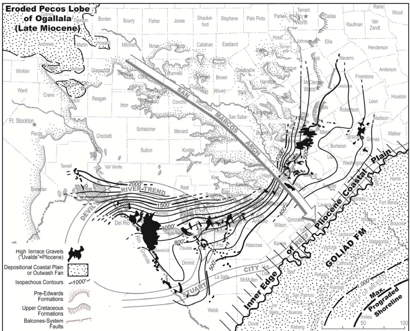
Figure 24. Pliocene isopach and depositional environments, with generalized structure on base of Uvalde Gravel and equivalent high terrace gravels (from Cook and Bally, 1975; Galloway et al., 2011; Texas Bureau of Economic Geology, Geologic Atlas of Texas (Austin [1974], Crystal City–Eagle Pass [1976], Del Rio [1977], Fort Stockton [1982], Laredo [1976], San Antonio [1983], Seguin [1974], Sonora [1981], and Waco [1970] sheets).
