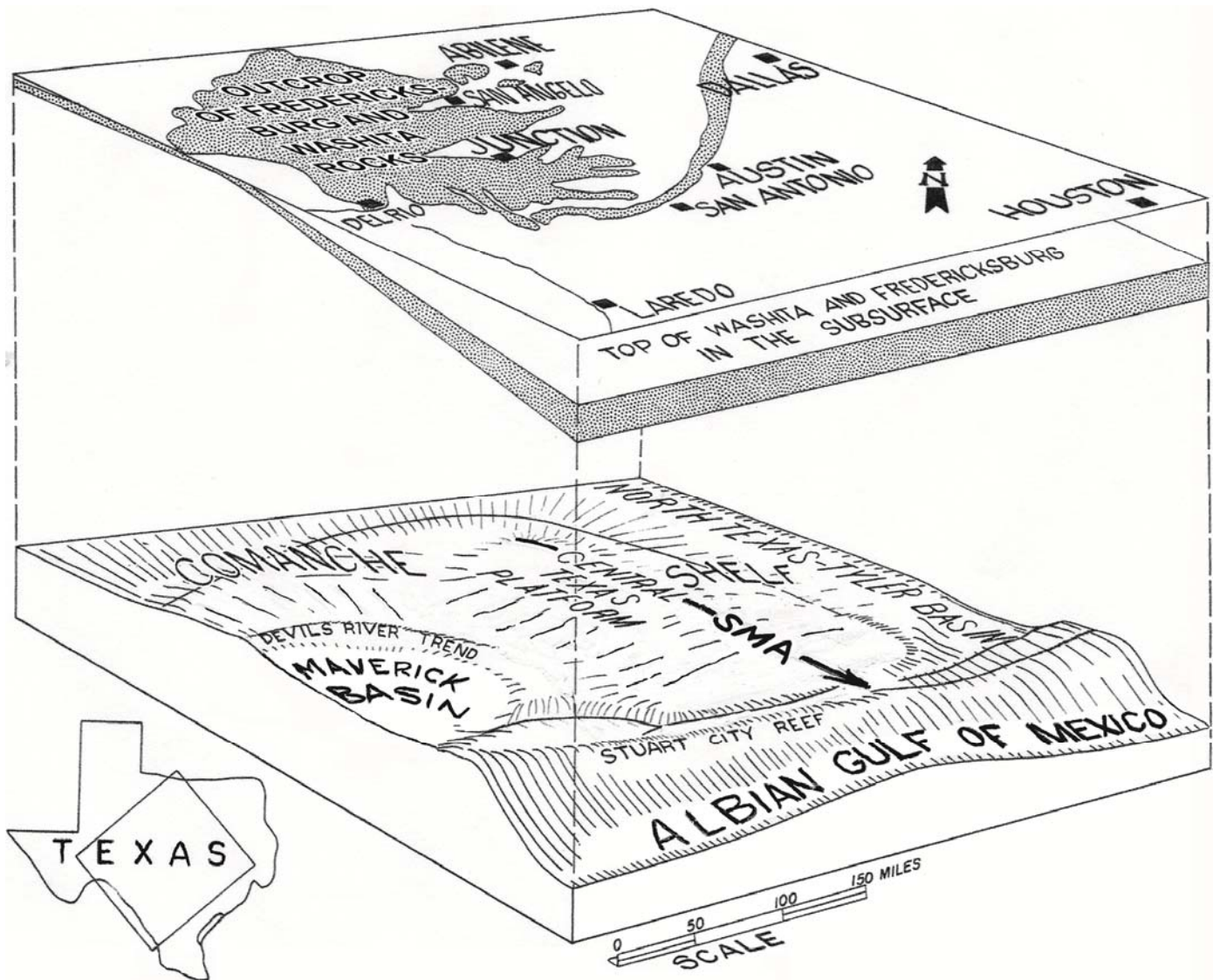
Figure 7. Regional depositional elements, Central Texas, end of Albian (modified after Rose, 1972).
