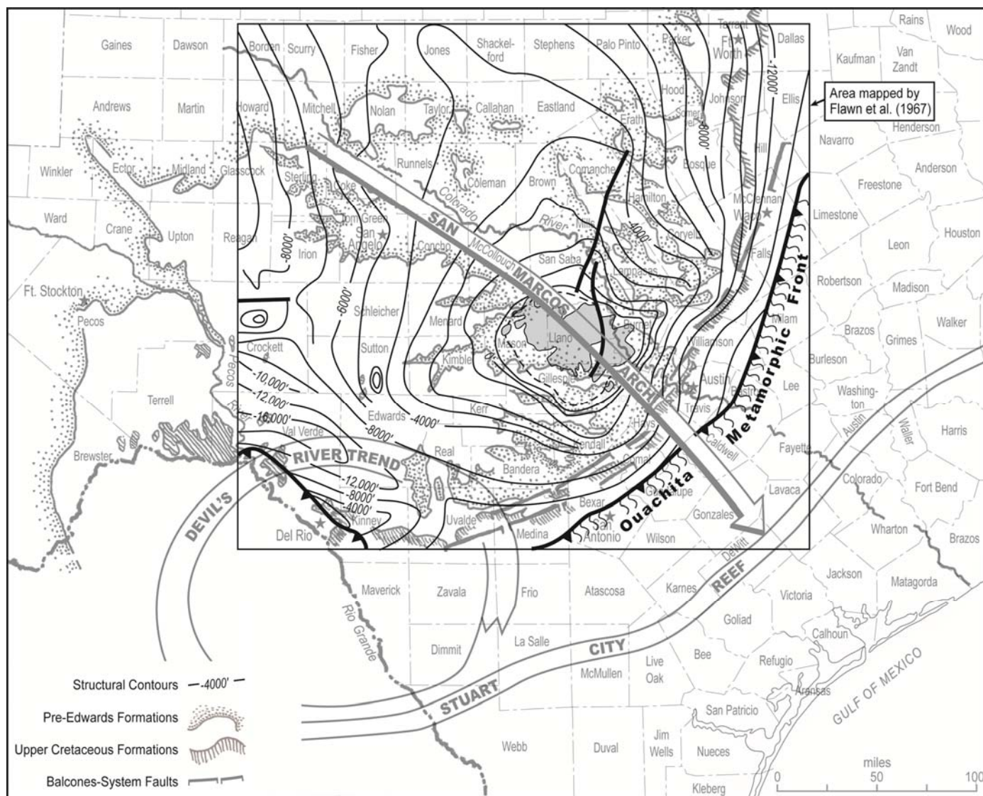
Figure 3. Structure on top Precambrian, Central Texas (after Flawn et al., 1967).
