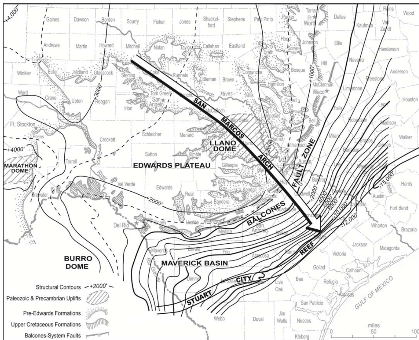
Figure 5. Structure on base Cretaceous (from Ewing, 2005).
