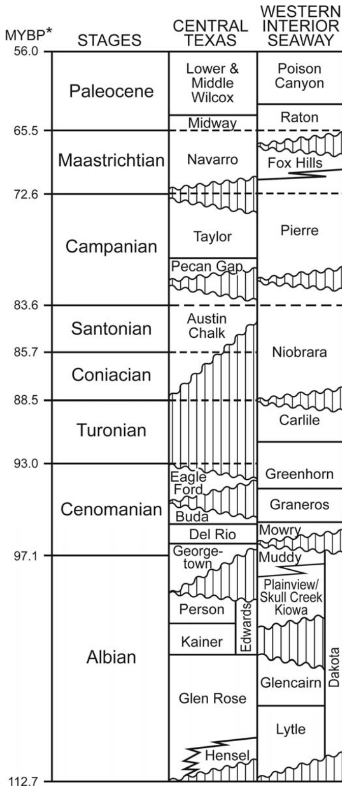
Figure 12. Correlation of Cretaceous successions, Central Texas and Western Interior Seaway (from Rose, 1972; Cook and Bally, 1975; Kauffmann, 1977; Young, 1986; Moore, 1996; Smith et al., 2000; Scott et al., 2003).
