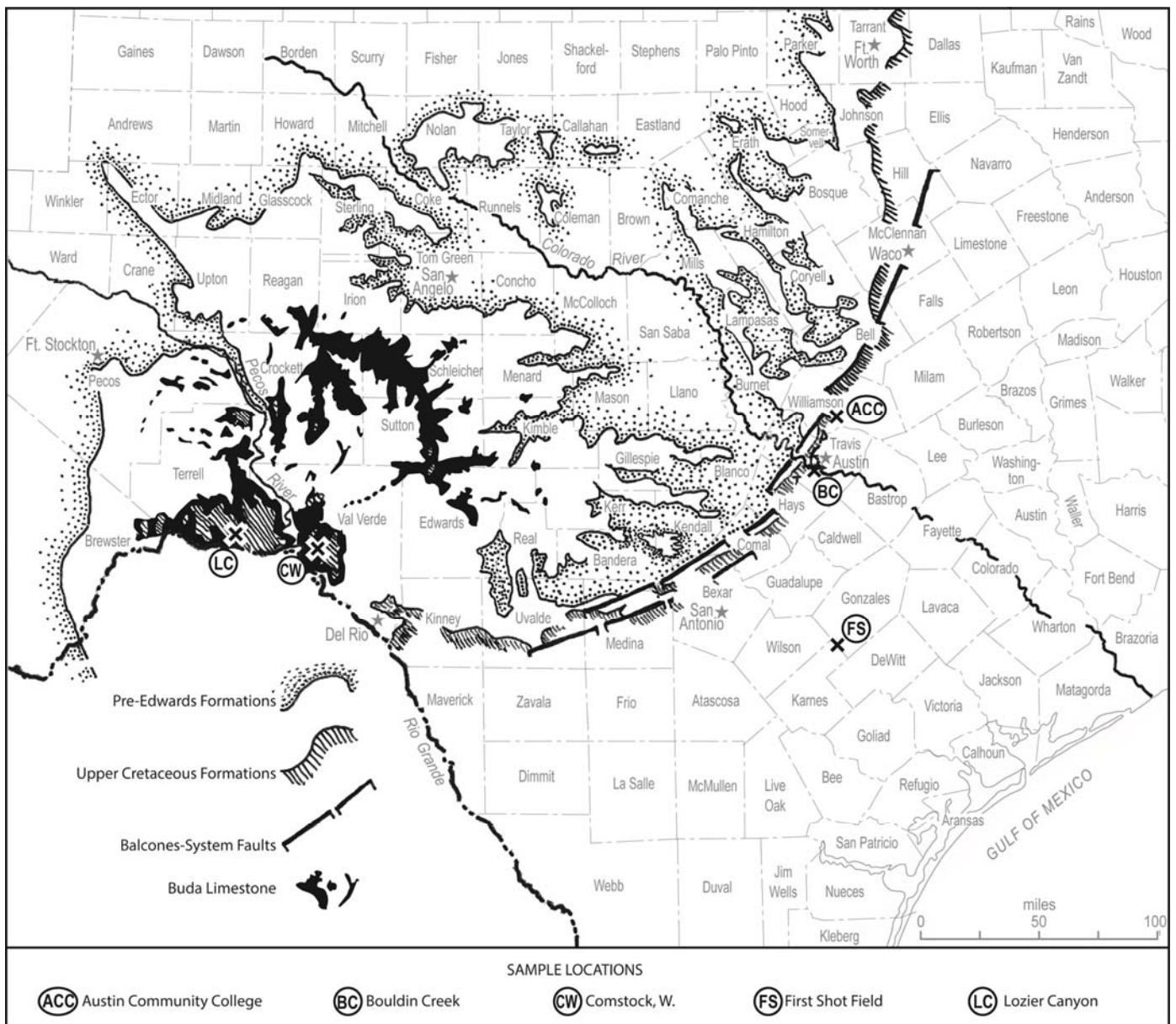
Figure 25. Locations of Eagle Ford and Boquillas samples for depth of burial study; A. Donovan and A. Miceli-Romero, 2014, 2015, personal communication; also Donovan et al., 2012).
