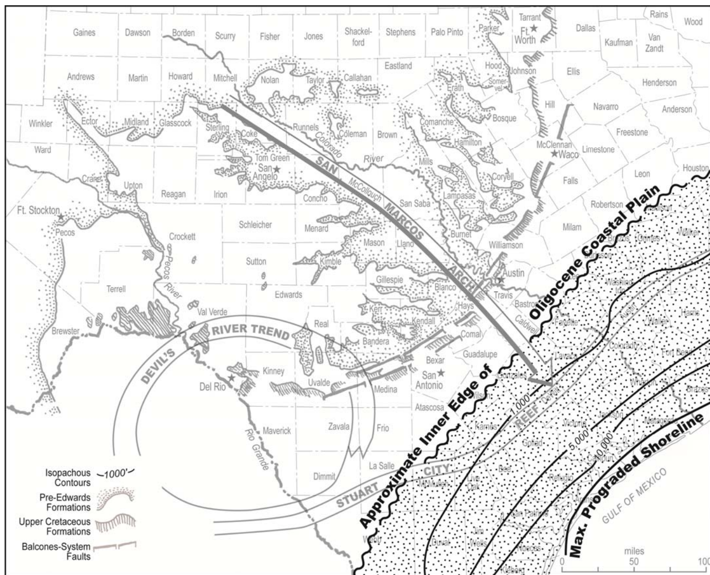
Figure 22. Oligocene isopach and depositional environments (from Cook and Bally, 1975; Galloway et al., 2011).
