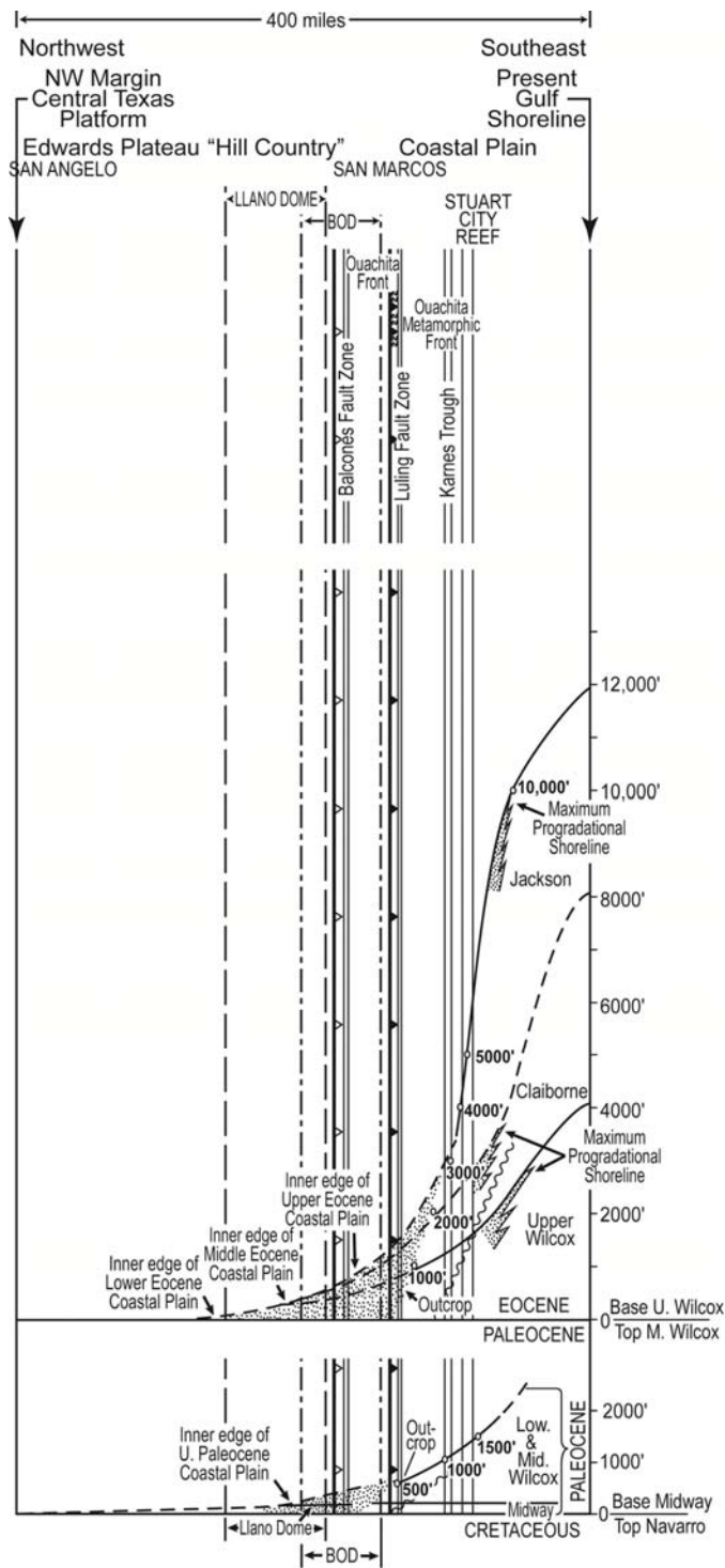
Figure 18. Projected northwest thinning of Paleocene and Eocene formations along San Marcos Arch, from the Gulf Coastal Plain across Central Texas Platform.
