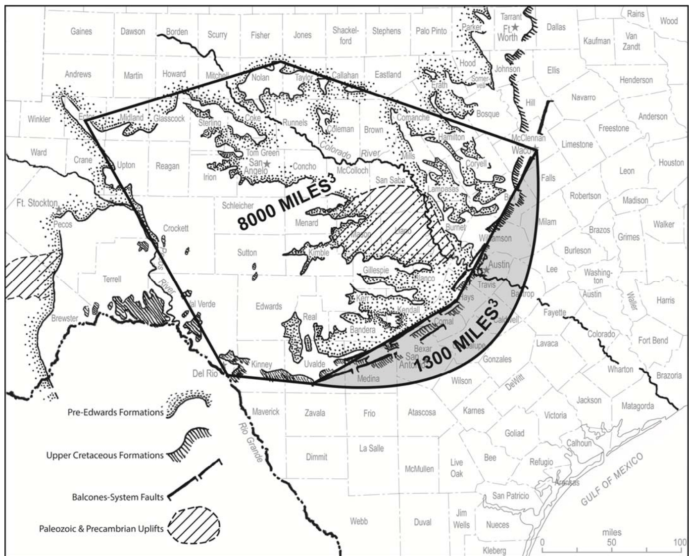
Figure 30. Estimated volumes of rock removed by Tertiary erosion from Edwards Plateau region and Balcones Fault Zone area; shaded area shows arcuate wedge of Upper Cretaceous, Paleocene, and Eocene sediments that were uplifted along gulfward front of the Balcones Fault Zone.
