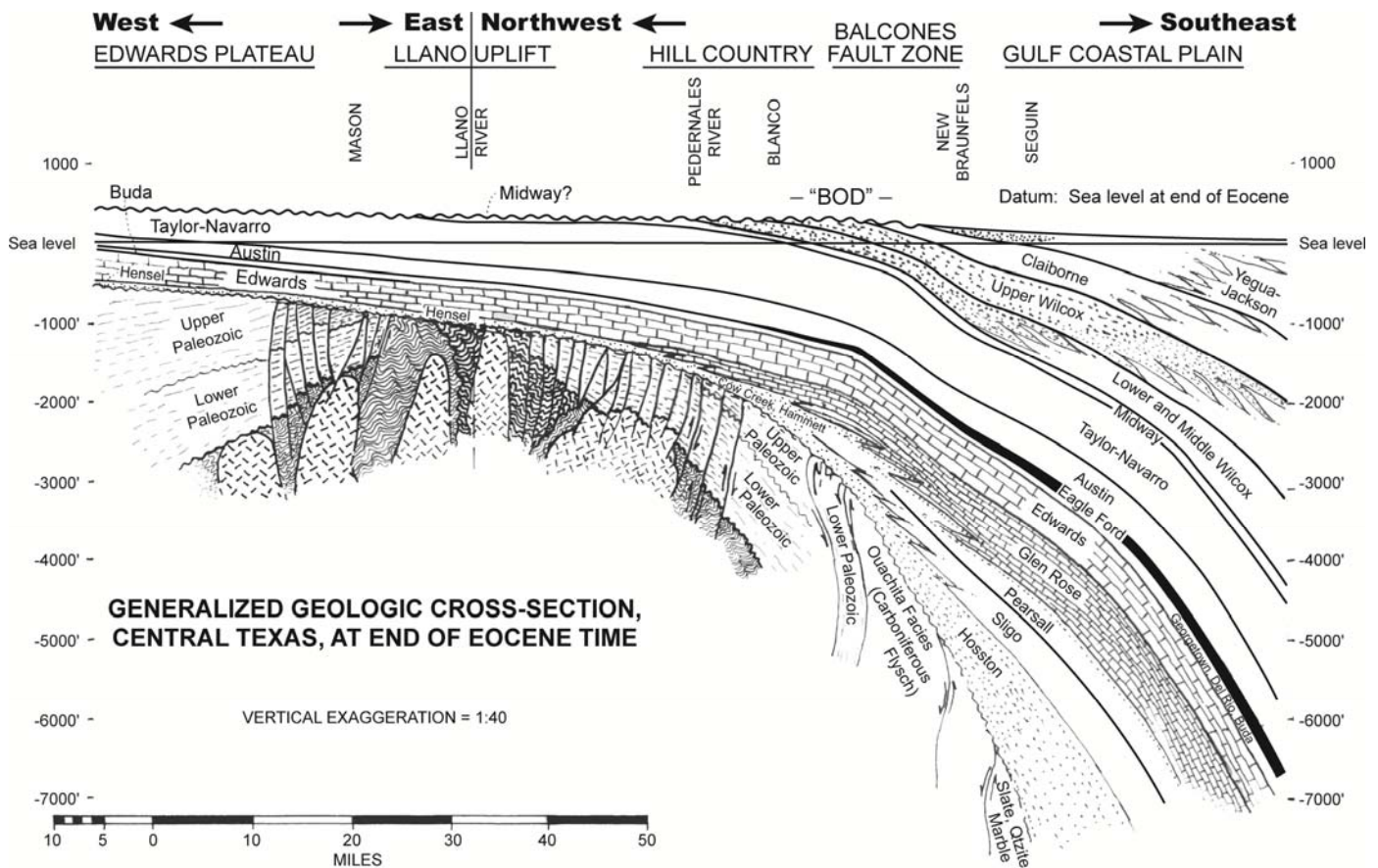
Figure 28. Generalized geologic cross-section, Central Texas, at end of Eocene time; datum = Eocene sea-level.
