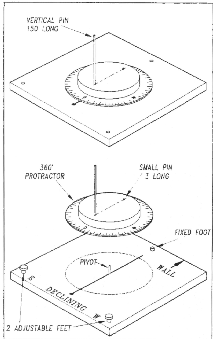
Declination Calculator Dimensions in millimetres
