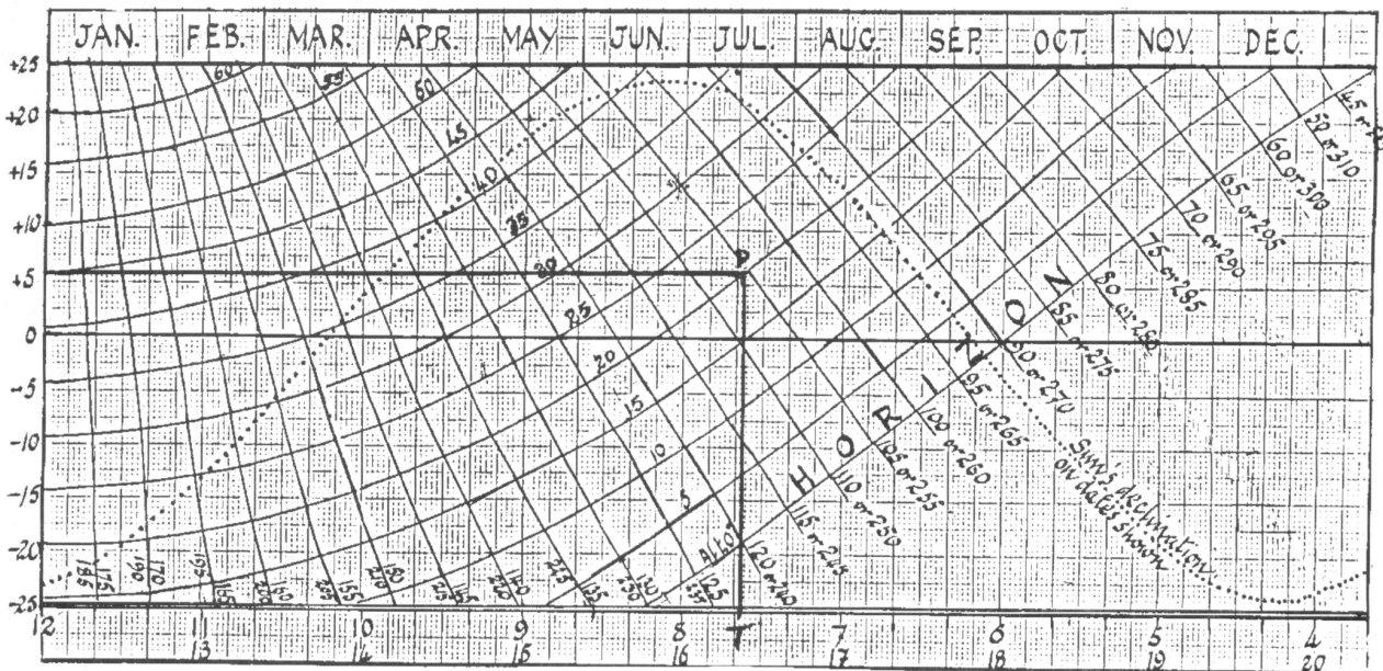
FIGURE 2: A SUN COMPASS AND SUN CLOCK
