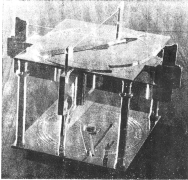
FIGURE 8. An equiangular bifilar sundial designed by M. U. Zakariya and the author. The dial is on the upper plate with hours marked around the circumference. The alidade has a line down its centre and must be turned until the intersection of the shadows of the threads lies on that line. The height and position of the threads are adjusted by micrometers on the underside of the plate, according to the latitude of the dial's location; adjustments for longitude and the equation of time are made with verniers on the dial face. The lower plate gives the equation of time. This dial is the first of a small series of bifilar dials to be constructed by Mr Zakariya.
