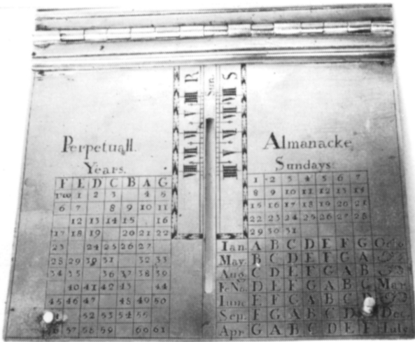
FIGURE 6: Calendar on reverse of Analemmatic Dial.
