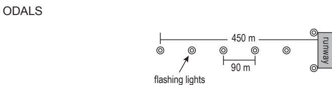
Figure 7.2—ODALS
