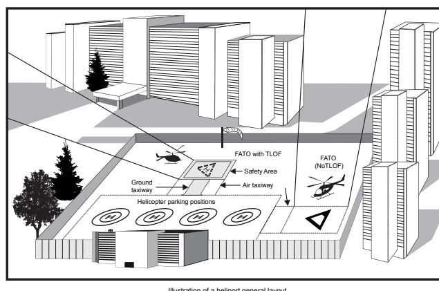
Figure 3.2—Heliport General Layout
