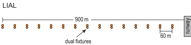
Figure 7.1—LIAL
