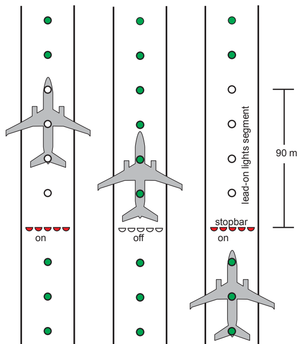
Figure 7.15—Stop Bar Lighting
