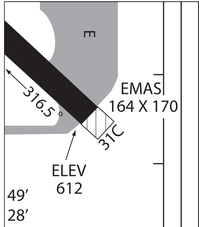
Figure 9.2—EMAS Depiction on an Aerodrome Sketch
