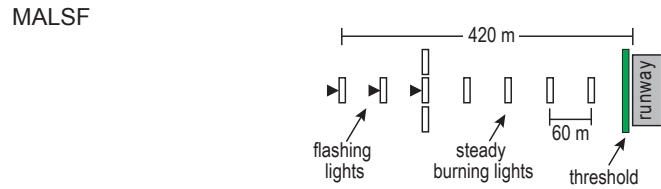
Figure 7.3—MALSF
