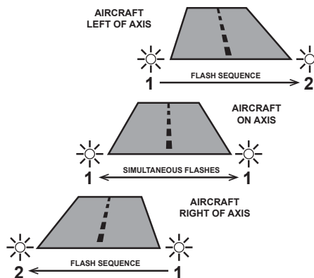
Figure 7.10—VAGS
