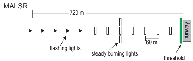
Figure 7.4—MALSR
