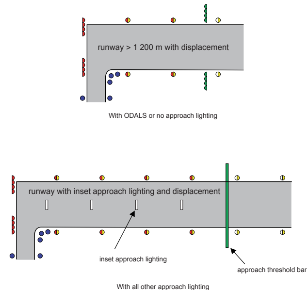
Figure 7.12—Displaced Threshold Lighting
