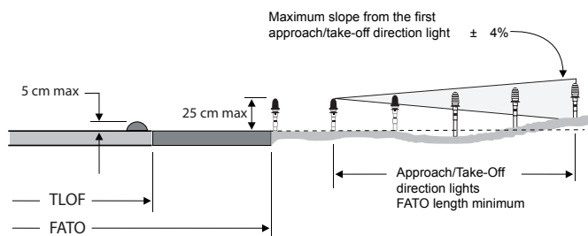
Figure 7.18—Maximum Mounting Height for TLOF, FATO, and Approach/Take-Off Direction Lights
