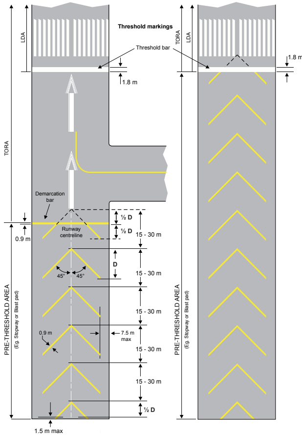
Figure 5.6—Stopway Markings
