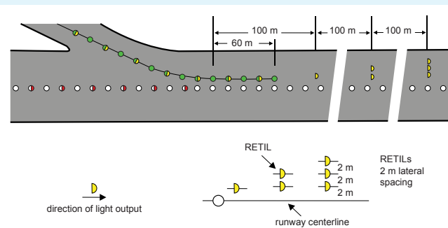
Figure 7.14—Rapid-Exit Taxiway Indicator Lights
