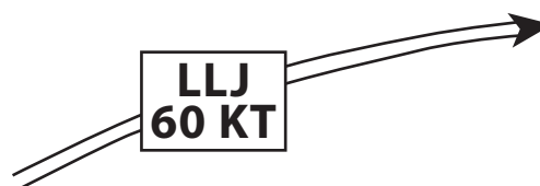
Figure 4.5(h)—LLJ
