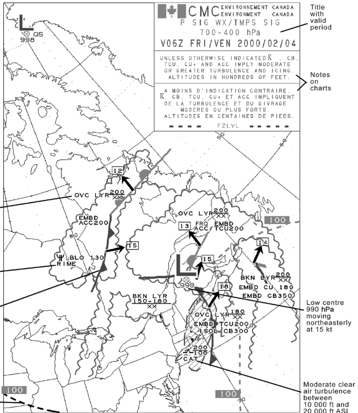
Figure 12.1(a)—Example of a Mid-Level Significant Weather Chart
