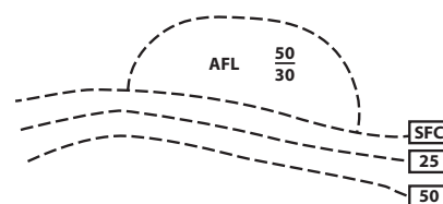
Figure 4.5(g)—Freezing Level
