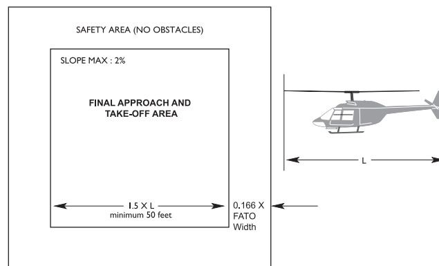
Figure 3.1—FATO/Safety Area
