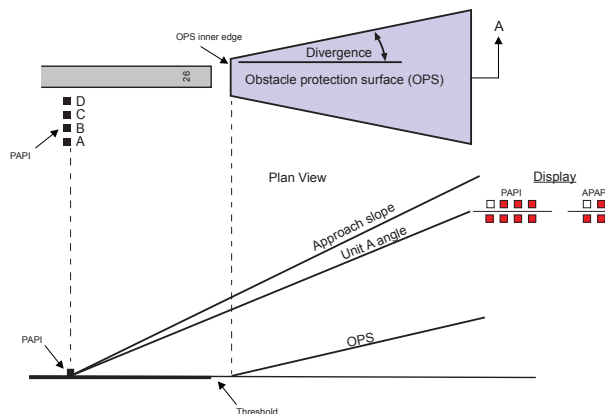
Figure 7.9—PAPI/APAPI OPS
