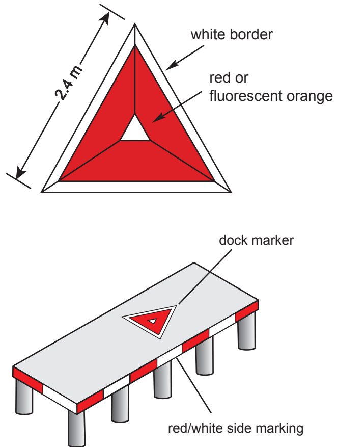
Figure 5.3—Seaplane Dock Markers
