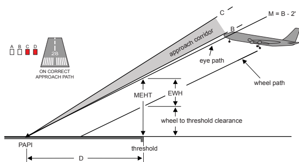
Figure 7.8—PAPI: Pilot Eye Path to Wheel Path
