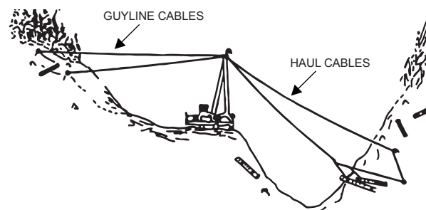
Figure 2.4—Highlead Spar
