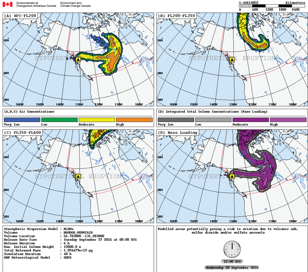
Figure 13.1—Example of Volcanic Ash Forecast Caused by a Hypothetical Eruption
