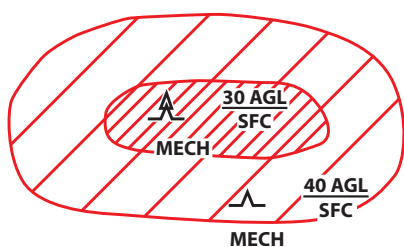
Figure 4.5(e)—Severe and Moderate Turbulence
