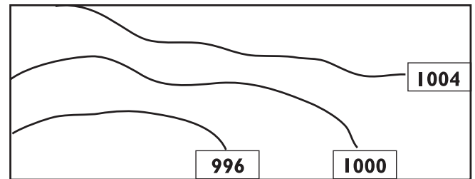
Figure 4.4(g)—Isobars
