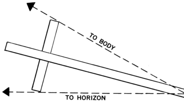
Figure 2808c. Improvised cross-staff.
