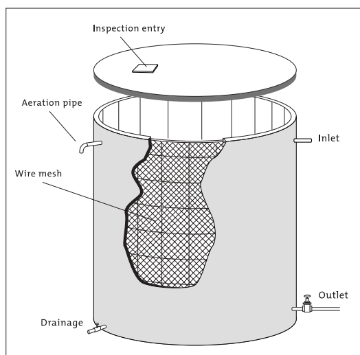
Figure 7.5 Ferrocement tank
