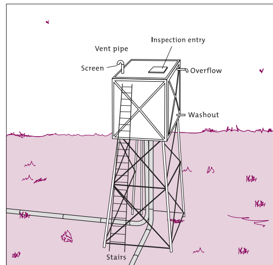
Figure 7.4 Elevated steel reservoir
