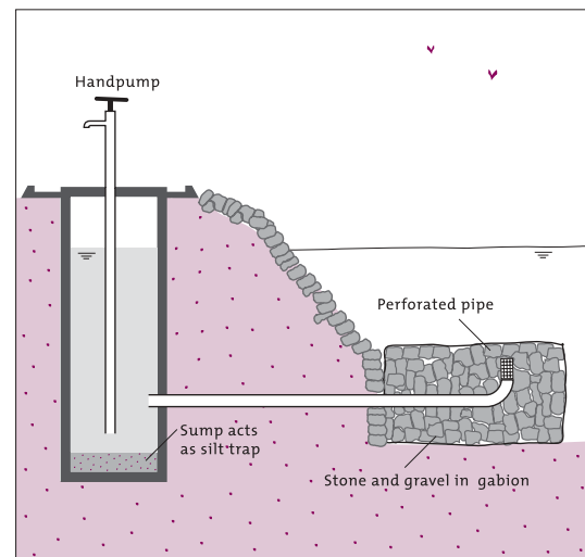
Figure 3.11 Sump intake
