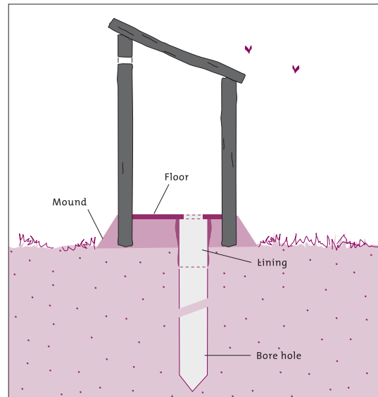
Figure 8.5 Bored-hole latrine
