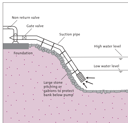
Figure 3.9 River-bottom intake
