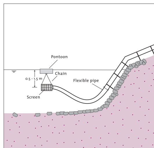
Figure 3.10 Floating intake
