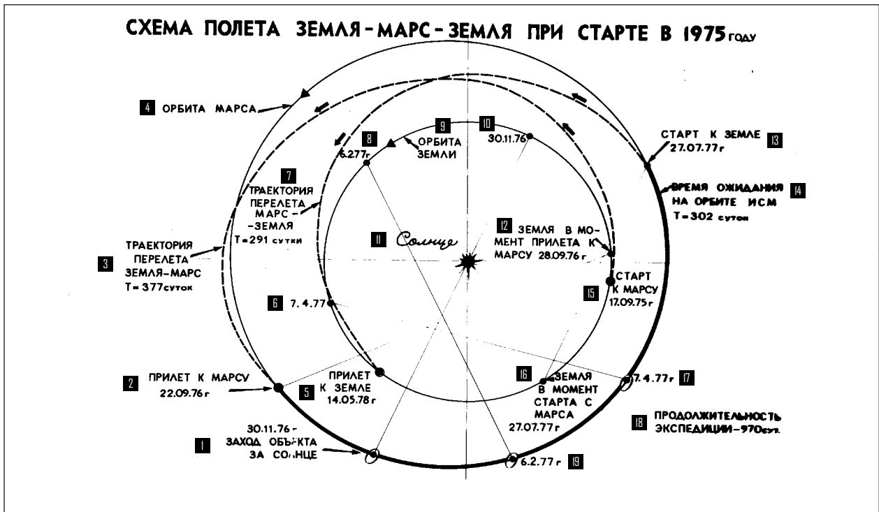
Figure 22. The Profile of an Earth-Mars-Earth Flight If the Spacecraft Would Have Been Landed in 1975—(1) 30.11.76, spacecraft is positioned behind the Sun, (2) 22.09.76, arrival at Mars, (3) interplanetary Earth-Mars trajectory, T=377 days, (4) Martian orbit, (5) 14.05.78, arrival at Earth, (6) 7.4.77, (7) interplanetary Mars-Earth trajectory, T=291 days, (8) 6.2.77, (9) Earth's orbit, (10) 30.11.76, (11) Sun, (12) 28.09.76, Earth's position at the time of the spacecraft arrival at Mars, (13) 27.07.77, spacecraft is launched to Earth, (14) time that the Martian satellite spent in orbit, T=302 days, (15) 17.09.75, launch to Mars, (16) 27.07.77, position of Earth at the time when the spacecraft was launched from Mars, (17) 7.4.77, (18) duration of the expedition—970 days, and (19) 6.2.77
