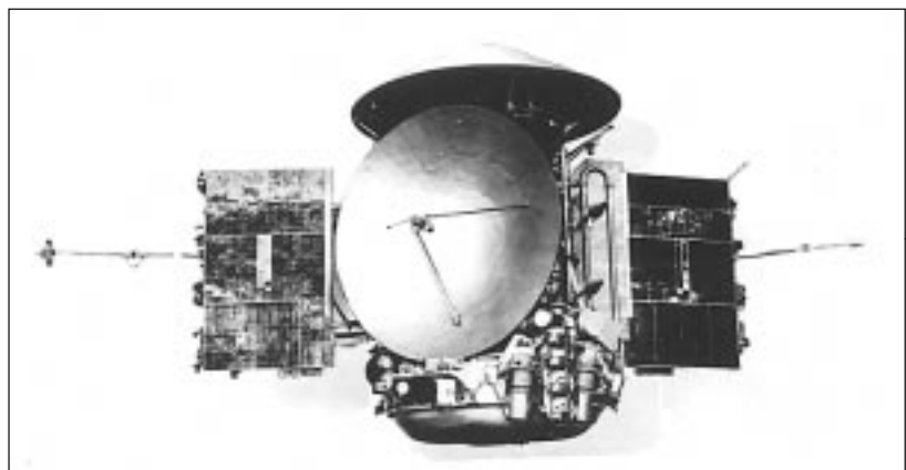
Figure 19. The Mars 6 and 7 Spacecraft
