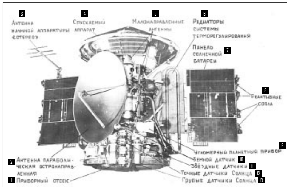
Figure 14. The Mars 3 Spacecraft— (1) instrument module, (2) high-gain parabolic antenna, (3) stereo anten- na of the scientific instru- ments, (4) lander, (5) low-gain antennas, (6) radiators of the tem- perature control system, (7) solar panel, (8) reac- tive nozzles, (9) device for planetary angle measure- ments, (10) Earth sensor, (11) star sensor, (12) precise solar sensor, and (13) rough solar sensor
