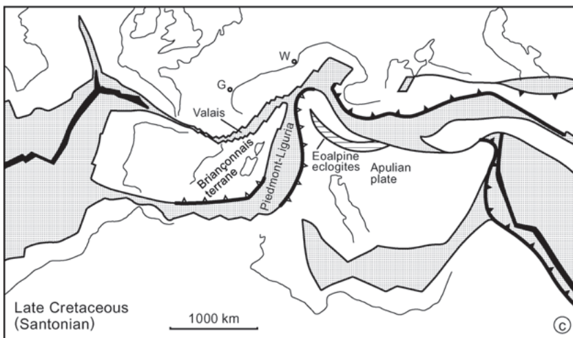
Fig. 2. Large-scale paleogeographical reconstruction for a) Late Triassic, b) Late Jurassic and c) Late Cretaceous times. G: Genève; W: Wien. After Frank 1987, Stampfli 1993, Schmid et al. 1997 and Stampfli et al. 2001.
