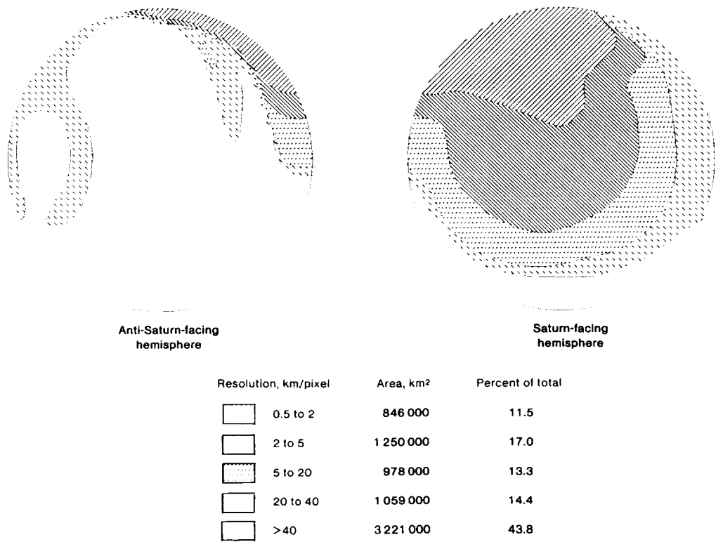
Figure 5-1. Resolution of Voyager pictures of Rhea in terms of aerial coverage.
