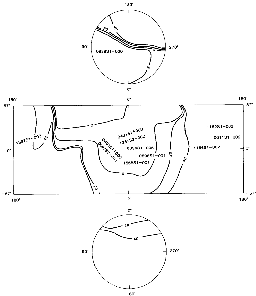
Figure 5-2. Index of Voyager 1 and 2 pictures used to compile the maps of Rhea. Picture numbers indicate the subspacraft point at the time the pictures were taken. Contour lines indicate the approximate resolution of available images in kilometers per picture element. (See also fig. 5-1.)
