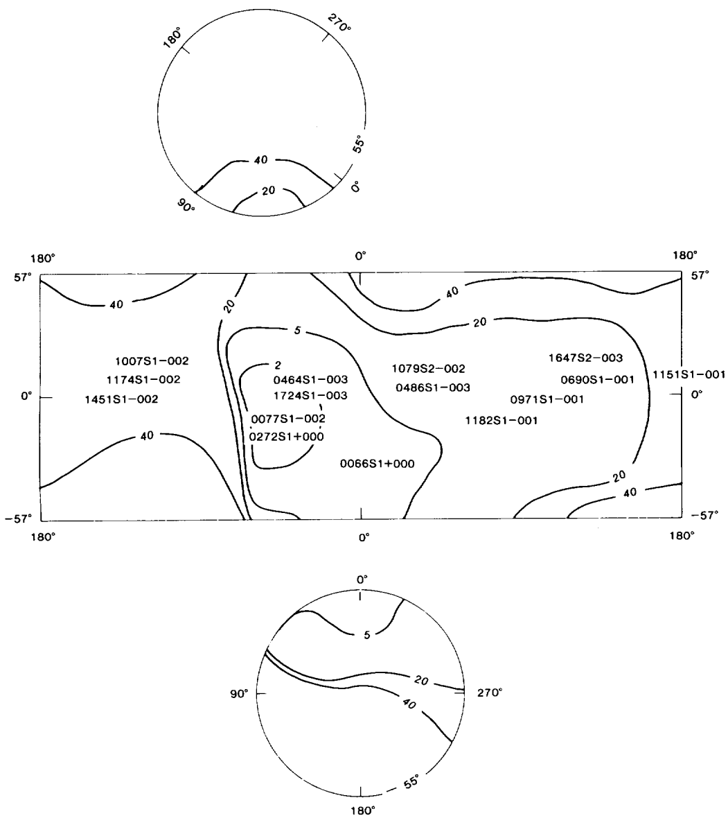
Figure 4-2. Index of Voyager 1 and 2 pictures used to compile the maps of Dione. Picture numbers indicate the subspacecraft point at the time the pictures were taken. Contour lines indicate the approximate resolution of available images in kilometers per picture element. (See also fig. 4-1.)
