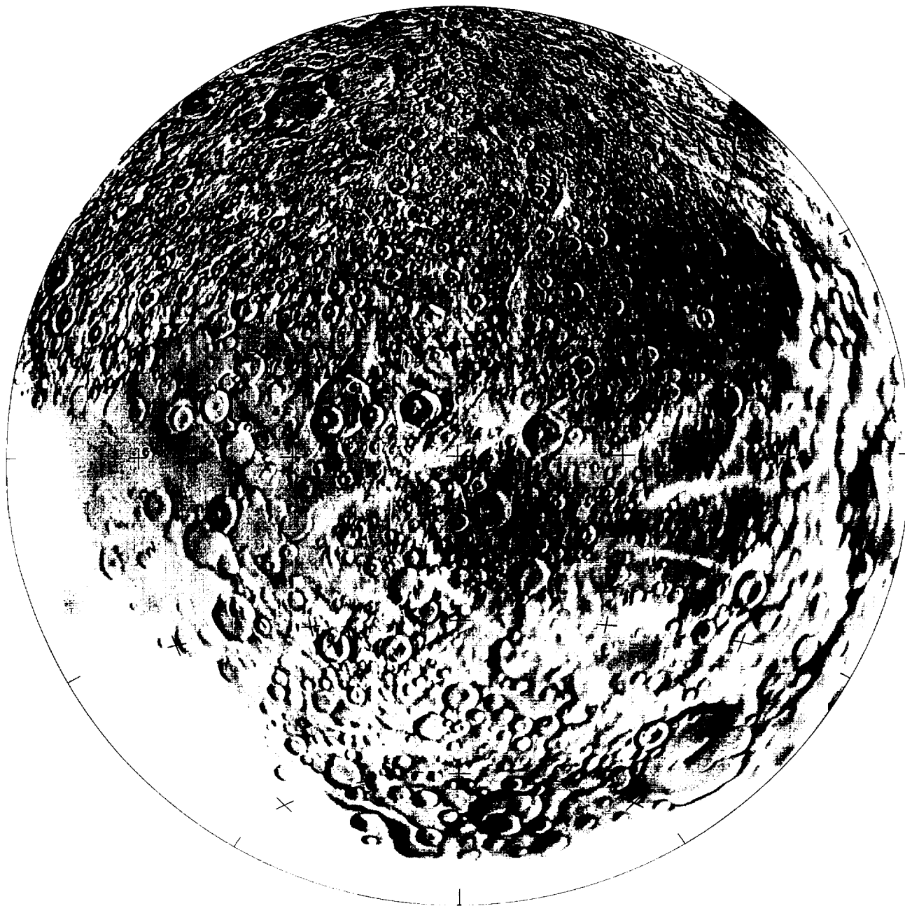
Figure 5-7. Map of the Saturn-facing hemisphere of Rhea on a Lambert azimuthal equal-area projection. Nomenclature is not shown, to avoid obscuring detail. Scale 1:10 000 000 (1 mm 2 = 100 km 2 ; 1 in 2 = ~25 000 mi 2 ).
