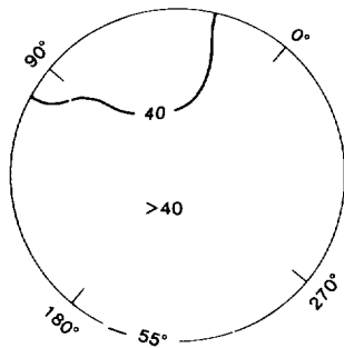
Figure 3-2. Index of Voyager 1 and 2 pictures used to compile the maps of Tethys. Picture numbers indicate the subspacescraft point at the time the pictures were taken. Contour lines indicate the approximate resolution of available images in kilometers per picture element. (See also fig. 3-1.)
