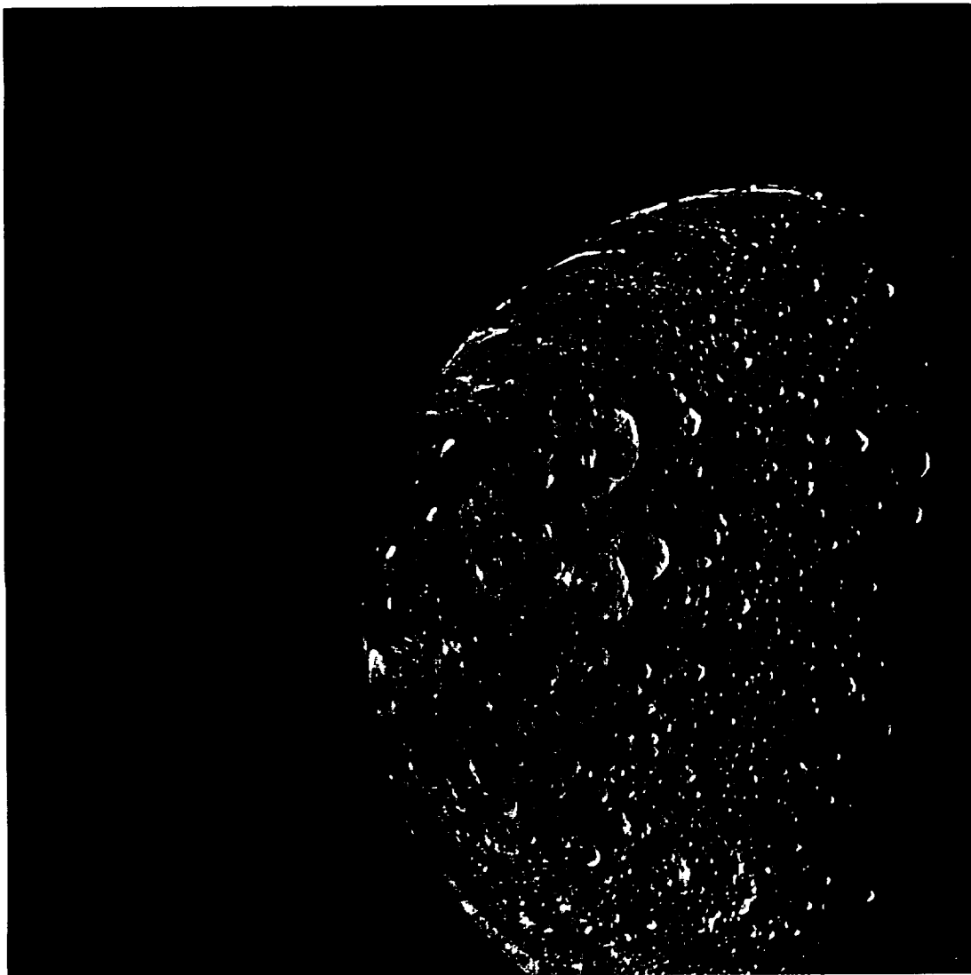
Figure C-8. High-pass-filtered version of figure C-5. A 101-X-101-pixel filter (300 X 300 km on Dione) was used on this image, thus subduing tonal variations covering areas larger than 300 X 300 km. Note also that midtones are uniform across the image, even near the terminator where the unfiltered image of figure C-5 is much darker.
