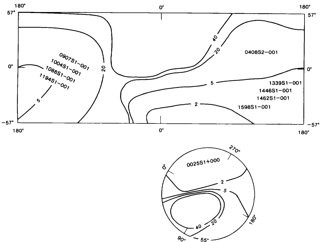
Figure 1-2. Index of Voyager 1 and 2 pictures used to compile the maps of Mimas. Picture numbers indicate the subspacecraft point at the time the pictures were taken. Contour lines indicate the approximate resolution of available images in kilometers per picture element. (See also fig. 1-1.)
