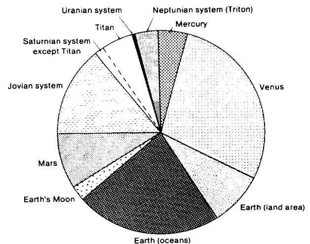
Figure 2. The total known mappable area in the solar system ( \approx 1.6 \times 10^6 \text{ km}^2 ). Planets that may not have solid (mappable) surfaces (Jupiter, Saturn, Uranus, and Neptune) are not included. Pluto and its satellite, Charon, would add only a minuscule amount to this diagram.
