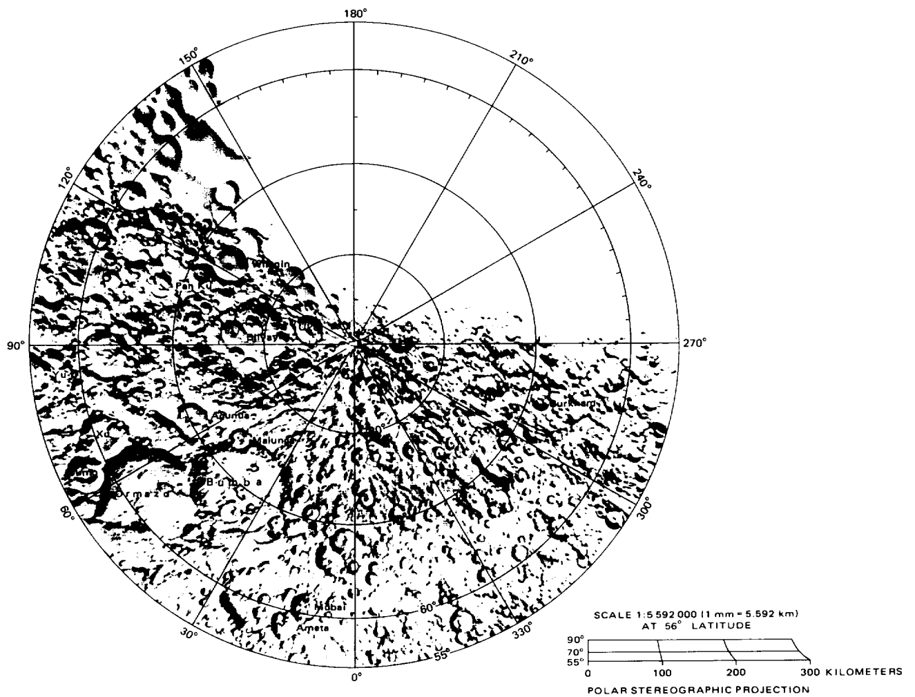
Figure 5-4. Map of the north polar regions of Rhea on a polar stereographic projection (part of map I-1484).
