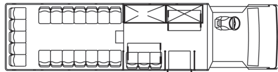
19 Passengers with 2 Wheelchairs or 22 Passengers
