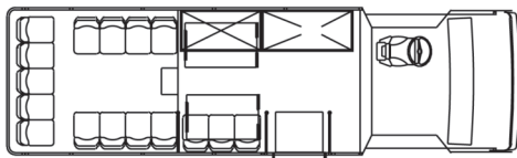
13 Passengers with 2 Wheelchairs or 16 Passengers
