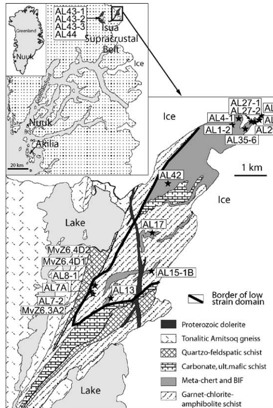
Fig. 1. Simplified geologic map (after Appel et al., 1998) of the eastern part of the Isua Supracrustal Belt in southern West Greenland. Most of the samples were collected from the ‘low-strain zone’ in the northeastern part of the ISB including metacarbonates (AL17, AL7-2, AL8-1, AL7A, MvZ6.3A2, MvZ6.4D1, MvZ6.4D2), BIFs (AL4-1, AL27-1, AL27-2, AL13, AL35-6, AL15-1B), metacherts (AL25, AL26, AL42) and mafic dykes (AL1-2, AL29-1). Three samples from a metasedimentary turbidite sequence (AL43-1, AL43-2, AL43-3) as well as a metacarbonate sample (AL44) from the western part of the belt were also studied. Metacarbonate sample AL7-2 was subdivided into a magnetite-rich band (AL7-2M) and a carbonate-rich band (AL7-2C). Sample AL17 represents heavily metasomatized chert. Subsamples from both carbonate dominated (AL17C) and chert dominated (AL17Chert) bands were analyzed.
