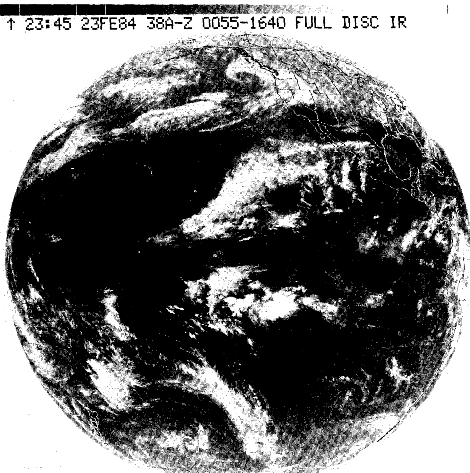
FIG. 1. Full disc IR picture at 2345 GMT 23 February 1984.
