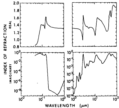
FIG. 10. Real and imaginary parts of the refractive index of ice in solar and thermal infrared wavelengths. (After Warren, 1984 with modifications.)
