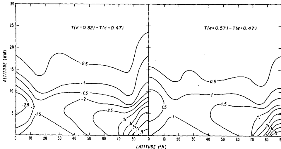
FIG. 19. The latitude–height distribution of temperature changes caused by a decrease (left) and increase (right) of the cirrus IR emissivity.
