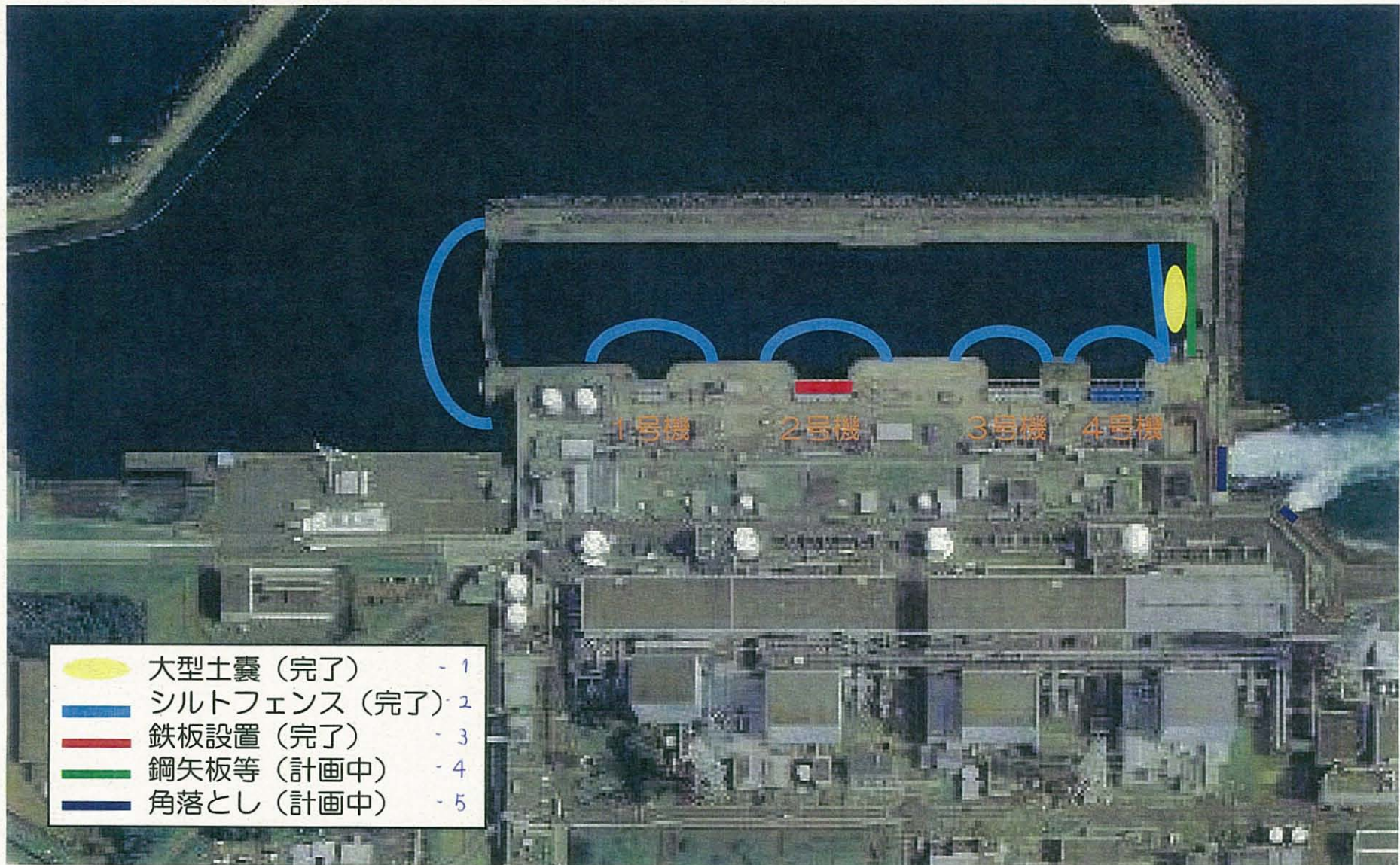
1. Large-sized sandbags. 2. Silt fence. 3. Steel plate insulation. 4. Sheet Pile. 5. Sliding timber Weir
