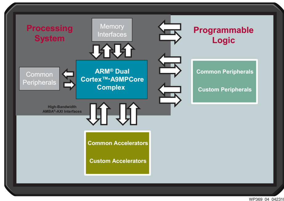
Figure 4: Extensible Processing Platform
