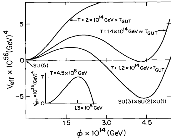
FIG. 1. Effective potential vs \varphi for various values of T .
