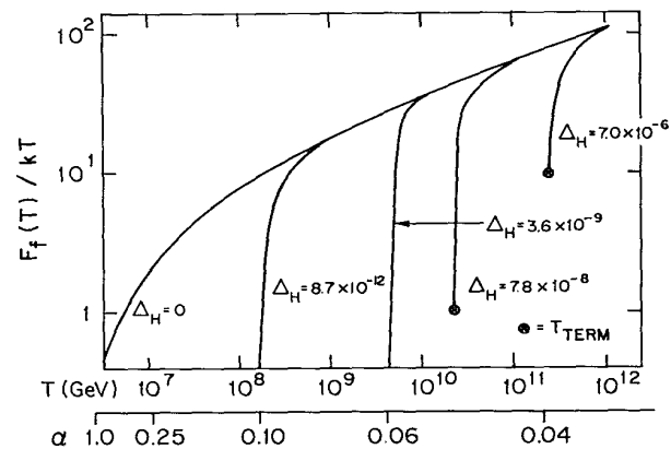
FIG. 2. F_f(T)/kT vs T . Curves terminate for p(T) \approx 1 . \Delta_H = (M_H^2 - M_{\text{CW}}^2)/M_{\text{CW}}^2 .
