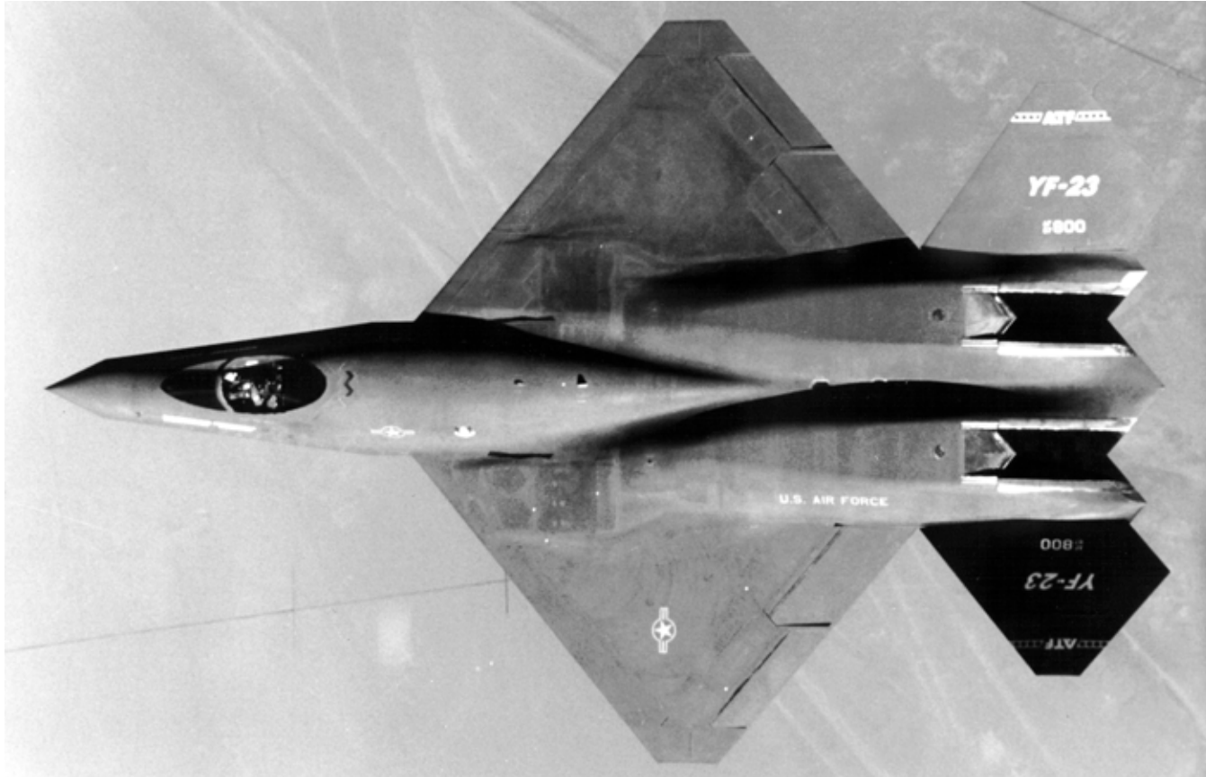
Photo 6.4—The Northrop/McDonnell-Douglas YF-23 flew in a three-month comparative test program with the YF-22 in early 1991. That April, the U.S. Air Force selected the YF-22 for full-scale development.
