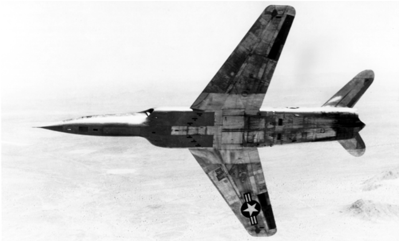
Photo 2.13—The Lockheed XF-90 long-range fighter prototype competed against the McDonnell XF-88 and North American XF-93 during flight tests undertaken in 1950. Although the Air Force considered all three to be inadequate, McDonnell was encouraged to develop the XF-88 further, which eventually evolved into the F-101 Voodoo.
