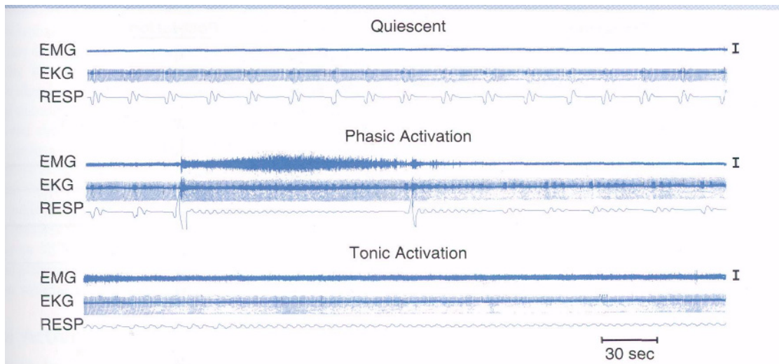
Figure 10-3. States seen in the chronic medullary cat. Note the absence of periods of atonia. EKG, electrocardiogram; EMG, electromyogram; RESP, thoracic strain gauge. Calibration 50 \mu V. (From Siegel JM, Tomaszewski KS, Nienhuis R: Behavioral states in the chronic medullary and mid-pontine cat. Electroencephalogr Clin Neurophysiol 1986;63:274-288, with permission.)
