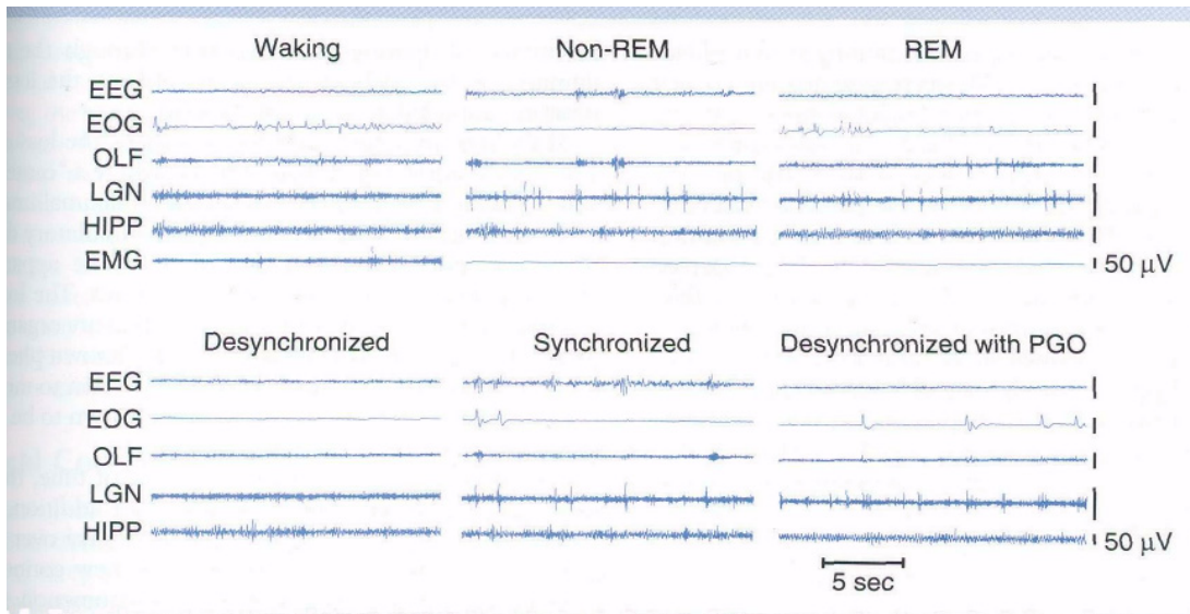
Figure 10-1. Top, Polygraph tracings of states seen in the intact cat. Bottom, States seen in the forebrain 4 days after transection at the pontomedullary junction. EEG, sensorimotor electroencephalogram; EOG, electrooculogram; OLF, olfactory bulb; LGN, lateral geniculate nucleus; HIPP, hippocampus; EMG, dorsal neck electromyogram. (From Siegel JM, Nienhuis R, Tomaszewski KS: REM sleep signs rostral to chronic transections at the pontomedullary junction. Neurosci Lett 1984;45:241-246, with permission.)
