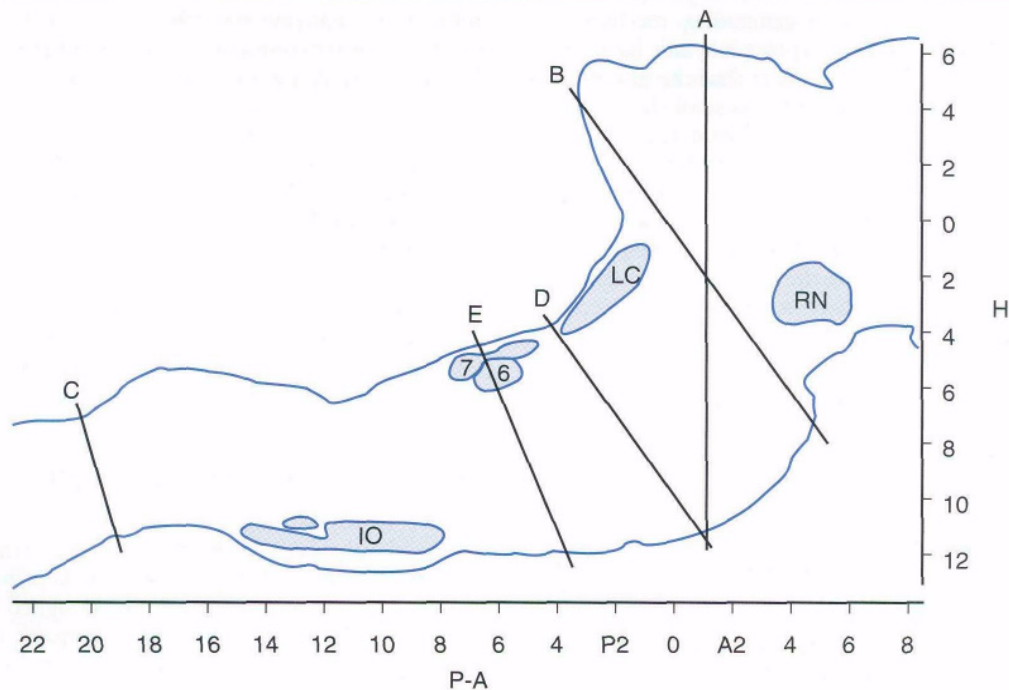
Figure 10-2. Outline of a sagittal section of the brainstem of the cat drawn from level L = 1.6 of the Berman atlas, indicating the level of key brainstem transection studies. A and B, midbrain-pontine junction; D, caudal pons; E, ponto-medullary junction; C, spino-medullary junction; RN, red nucleus; LC, locus coeruleus; 6, abducens nucleus; 7, genu of the facial nerve; IO, inferior olive. H (horizontal) and P-A (posterior-anterior) scales are drawn from the atlas. (From Siegel JM: Pontomedullary interactions in the generation of REM sleep, in McGinty DJ, Drucker-Colin R, Morrison A, Parmeggiani PL [eds]: Brain Mechanisms of Sleep . New York, Raven Press, 1985, pp 157-174, with permission.)
