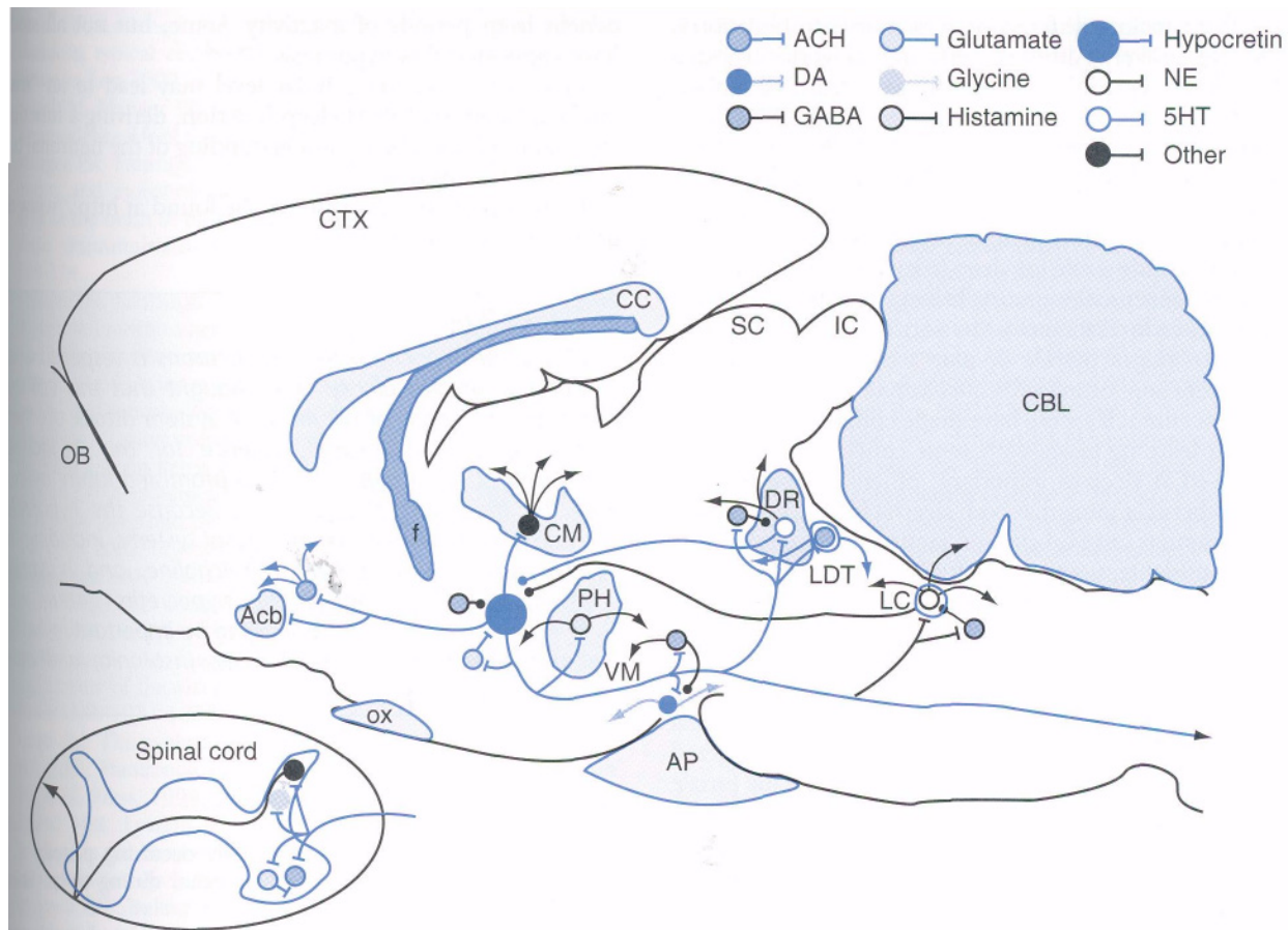
figure 10-10. Major identified synaptic interactions of hypocretin (Hcrt) neurons. Lines terminated by perpendicular lines denote excitation; <math>\langle r terminations </math> indicate inhibition. Arrows indicate direction of projections. CC, corpus callosum; CTX, cortex; 5HT, serotonin; Acb, nucleus accumbens; ACH, acetylcholine; AP, anterior pituitary; CBL, cerebellum; CM, centromedian nucleus of the thalamus; DA, dopamine; DR, dorsal raphe nucleus; f, fornix; IC, inferior colliculus; LC, locus coeruleus; LDT, laterodorsal tegmentum and Pedunculo-pontine; NE, norepinephrine; OB, olfactory bulb; ox, optic chiasm; PH, posterior hypothalamus; SC, superior colliculus; VM, ventral midbrain. (From color figure in Siegel JM, Ann Rev Psychol 55:125-148, with permission.)
