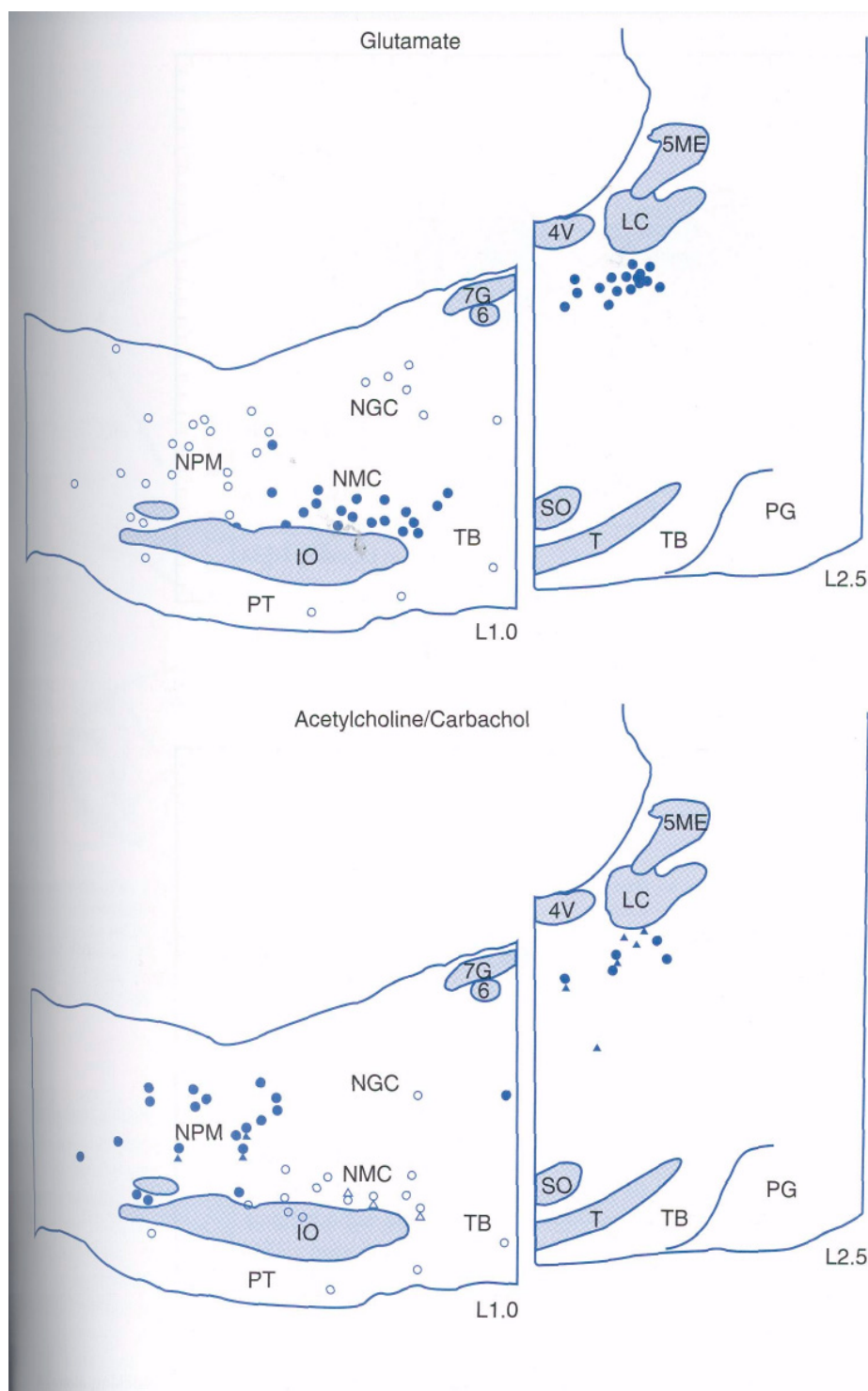
Figure 10-8. Sagittal map of pontomedullary inhibitory areas. Electrical stimulation produced atonia at all the points mapped. All electrically defined inhibitory sites were microinjected with glutamate or cholinergic agonists. Filled symbols represent points at which microinjections decreased muscle tone (to less than 30% of baseline values or to complete atonia). Open circles indicate points at which injections increased or produced no change in baseline values. Glutamate injections are shown at the top, acetylcholine (ACh) and carbachol (Carb) injections at the bottom. At the bottom, circles and triangles represent ACh and Carb injections, respectively. 4V, fourth ventricle; 5ME, mesencephalic trigeminal tract; 6, abducens nucleus; 7G, genu of the facial nerve; IO, inferior olivary nucleus; LC, locus coeruleus nucleus; NGC, nucleus gigantocellularis; NMC, nucleus magnocellularis; NPM, nucleus paramedianus; PG, pontine gray; PT, pyramidal tract; SO, superior olivary nucleus; T, nucleus of the trapezoid body; TB, trapezoid body. (From Lai YY, Siegel JM: Medullary regions mediating atonia. J Neurosci 1988;8: 4790-4796, with permission.)
