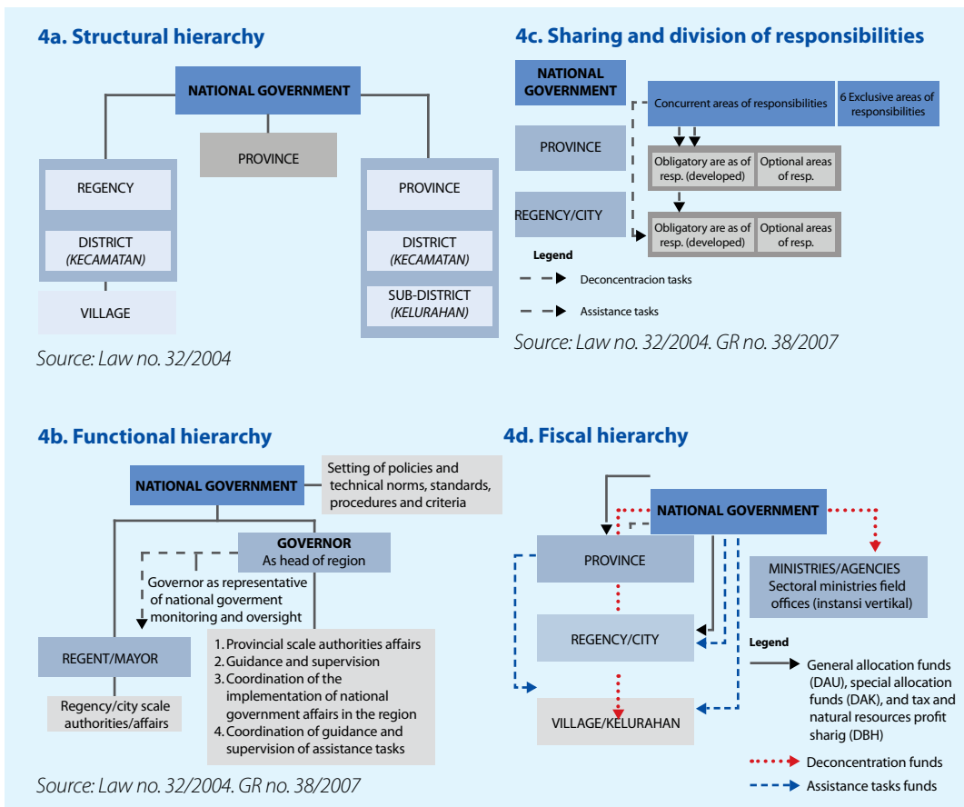
Figure 4.1.: Multiple hierarchies
