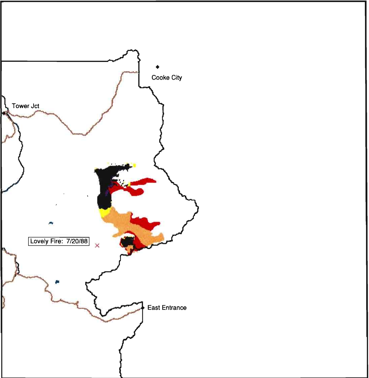
Clover-Mist Fire Growth for week ending July 23, 1988 0 5 10 15 20 25 miles 40.2 km (February 1993)
