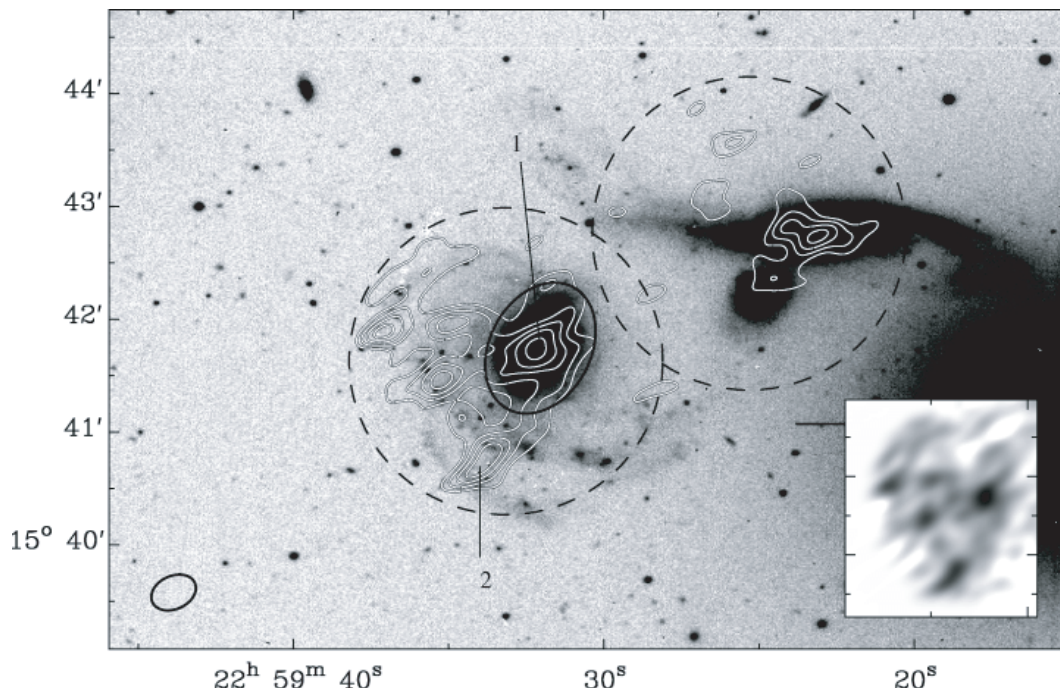
FIG 4.7.— SCUBA 850\ \mu\text{m} maps of NGC7465, overlaid on the greyscale B-band image. Dashed circles indicate the SCUBA field of view, while the solid ellipse indicates the B = 25\ \text{mag arcsec}^{-2} isophotal size. The dust emission extends considerably beyond this isophote (Thomas et al. 2002). The inset is the SCUBA image in greyscale.
