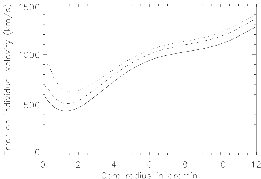
FIG 3.11.—The total rms error in individual cluster velocities, including all contributions (primary CMB, background kinetic SZ, residuals from component separation, Planck -like instrumental noise). The solid, dotted, and dashed lines represent SCDM, OCDM and \Lambda CDM models, respectively (Aghanim, Górski, and Puget 2001)
