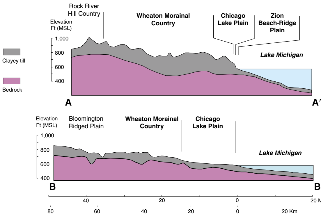
The thickness of glacial sediment is generally greatest in the northern part of Chicagoland (after Willman 1971, Herzog et al. 1994).
