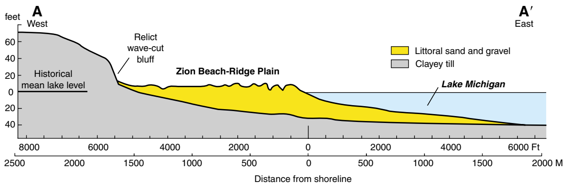
Generalized cross section showing the beach ridge sediments overlying a relict nearshore profile eroded in till (modified from Chrzastowski and Trask 1995).
