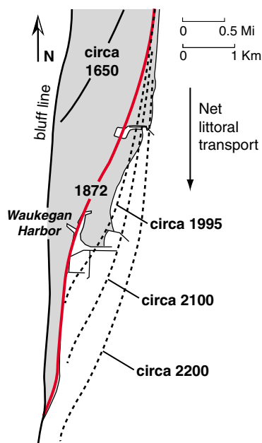
Projected shoreline change if Waukegan Harbor had not been built (modified from Chrzastowski and Trask 1995).
