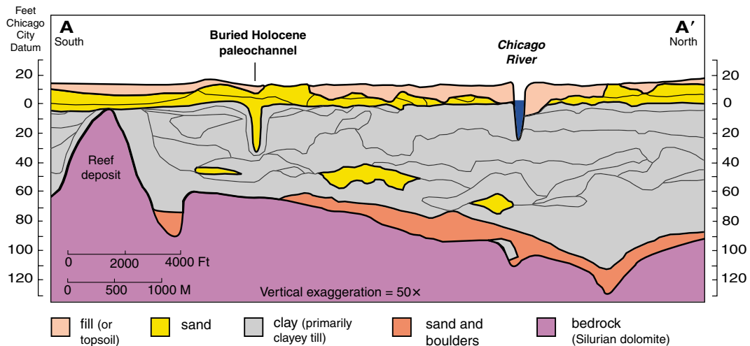
The Chicago Loop is underlain by fill, lacustrine sand, and a thick sequence of glacial clay over basal sand and boulders (cross section modified from Peck and Reed 1954).
