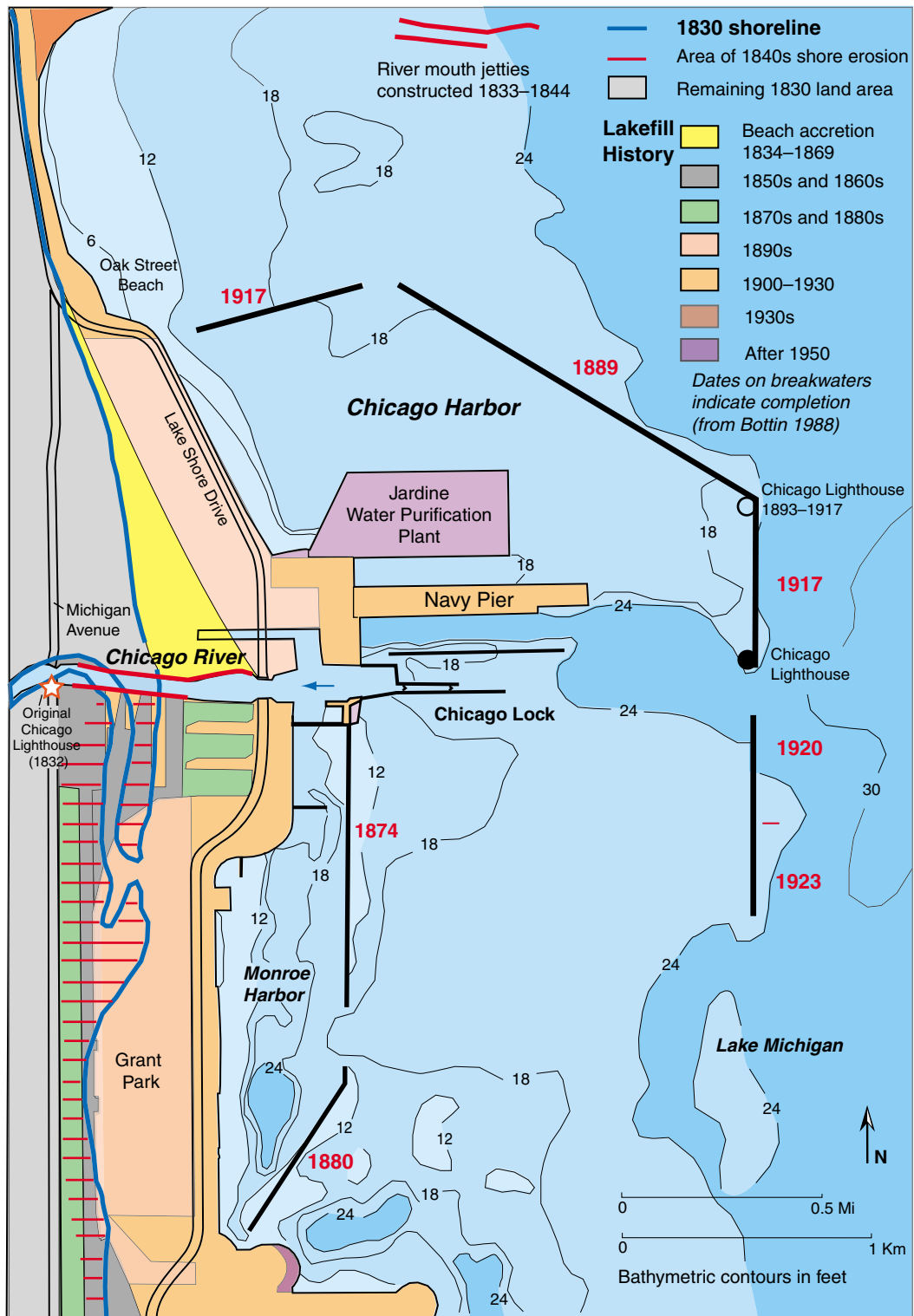
Historical shoreline change and bathymetry in the vicinity of Chicago Harbor (after Chrzastowski 1991, 1998).
