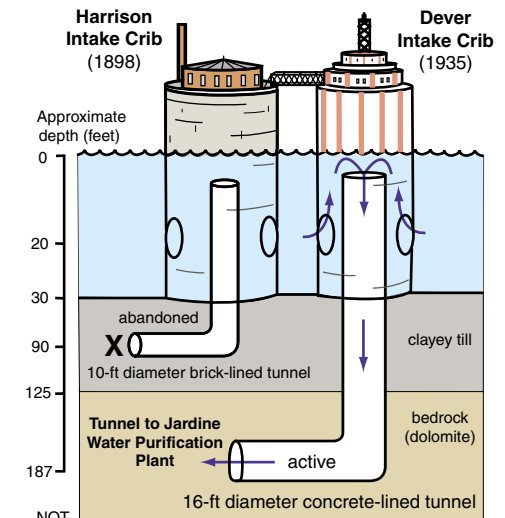
Intake crib schematic.
