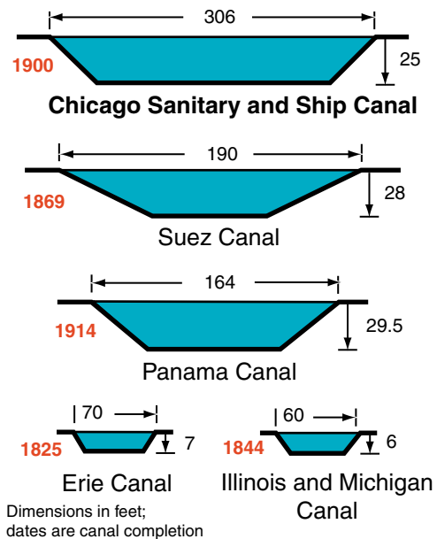
Schematic comparison of Chicago Sanitary and Ship Canal and other major canals (modified from chipublic.org).
