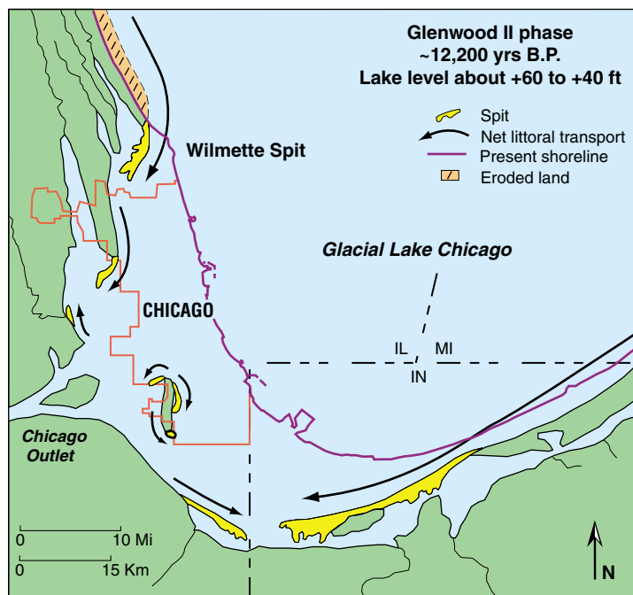
Paleogeography of the Chicago area during formation of Wilmette Spit (modified from Chrzastowski and Thompson 1992).
