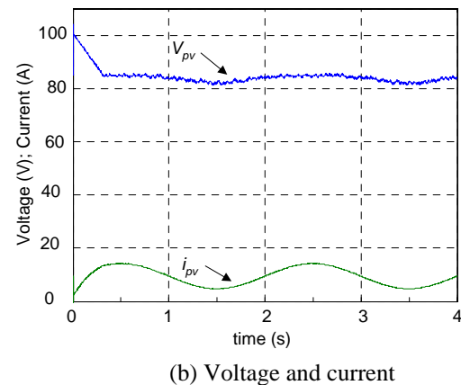
Fig. 8. The PV output of MP&O method under sinusoidal changing irradiance
