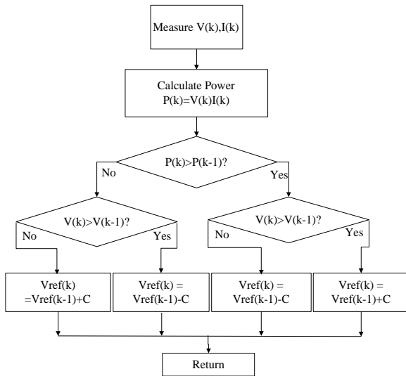
Fig. 2. P&O method flow chart
