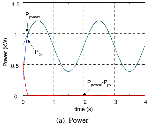
(a) Power (c) Voltage and current Fig. 9. The PV output of proposed EPP method under sinusoidal changing irradiance
