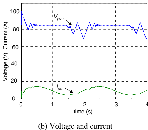
Fig. 7. The PV output of P&O method under sinusoidal changing irradiance
