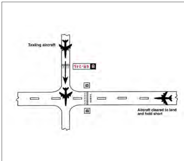
FIG 4-3-7 Land and Hold Short of an Intersecting Taxiway
