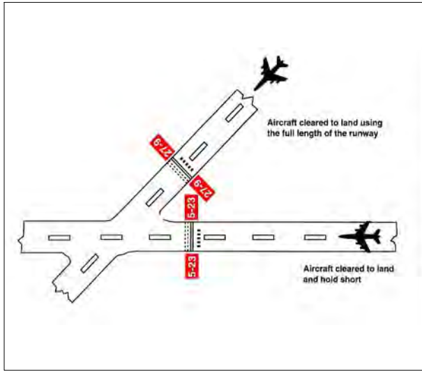
FIG 4-3-6 Land and Hold Short of an Intersecting Runway
