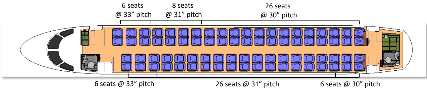
High Capacity – 78 seats – Single Class – 33"/31"/30" Elite Seat
