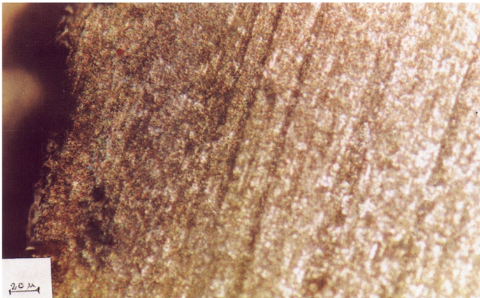
Fig. 6. Microstructure of the dagger piece showing mainly ferrite with a banded structure. The cutting edge shows mostly pearlite dark etching (500 X)
