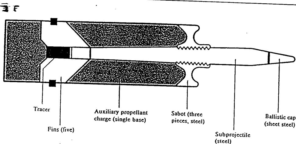
Figure 23 Cutaway View of a Soviet BM-9 125-mm Kinetic-Energy Tank Gun Round
