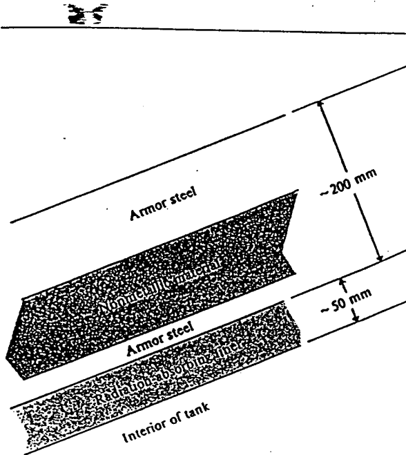
Figure 3 Configuration of Soviet T-72/T-64 Glacis Armor Array
