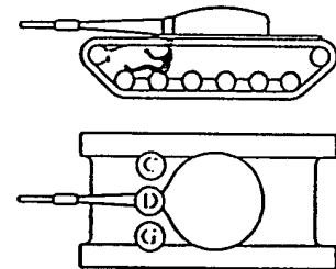
Reduced-volume-turret tank with crew forward in hull
