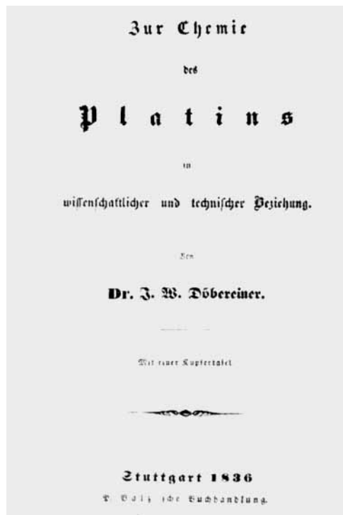
The title page of Döbereiner's book on the chemistry of platinum
