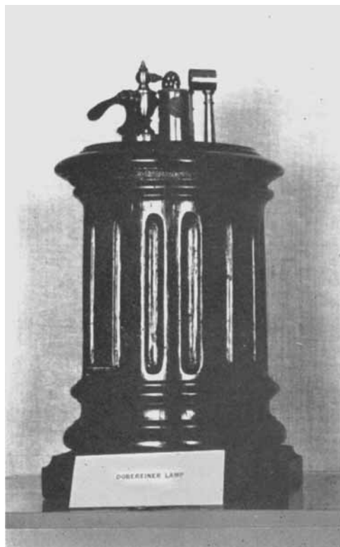
One of many types of Döbereiner lamp in which a jet of hydrogen, generated from zinc and dilute sulphuric acid, is ignited by a small amount of finely divided platinum. (By courtesy of the Science Museum)
