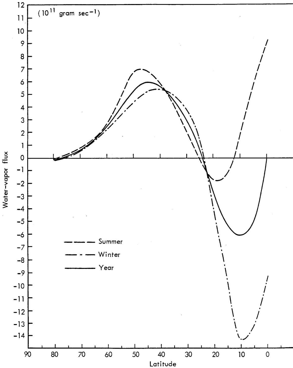
Fig. 4 — The meridional distribution of zonally averaged water-vapor flux in the atmosphere computed from atmospheric data. (After Starr, et al. , 1957.)
