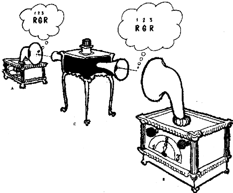
Figure 7 – Instruction sets.
