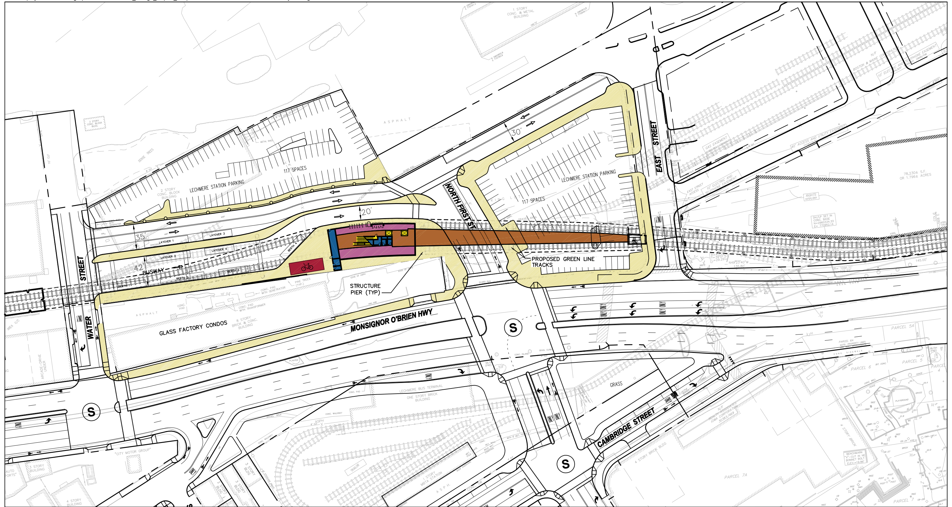
Figure 3.7-2 Relocated Lechmere Station Station Layout
