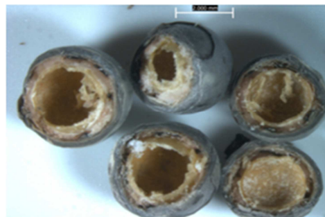
Figure 2 Capsules cut open shows void space to accommodate expansion of salt
